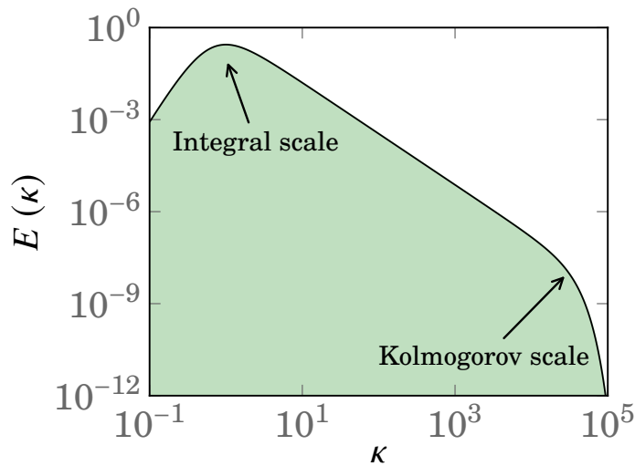
Figure 2.1.: Energy spectra
