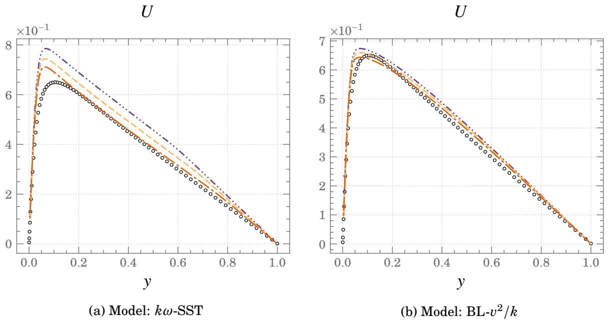
Figure 4.11.: Mean profiles of Velocity at Ra \approx 1.7 \times 10^7 ( Gr = 3 \times 10^6 ) \circ \circ \circ DNS --- FBE --- GGDH - \cdot - \cdot SGDH
