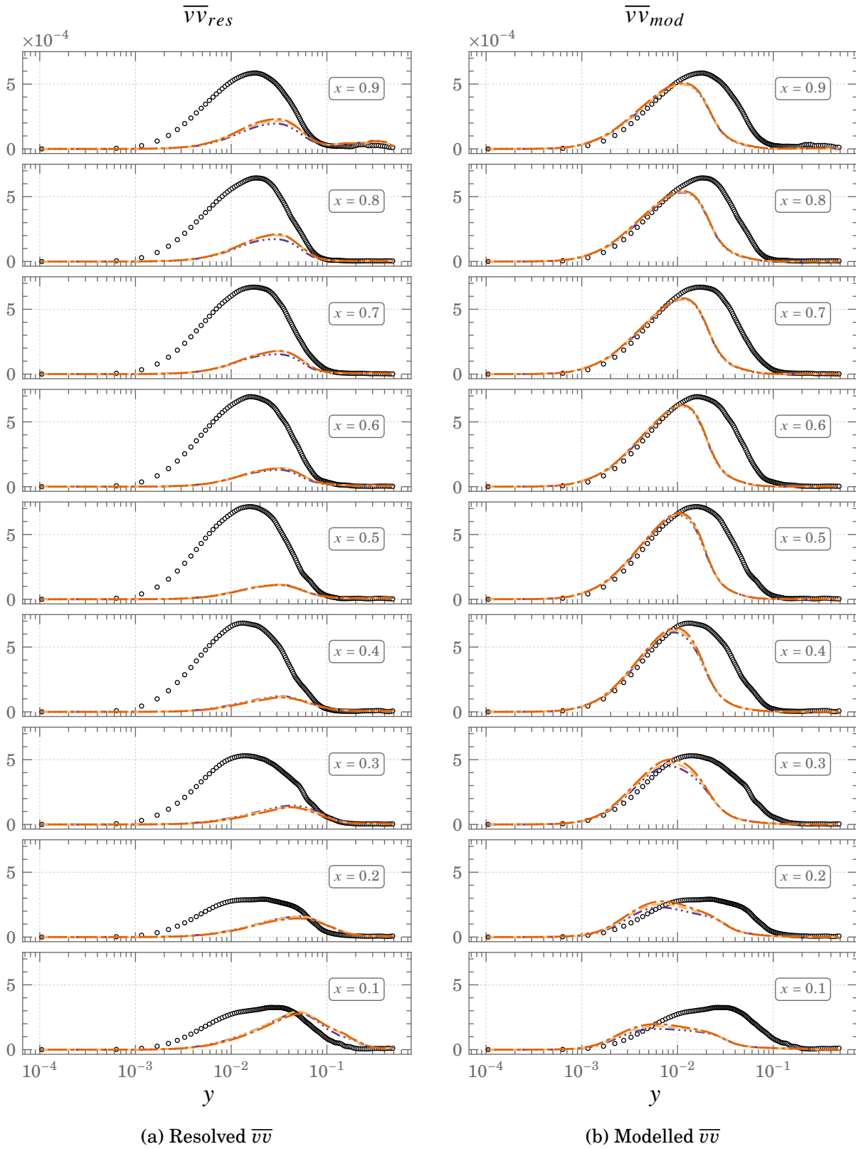
Figure 5.22.: Resolved and modelled contributions of \overline{v'v'} using the HTLES model for Square DHC at Ra = 10^{11}
