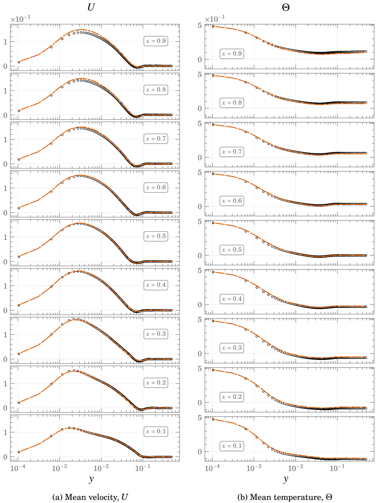
Figure A.13.: Comparisons of mean velocity and temperature profiles for Square DHC at Ra = 10^{11}
