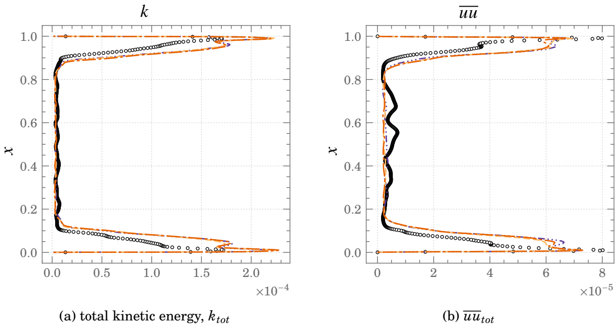
Figure A.10.: Comparisons of total kinetic energy and \overline{uu}_{tot} profiles at the mid cavity ( y = 0.5 ) for Square DHC at Ra = 10^{11} \circ \circ \circ DNS -\cdot-\cdot- 498 \times 80 -\cdot-\cdot- 664 \times 80 -\cdot-\cdot- 996 \times 100
