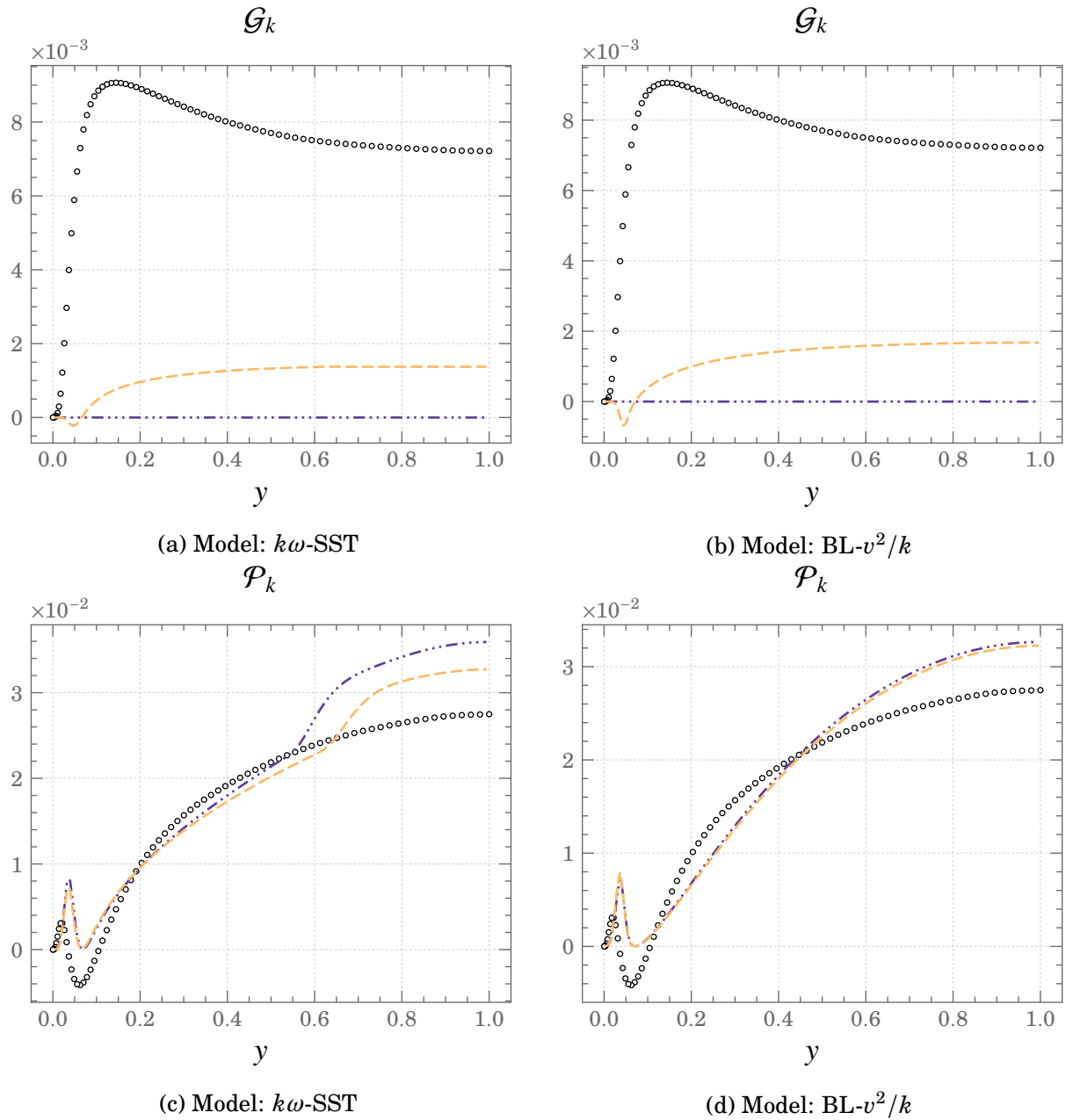
Figure 4.1.: Kinetic energy production, \mathcal{G}_k and \mathcal{P}_k at Ra \approx 1.7 \times 10^7 ( Gr = 3 \times 10^6 ) \circ \circ \circ DNS --- GGDH - \cdot - \cdot - SGDH
