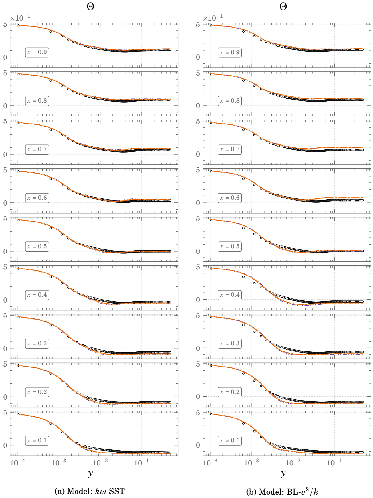
Figure 4.22.: Mean profiles of Temperature at Ra \times 10^{11}
