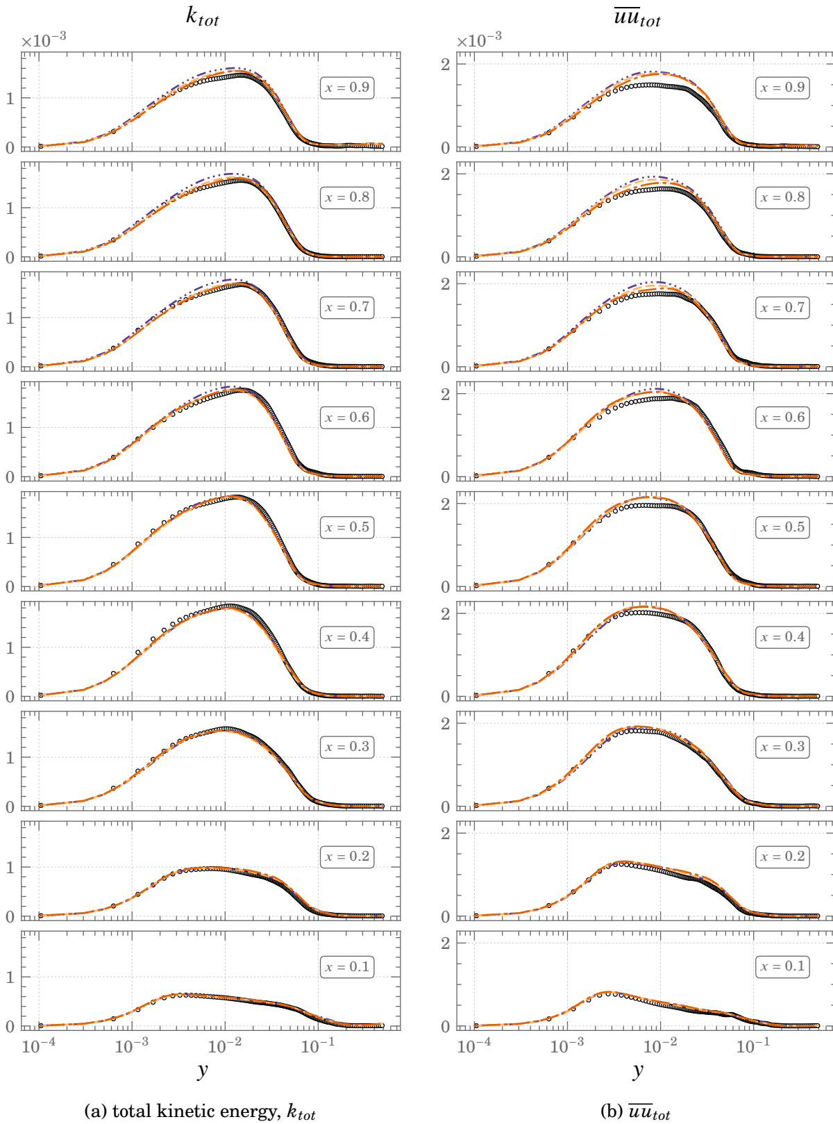
Figure A.2.: Comparisons of k_{tot} and \overline{u'u}_{tot} profiles for Square DHC at Ra = 10^{11} \circ \circ \circ DNS - - - 498 \times 80 - - - 664 \times 80 \cdots \cdots 996 \times 100
