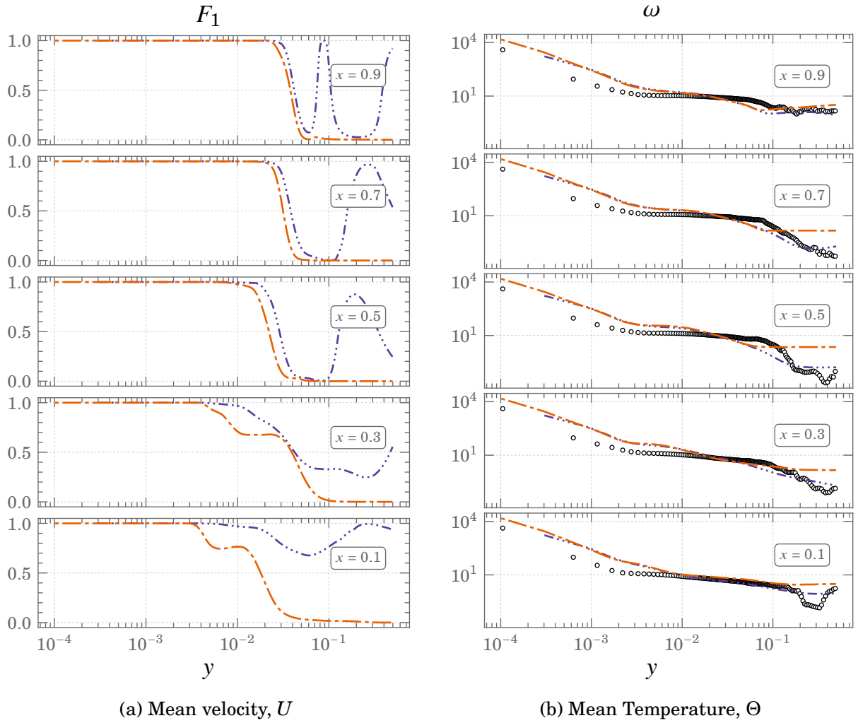
Figure 4.39.: Profiles of the blending function, F_1 and Specific dissipation rate, \omega for SGDH heat flux closure at Ra \times 10^{11} \circ \circ \circ DNS -\cdot-\cdot- G_\omega^{SST} \cdots G_\omega^{k\omega}
