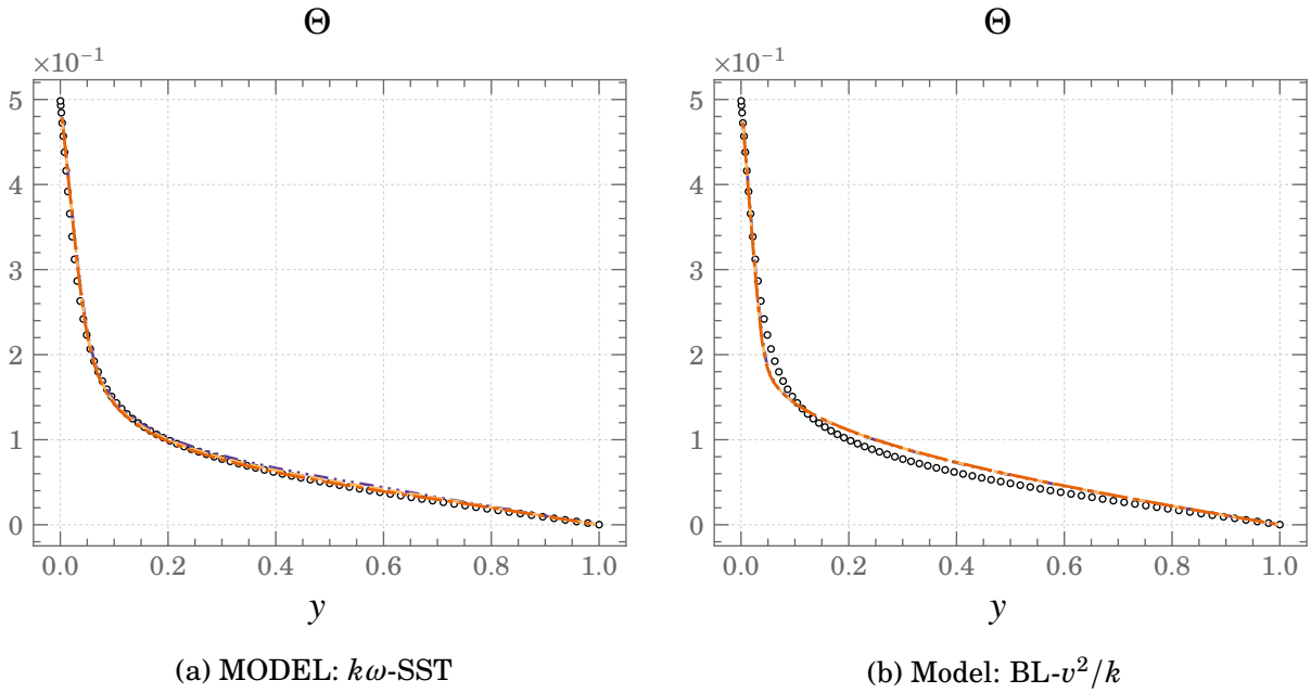
Figure 4.15.: Mean profiles of Temperature at Ra \approx 1.7 \times 10^7 ( Gr = 3 \times 10^6 ) \circ \circ \circ DNS --- FBE --- GGDH \cdots SGDH
