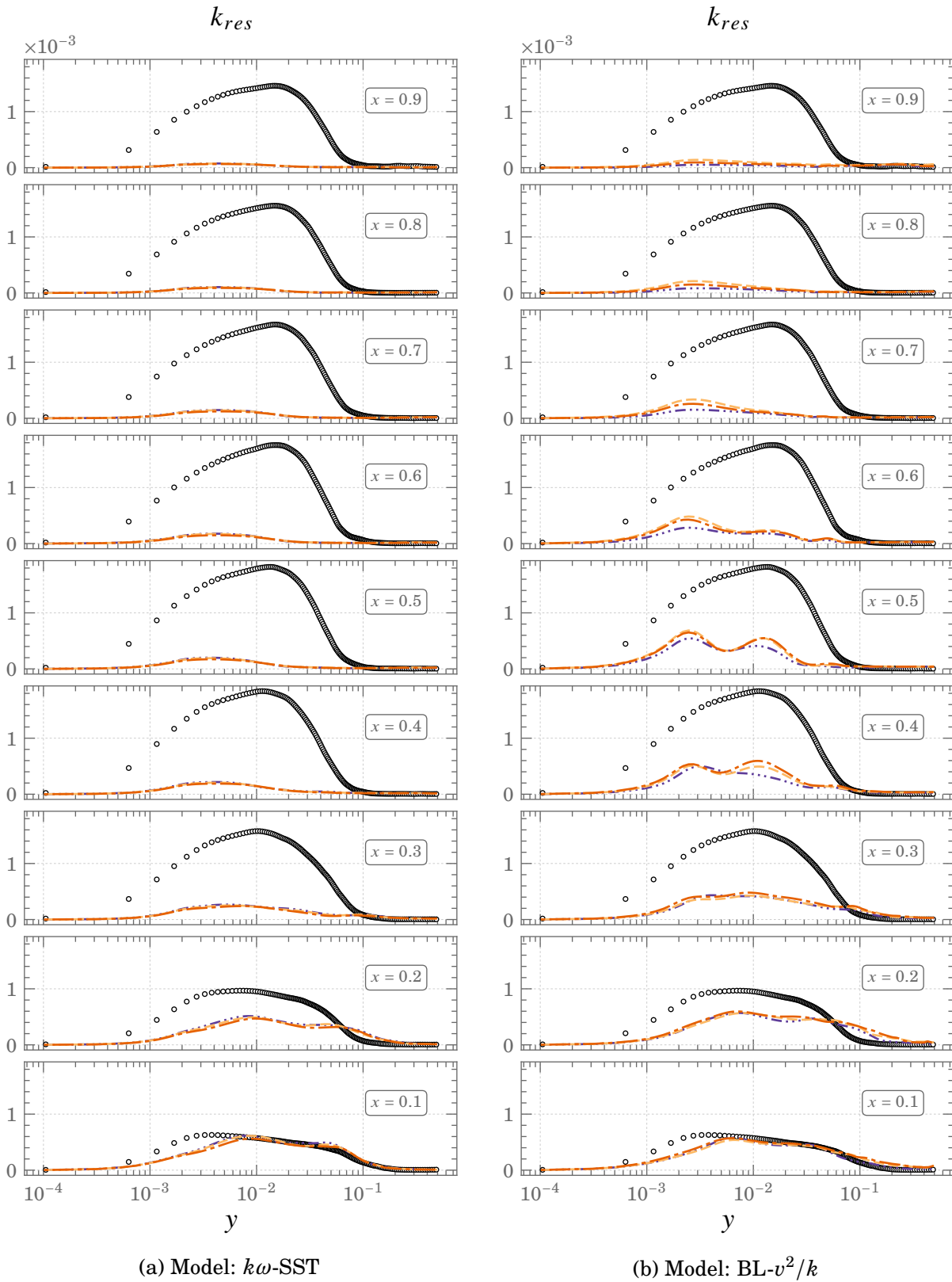
Figure 4.33.: Mean profiles of resolved turbulent kinetic energy, k_{res} , at Ra \times 10^{11} \circ \circ \circ DNS --- FBE --- GGDH - \cdot - \cdot - SGDH
