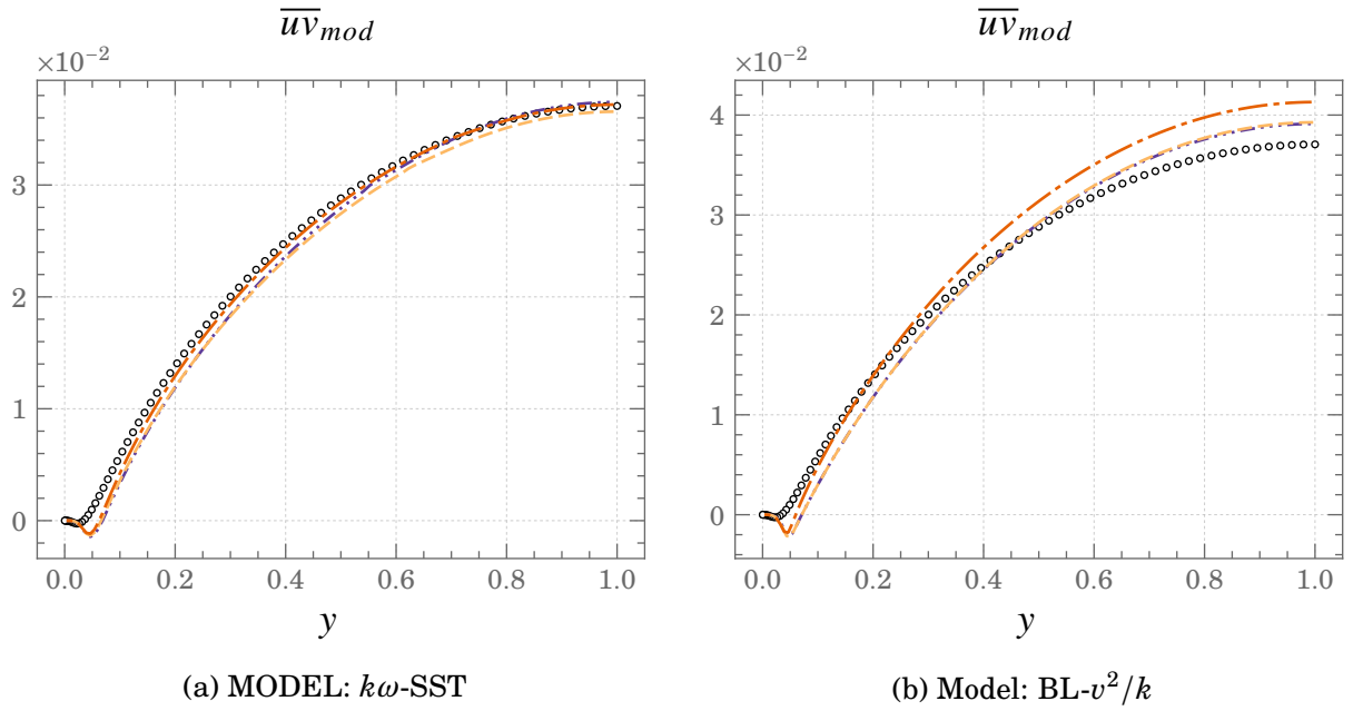
Figure 4.10.: Mean profiles of the turbulent shear stress, \overline{uv} \circ \circ \circ DNS --- FBE --- GGDH - \cdot - \cdot SGDH
