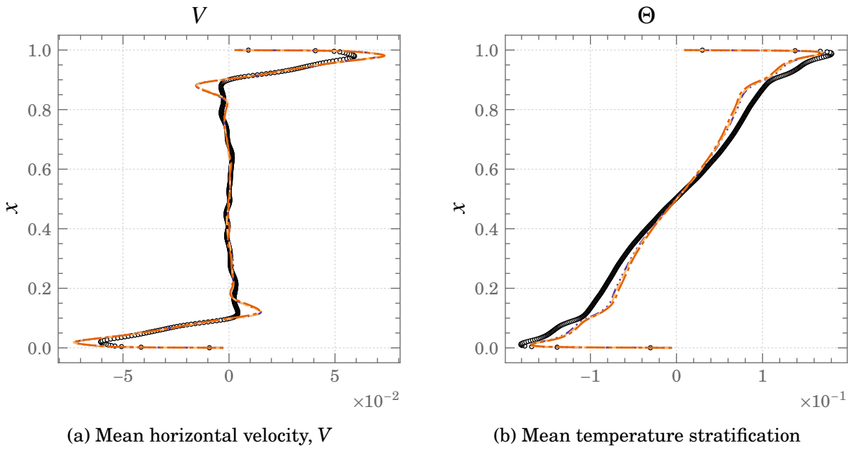
Figure A.9.: Comparisons of mean horizontal velocity and temperature stratification profiles at the mid cavity ( y = 0.5 ) for Square DHC at Ra = 10^{11} \circ \circ \circ DNS -\cdot-\cdot- 498 \times 80 -\cdot-\cdot- 664 \times 80 -\cdot-\cdot- 996 \times 100
