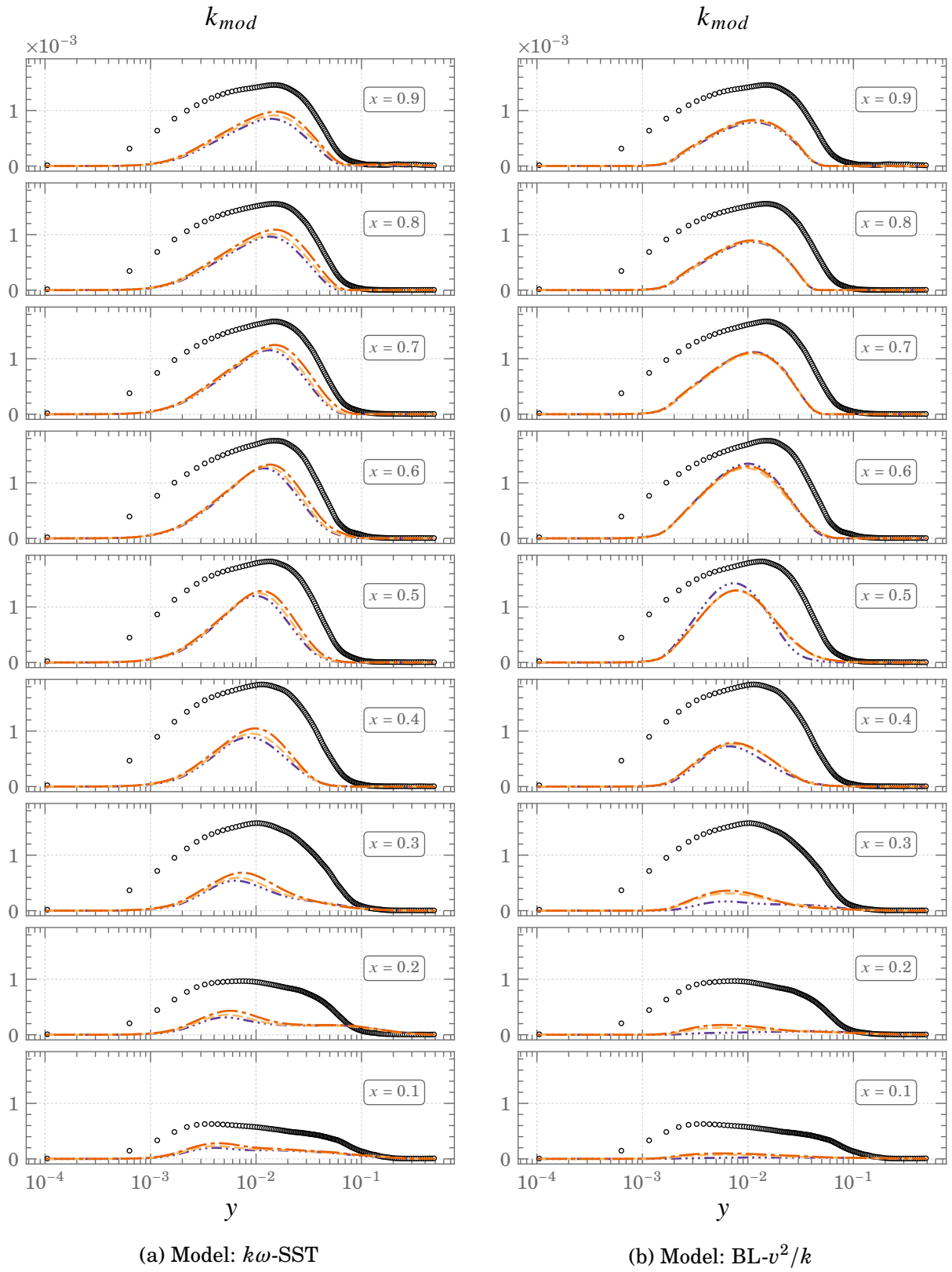
Figure 4.32.: Mean profiles of modelled turbulent kinetic energy, k_{mod} , at Ra \times 10^{11} \circ \circ \circ DNS --- FBE --- GGDH \cdots SGDH
