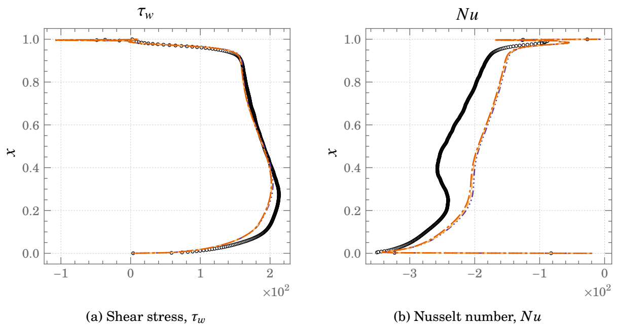
Figure 5.29.: Profiles of Wall shear stress and Nusselt number at the hot wall using the HTLES model for Square DHC at Ra \times 10^{11}
