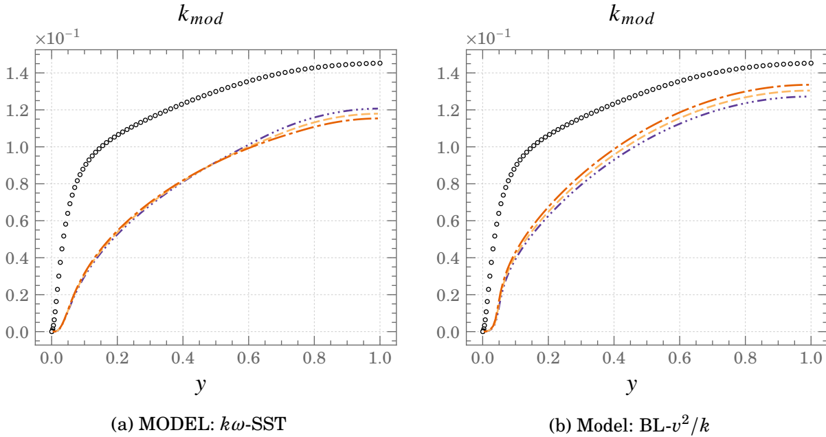
Figure 4.12.: Mean profiles of the turbulent kinetic energy, k
