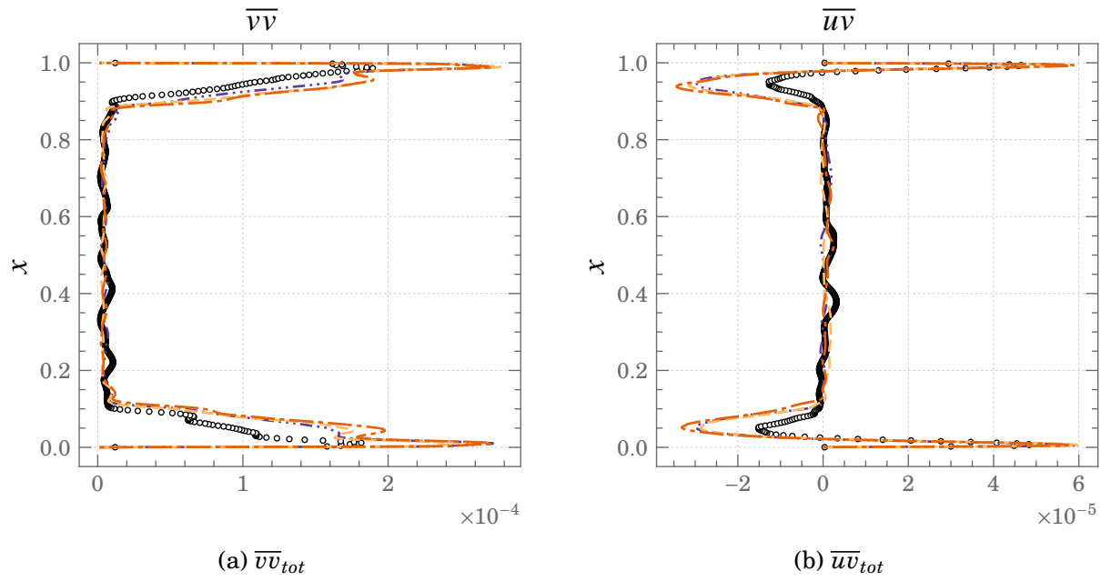
Figure A.23.: Comparisons of \overline{v v}_{tot} and \overline{u v}_{tot} profiles at the mid cavity ( y = 0.5 ) for Square DHC at Ra = 10^{11}
