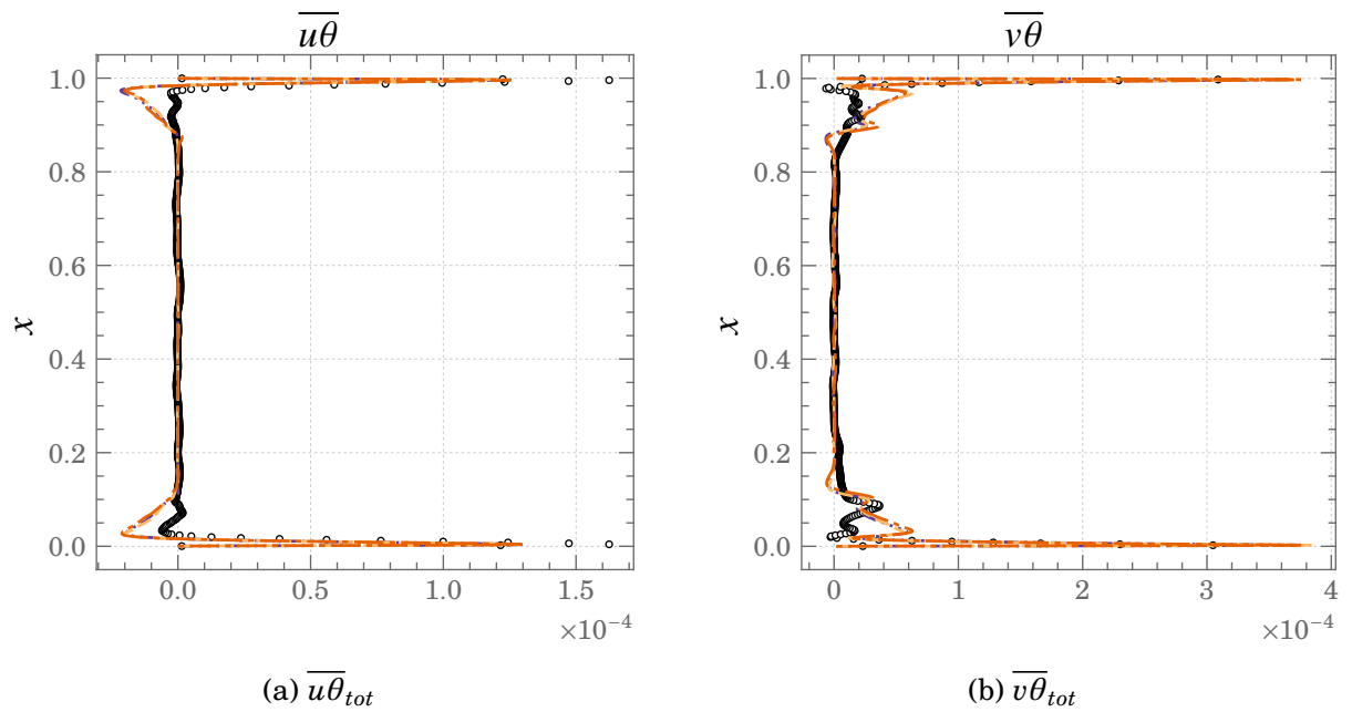
Figure A.24.: Comparisons of \overline{u \theta}_{tot} and \overline{v \theta}_{tot} profiles at the mid cavity ( y = 0.5 ) for Square DHC at Ra = 10^{11}
