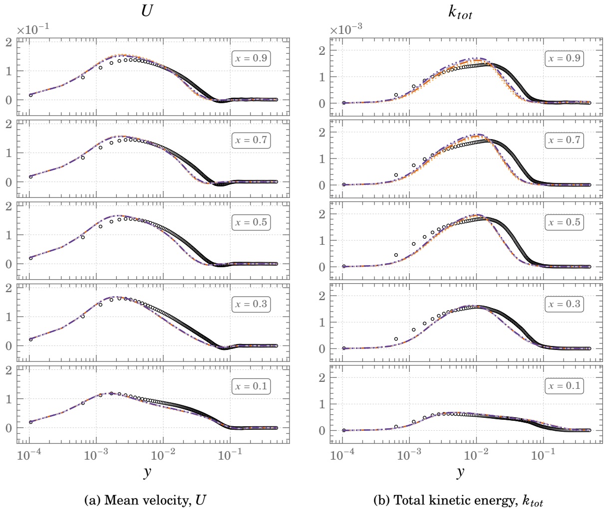
Figure 5.1.: Mean profiles of Velocity and total kinetic energy for various meshes at Ra \times 10^{11} \circ \circ \circ DNS \cdots 249^2 -\cdots- 332^2 -\cdots- 415^2 -\cdots- 498^2
