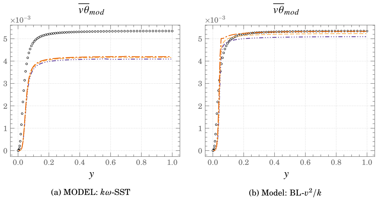
Figure 4.17.: Mean profiles of the Wall normal heat flux, \overline{v\theta} \circ \circ \circ DNS --- FBE --- GGDH - \cdot - \cdot - SGDH
