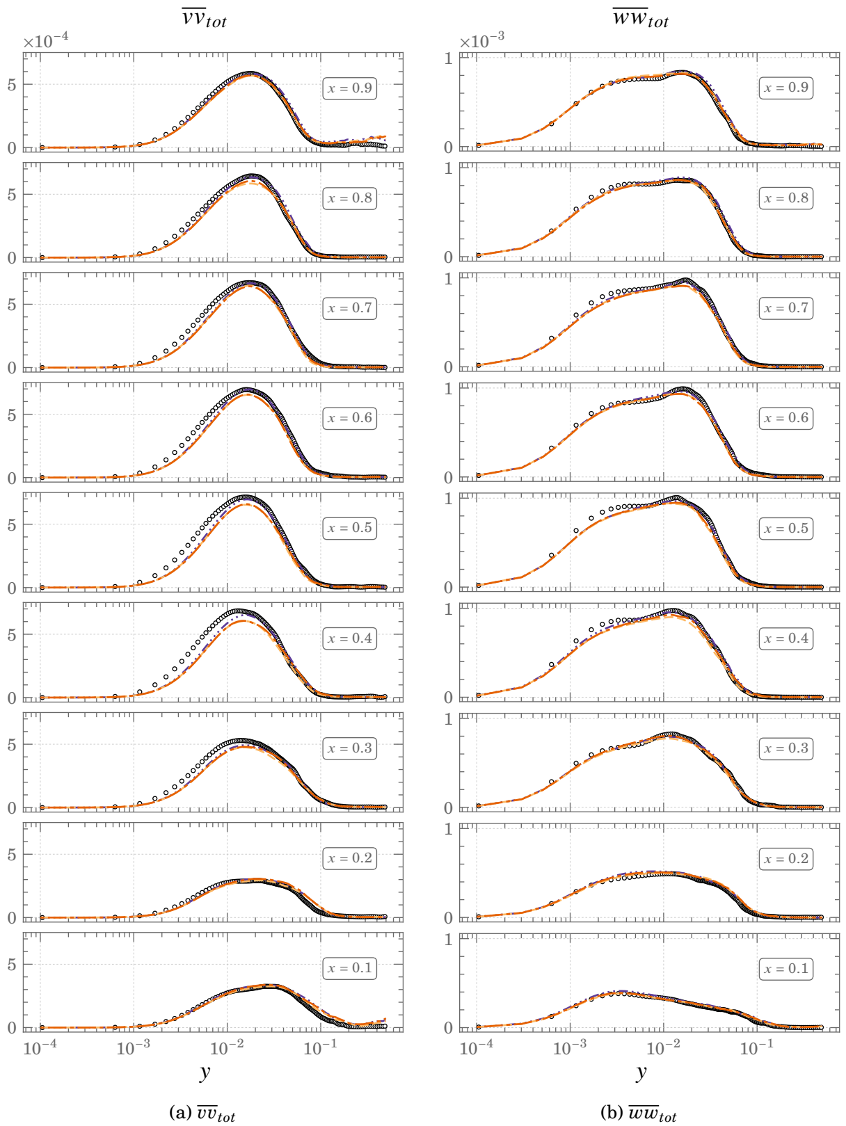
Figure A.15.: Comparisons of \overline{v v}_{tot} and \overline{w w}_{tot} profiles for Square DHC at Ra = 10^{11} \circ \circ \circ DNS -\cdot-\cdot- Dyn-SMAG -\cdot-\cdot- SMAG \cdots\cdots WALE
