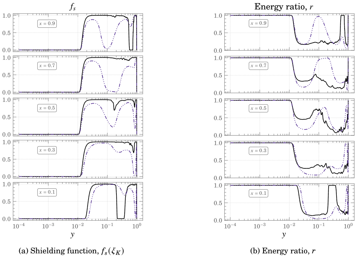
Figure 5.7.: Behaviour of the shielding function and its impact on the energy ratio in HTLES - - - f_s(\xi_K) — DNS
