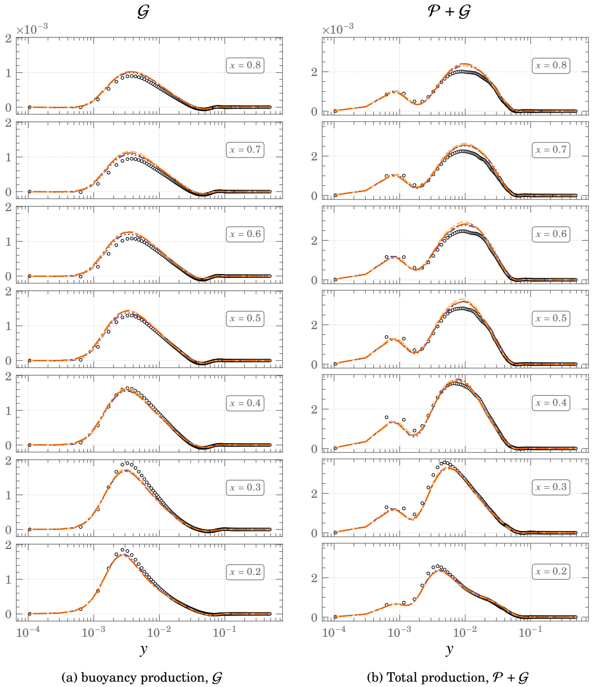
Figure A.17.: Comparisons of buoyancy production, \mathcal{G} , and total production, \mathcal{P} + \mathcal{G} , profiles for Square DHC at Ra = 10^{11} \circ \circ \circ DNS --- Dyn-SMAG --- SMAG \cdots WALE
