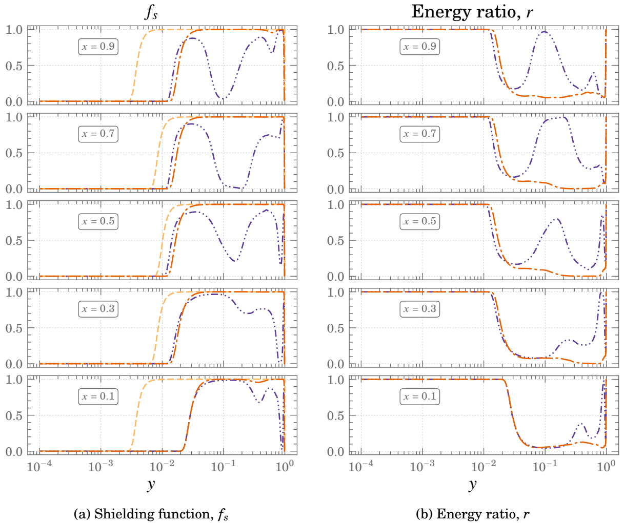
Figure 5.12.: Behaviour of the shielding functions and the resulting energy ratio imposed by the model in a Square DHC at Ra = 10^{11} \text{---} f_s(\xi_D) \text{-}\cdot\text{-}\cdot\text{-}\cdot f_s(\xi_K) \text{-}\cdot\text{-}\cdot\text{-}\cdot f_s(\xi_\alpha)
