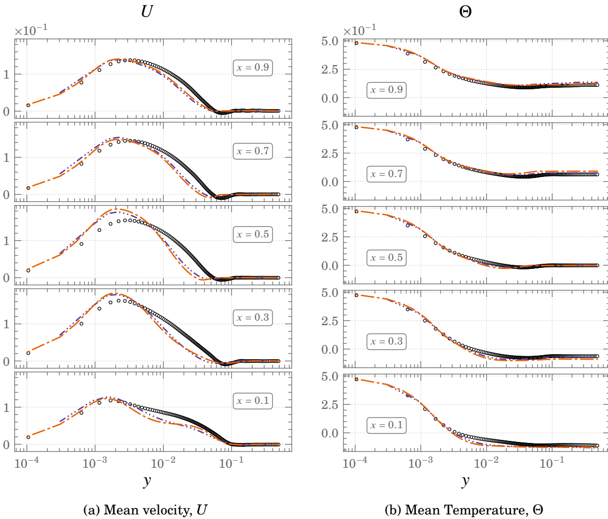
Figure 4.36.: Mean profiles of Velocity and Temperature for SGDH heat flux closure at Ra \times 10^{11} \circ \circ \circ DNS --- G_{\omega}^{SST} \cdots G_{\omega}^{k\omega}
