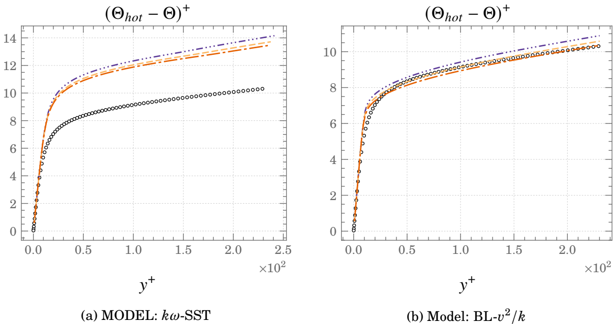
Figure 4.16.: Mean profiles of Temperature normalised with inner wall units at Ra \approx 1.7 \times 10^7 ( Gr = 3 \times 10^6 ) \circ \circ \circ DNS --- FBE --- GGDH \cdots SGDH
