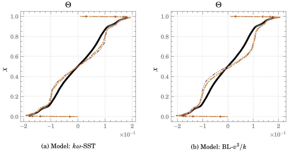
Figure 4.20.: Profiles of Temperature stratification at y = 0.5 for Ra \times 10^{11} \circ \circ \circ DNS --- FBE \cdots GGDH \cdots SGDH
