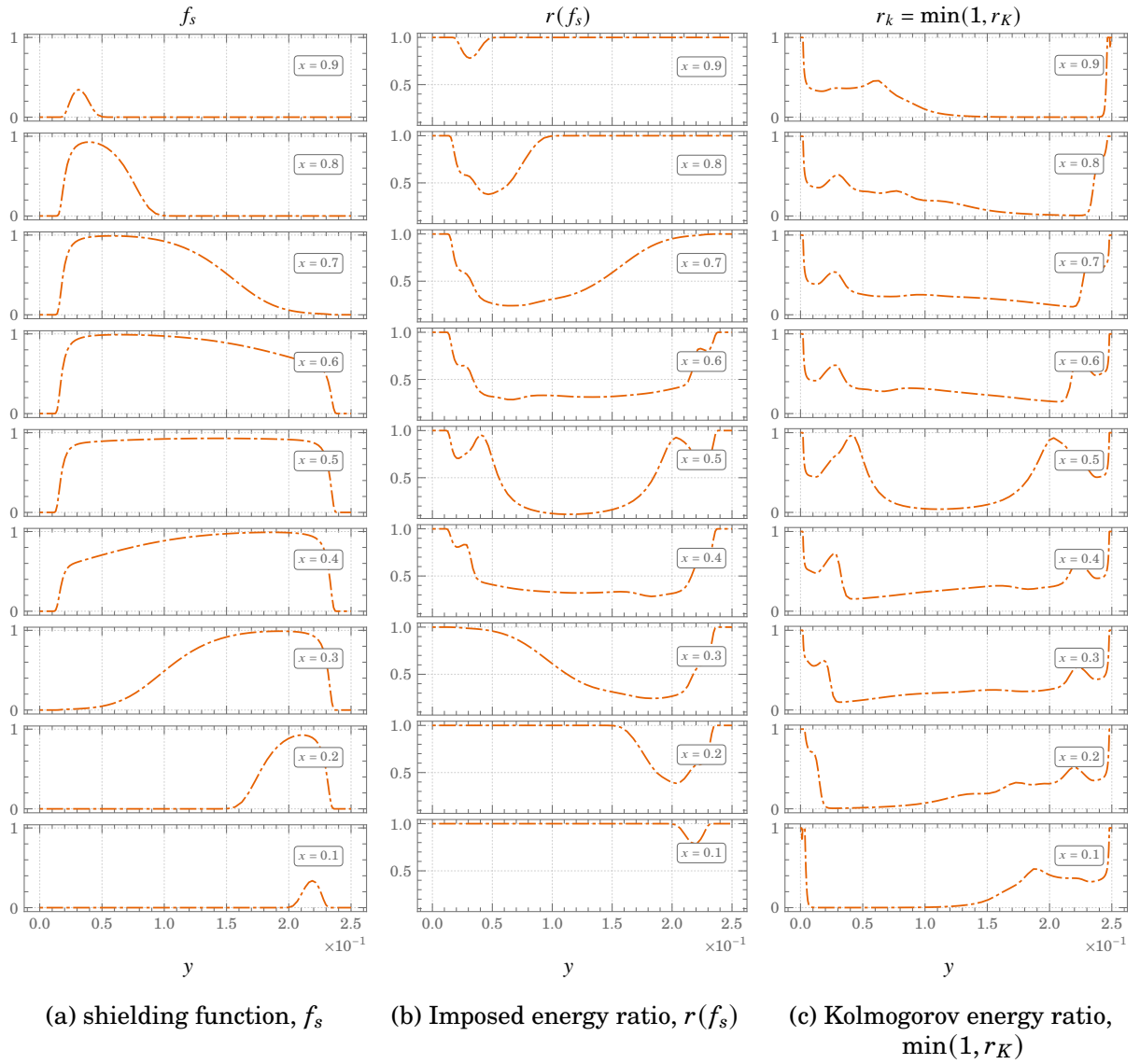
Figure B.4.: profiles of f_s , r(f_s) , and \min(1, r_K) for Rectangular DHC at Ra = 10^{11} - - - HTLES
