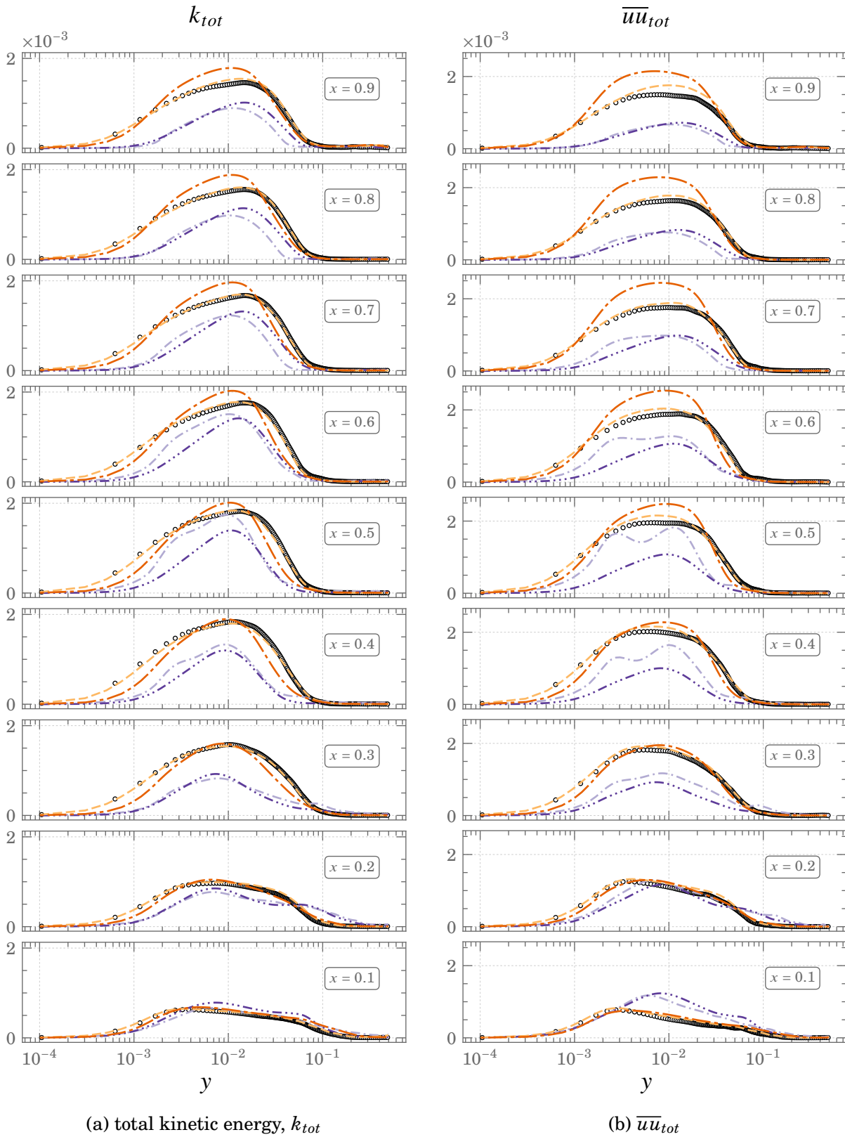
Figure 5.31.: Comparisons of k_{tot} and \overline{u'u}_{tot} profiles for Square DHC at Ra = 10^{11} ○ ○ ○ DNS - - - HTLES - - - LES - - - RANS – BL ····· RANS – KW
