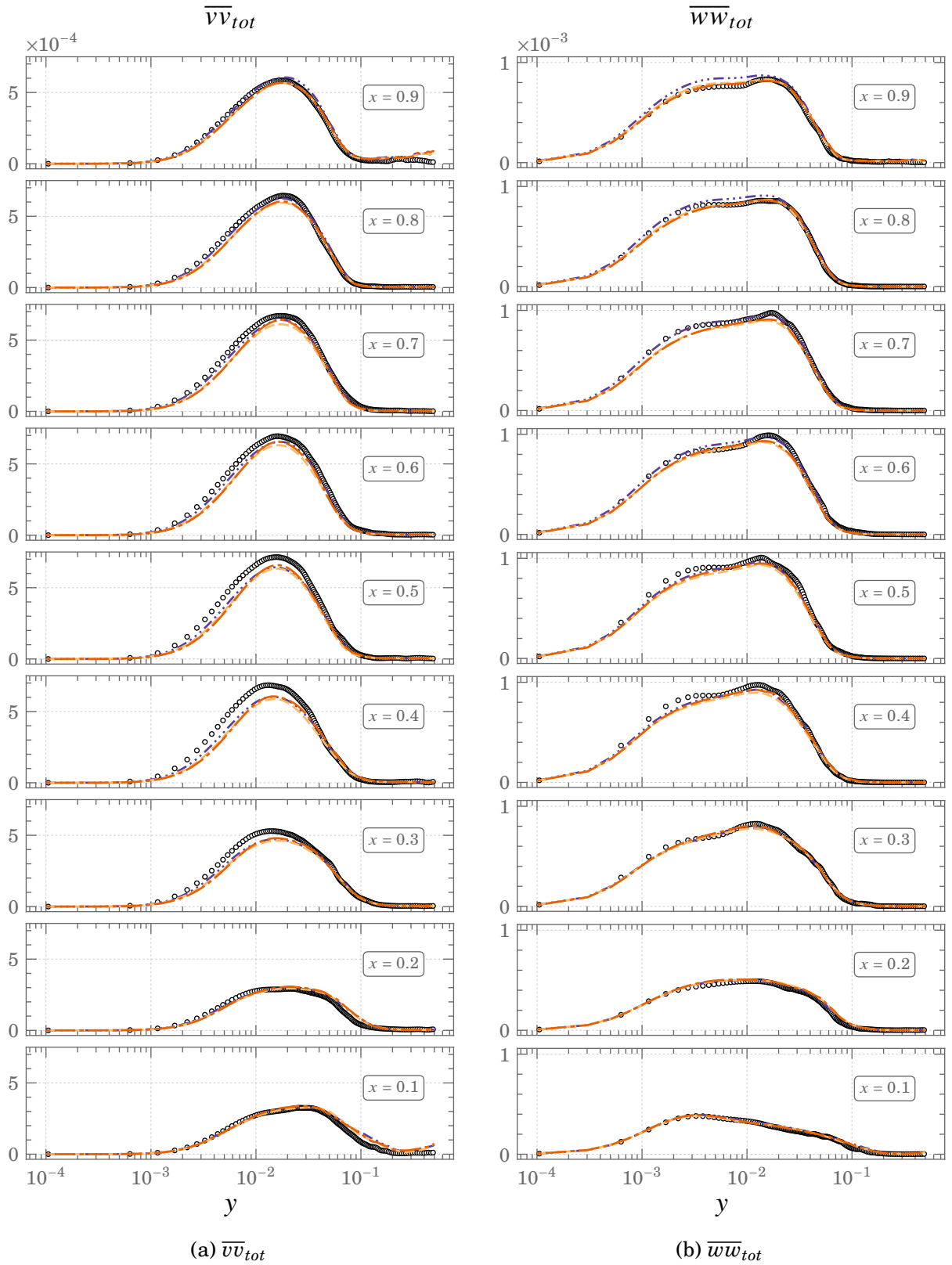
Figure A.3.: Comparisons of \overline{v v}_{tot} and \overline{w w}_{tot} profiles for Square DHC at Ra = 10^{11} \circ \circ \circ DNS --- 498 \times 80 --- 664 \times 80 \cdots 996 \times 100
