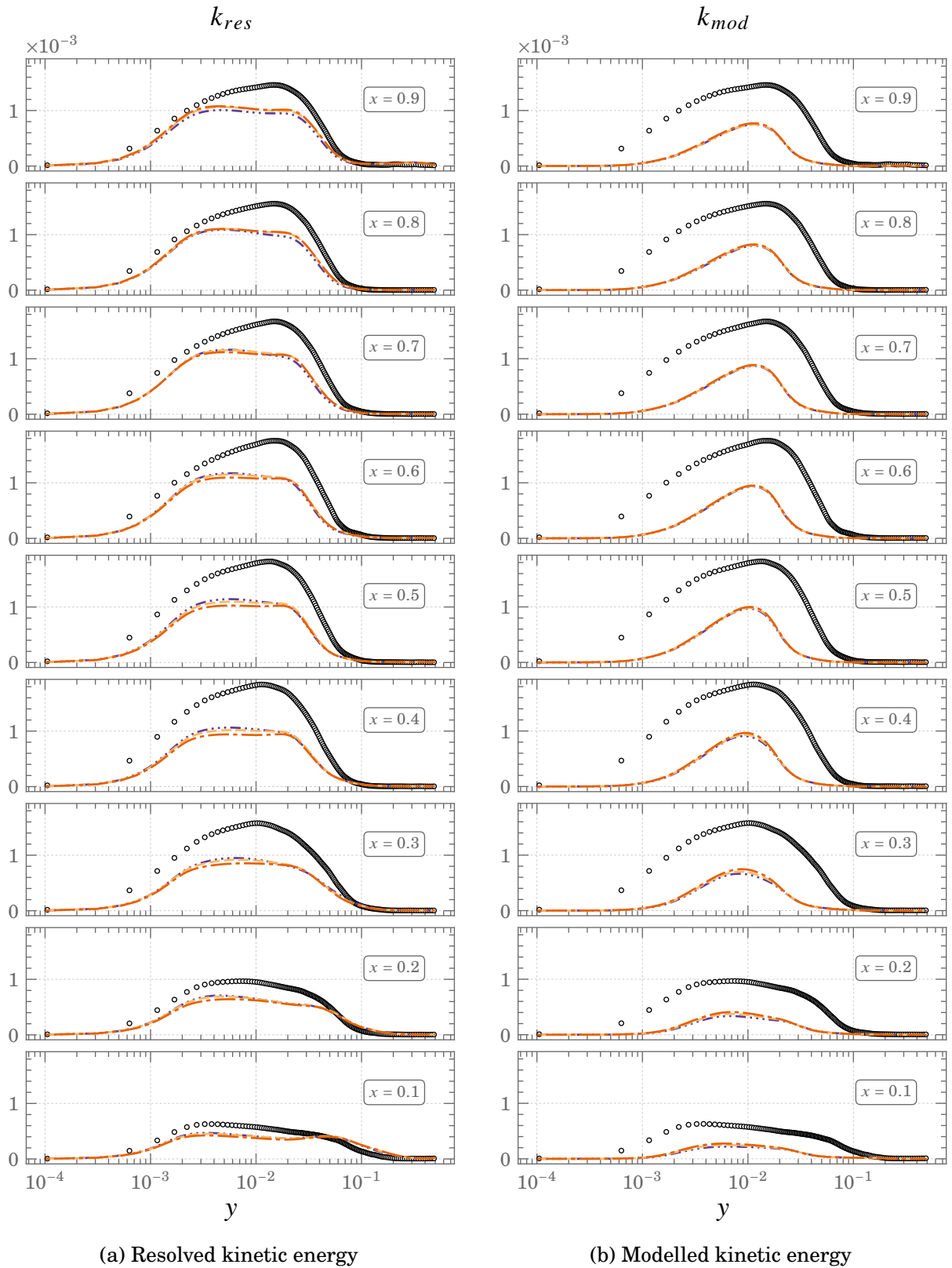
Figure 5.19.: Resolved and modelled contributions of total kinetic energy using the HTLES model for Square DHC at Ra = 10^{11} \circ \circ \circ DNS --- FBE --- GGDH --- SGDH
