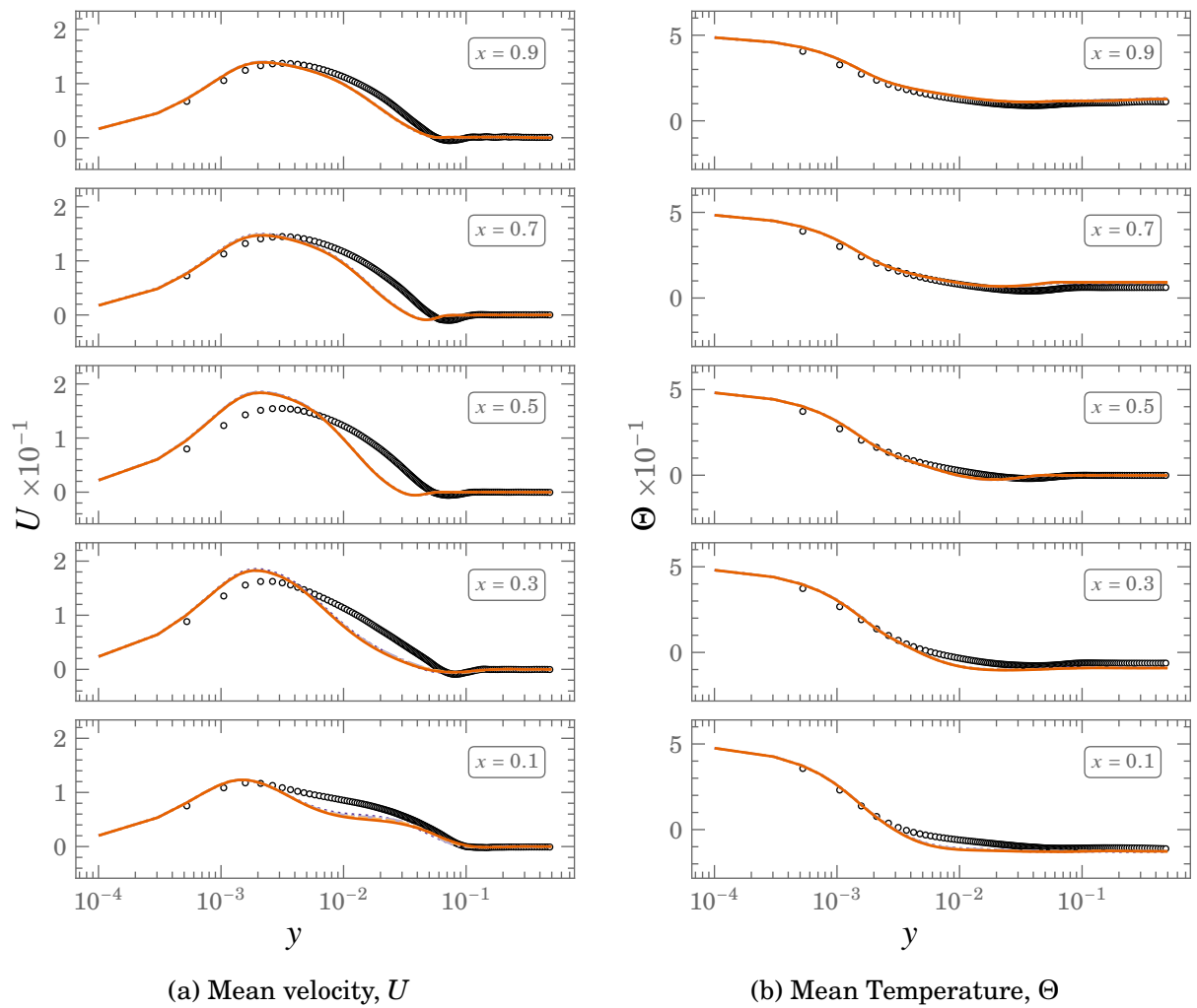
Figure 4.18.: Mean profiles of Velocity and Temperature for various meshes at Ra \times 10^{11} \circ \circ \circ \circ DNS \cdots 249^2 -\cdot- 332^2 --- 415^2 --- 498^2
