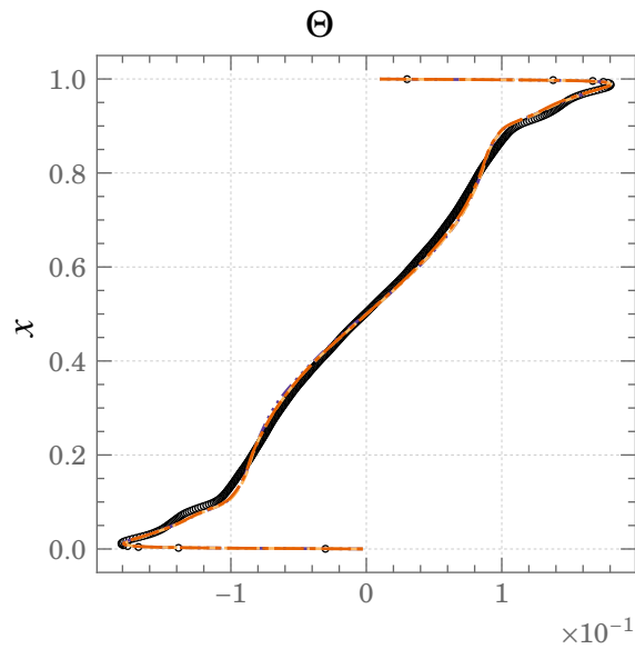
Figure 5.17.: Stratification observed using the HTLES model for Square DHC at Ra \times 10^{11} ○ ○ ○ DNS - - - FBE - - - GGDH ····· SGDH
