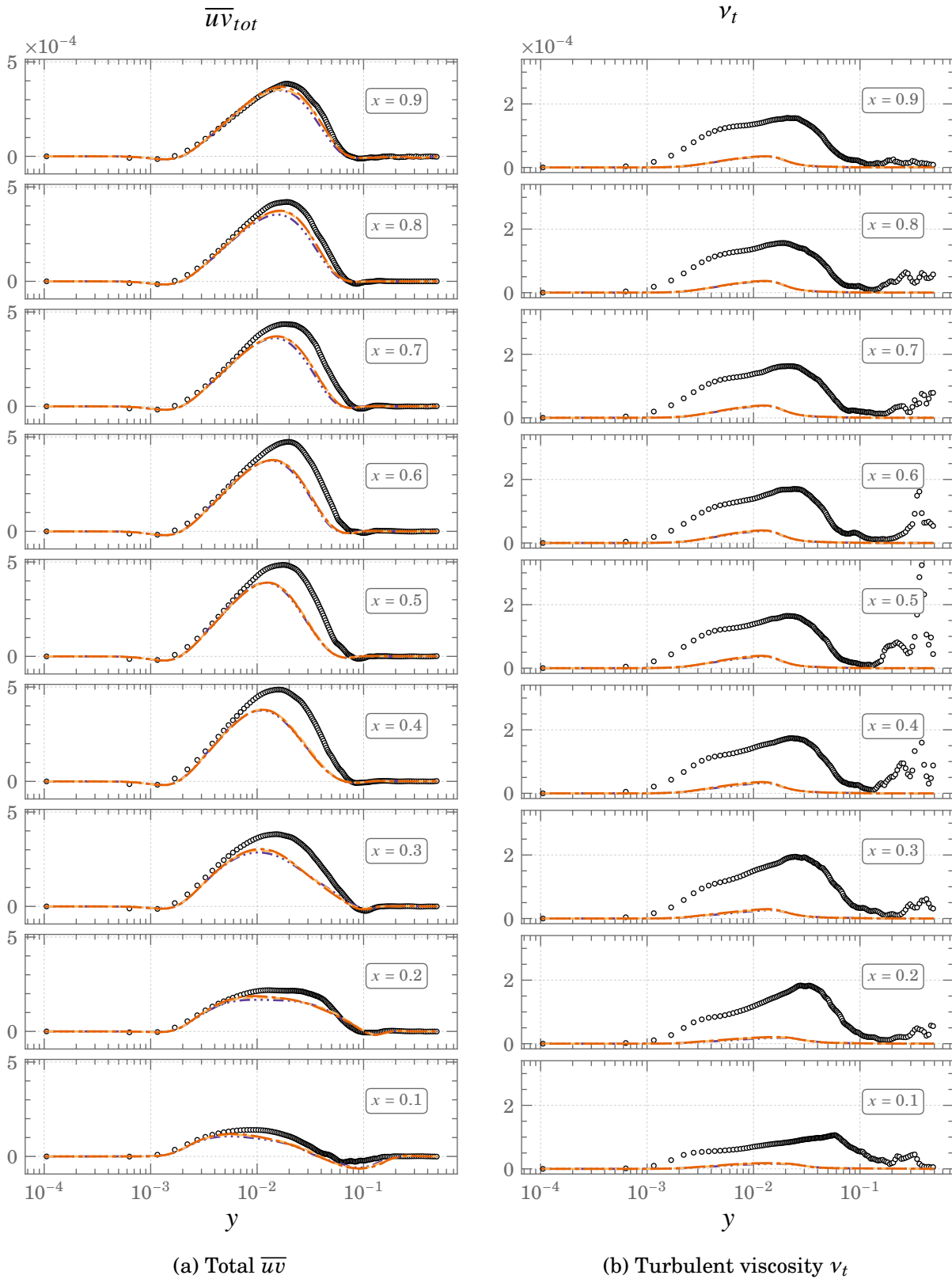
Figure 5.24.: Predictions of total shear stress, \overline{uv} and turbulent viscosity, \nu_t using the HTLES model for Square DHC at Ra = 10^{11}
