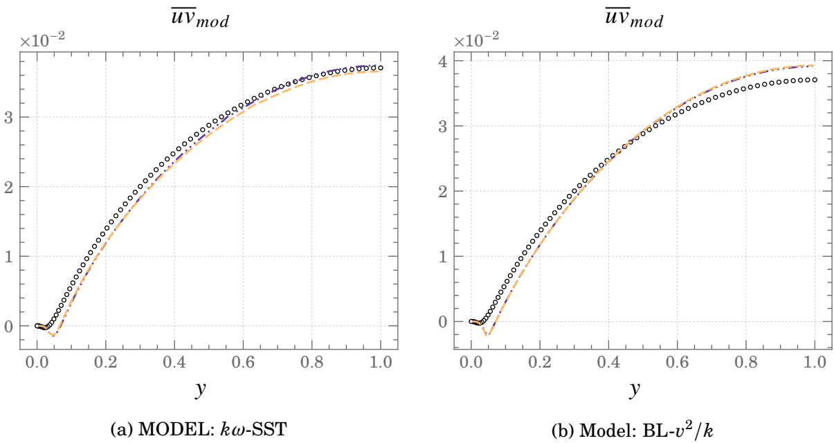
Figure 4.5.: Mean profiles of the turbulent shear stress, \overline{uv} \circ \circ \circ DNS --- GGDH \cdots SGD
