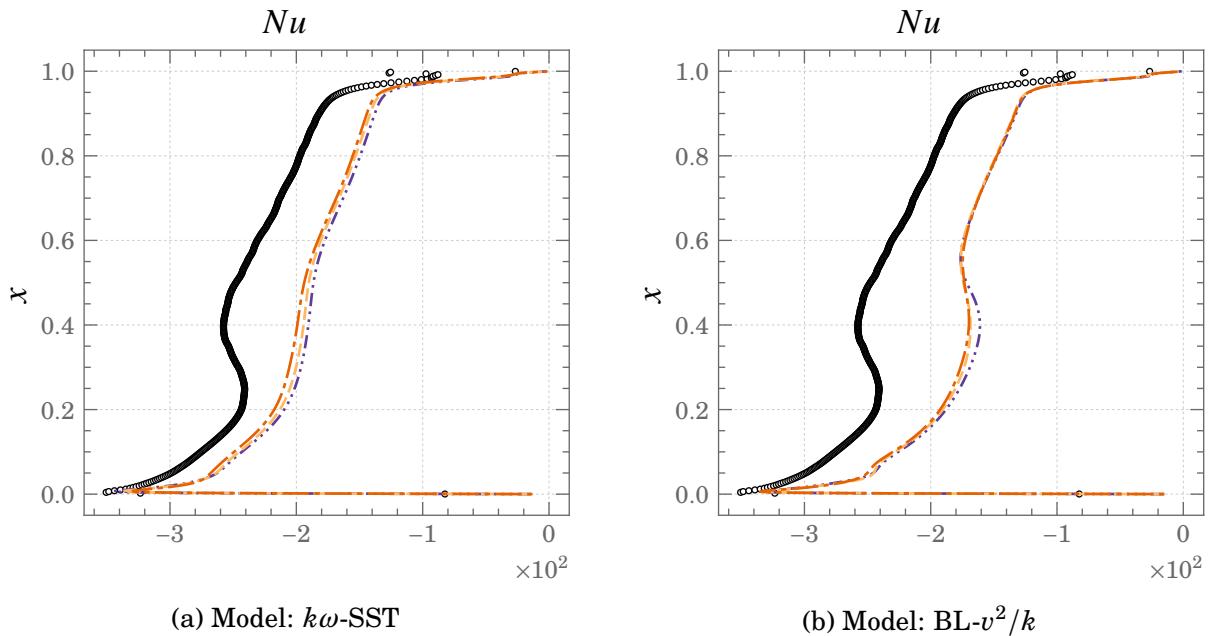
Figure 4.35.: Profiles of Nusselt number at the hot wall for Ra \times 10^{11} \circ \circ \circ DNS --- FBE - \cdot - GGDH - \cdot \cdot - SGDH
