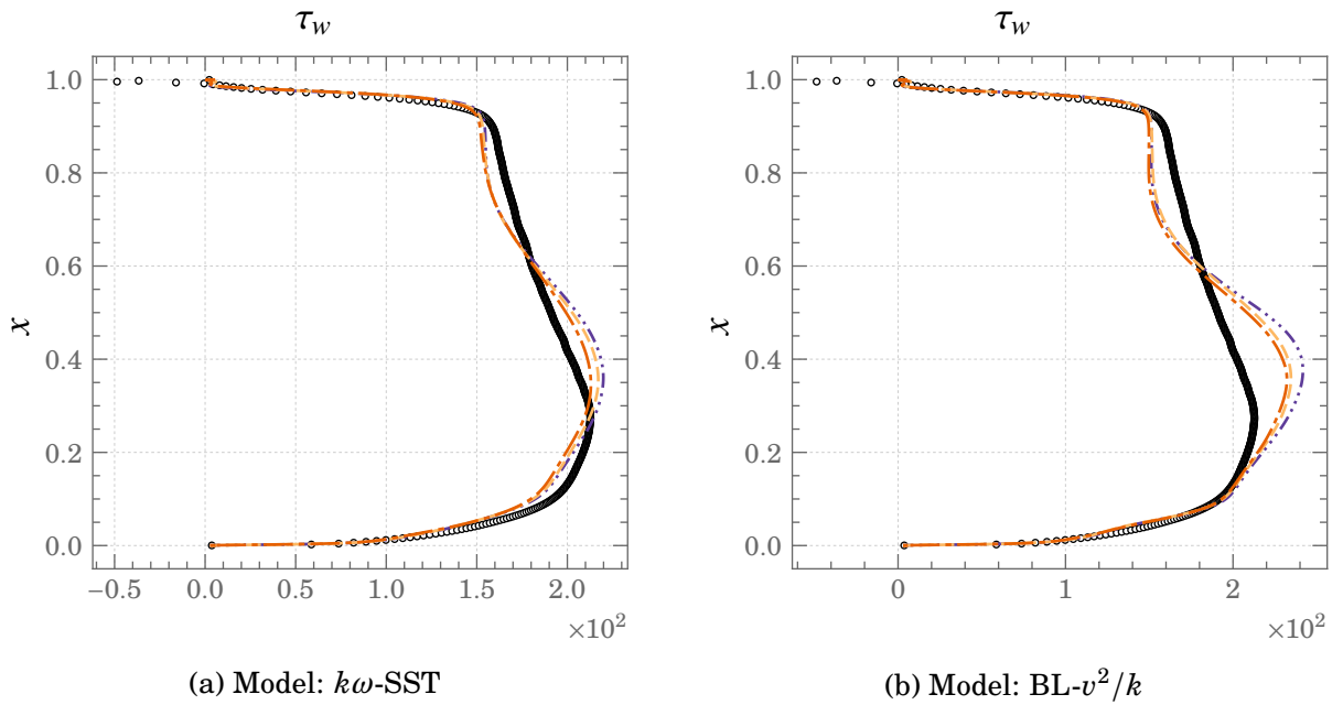
Figure 4.34.: Profiles of Wall shear stress, \tau_w , at the hot wall for Ra \times 10^{11} \circ \circ \circ DNS --- FBE - \cdot - GGDH - \cdot \cdot - SGDH
