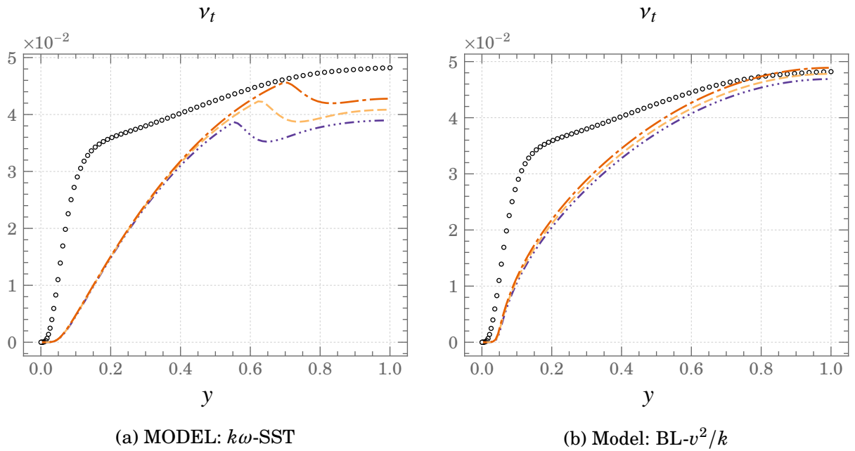
Figure 4.13.: Mean profiles of the turbulent viscosity, v_t \circ \circ \circ DNS - - - FBE - - - GGDH - \cdot - \cdot - SGDH
