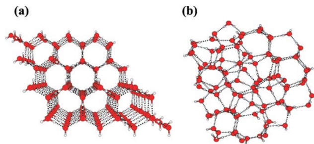
Figure 1.22: Molecular arrangement of (a) Ice Ih, (b) Low Density Amorphous ice (LDA). Almost all molecules join in the network of hydrogen bonds (black dashes). Figure from Belosludov et al. (2008)
