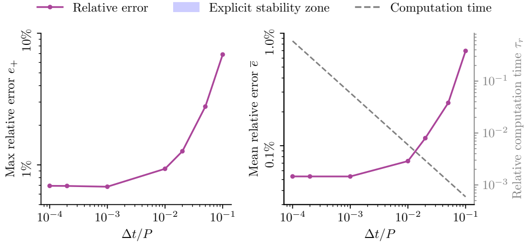
Figure 2.5: Relative errors produced by the fully implicit scheme when increasing the timestep \Delta t (log-scales). The reference is Spencer’s explicit thermal model computed with 10^4 points per day. Timestep \Delta t is represented as a fraction of the surface flux’ period P . The stability zone of the explicit scheme F < 1/2 is represented in light blue. ( Left ) Maximum error e_+ . ( Right ) Average error \bar{e} and relative computation time \tau_r . The computational advantage of the fully implicit solver enables much faster temperature calculations.
