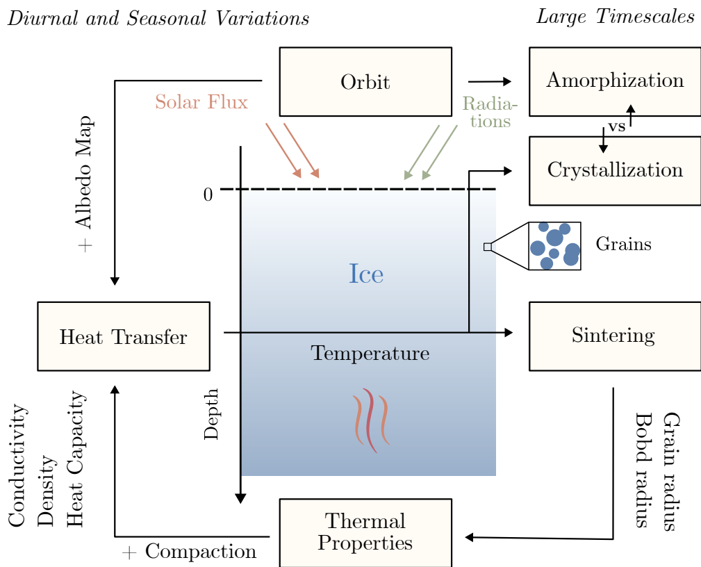
Figure 1.23: Block diagram of the proposed simulation model LunaIcy showing the multiphysics coupling between each modules.
