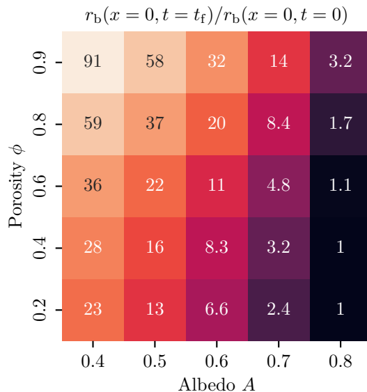
Figure 4.12: Sintering efficiency heatmap for the top layer as a function of porosity and albedo. Colors indicate the ratio of the top layer bond radius after one million years r_b(t = t_f) to the initial bond radius r_b(t = 0) . In the majority of scenarios, the bond radius more than doubles after one million years, except for very high albedo.
