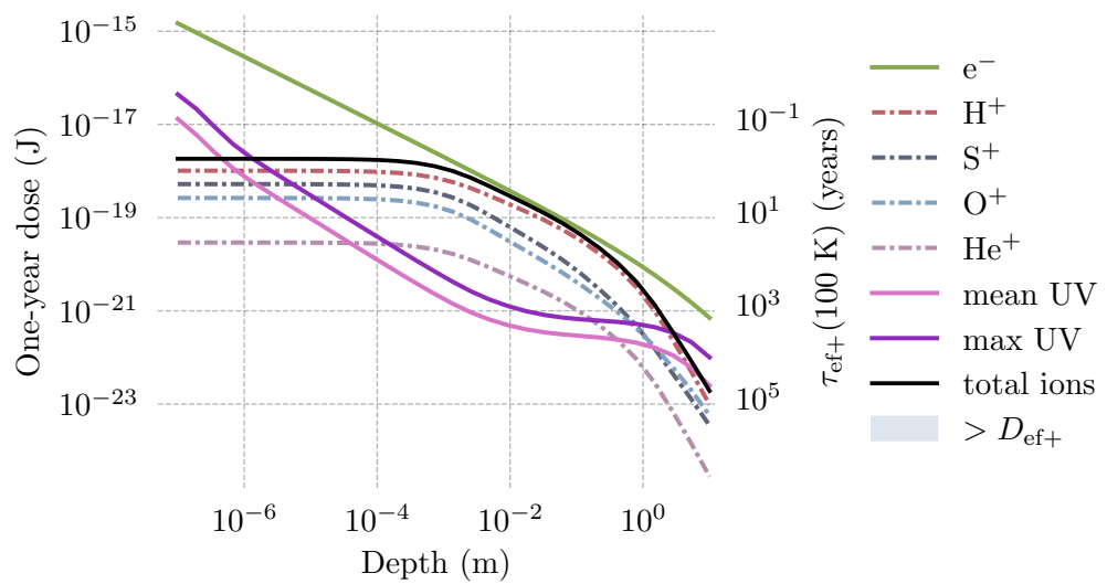
Figure 5.3: One-year irradiation dose penetrating the depths of a pure \text{H}_2\text{O} surface on Europa. Particle-induced doses are represented by dash dots. UV doses are computed at the equator using Europa's mean distance to the Sun 5.20 AU, with the maximum UV corresponding to the highest daily value and the mean UV to the average over the day. The total ion dose is represented by the black line and can be compared with the efficient dose for amorphization D_{\text{ef}+} , illustrated by the blue area.
