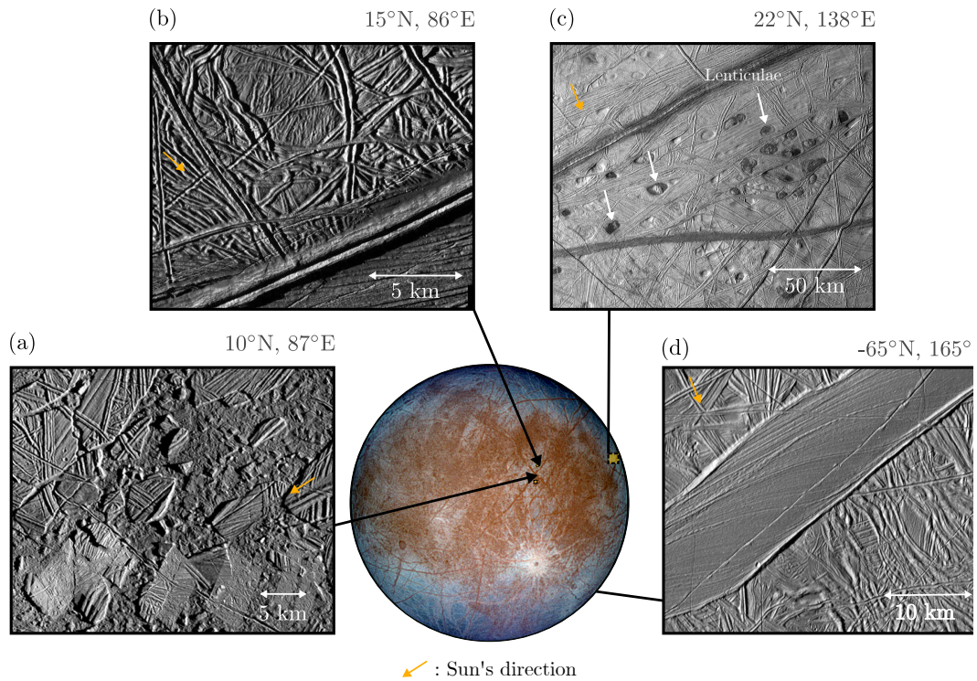
Figure 1.9: Satellite images of different surfaces features mapped to a composite representation of Europa: (a) Ice raft in the Conamara Chaos region (10° N, 87° E); (b) Double ridges separating a ridge plain and a smooth terrain, north from the Conamara Chaos region (15° N, 86° E); (c) Low albedo features: spots, pits and ridges, north-west of Rhadamanthys Linea (22° N, 138° E); (d) A smooth band opened a ridge plain, showing evidence of extension at -65° N, 165° E.
