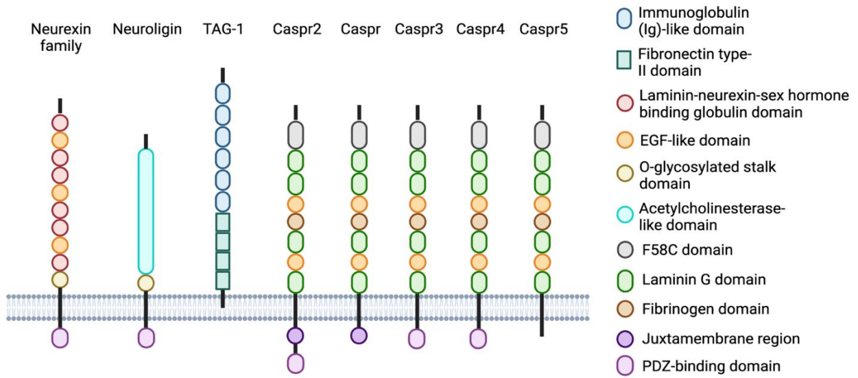
Figure 7: Cell adhesion molecules and their structure.
