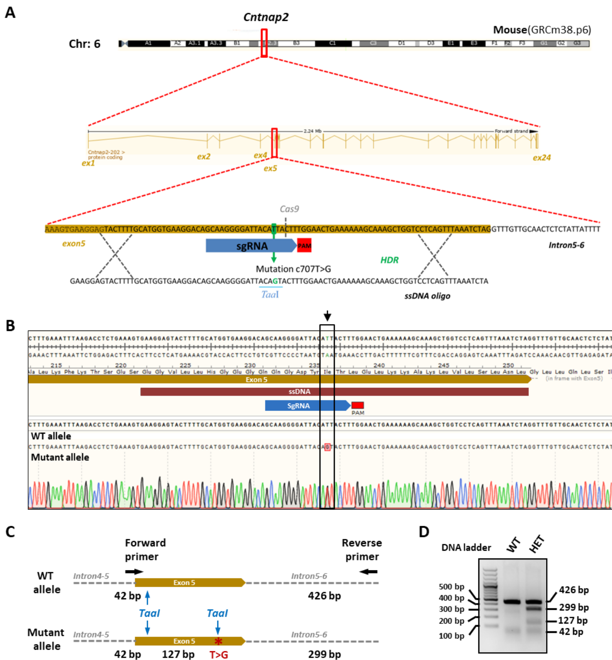
Supplementary Figure S1 | Generation of KI-I236S mice and genotyping. (A) Schema of the sgRNA CRISPR/Cas9 strategy used to generate the mutant mice, showing Cntnap2 genomic locus and the sgRNA sequence. The mutation c707T>G in Cntnap2 exon 5 leads to the introduction of a digestion site for the restriction enzyme Taal (HpyCH4III) site. (B) Validation of the mutation by sequencing. (C) Schema of the genotyping strategy by PCR of tail-tip genomic DNA with primers Forward and Reverse amplifying a 468-bp product, and subsequent digestion with Taal leading to 2 products for the WT allele (426 bp, 42 bp), and three products for the mutant allele (299 bp, 127bp, 42 bp). (D) PCR analysis on genomic DNAs of WT and HET mice (2% agarose gel, 100 bp ladder).
