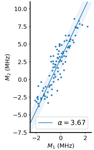
Figure 8.3: Measured data for phase measurement. The amplification factor is fixed for a fixed number of atoms at the same temperature and a fixed delay between measurements. The combination of M_1 and M_2 allows us to assign a phase value to the cycle, and our uncertainty is given by how much our data points spread around the corresponding line for a given phase value. The shading in this case shows \pm\sqrt{\text{Var}(M_2|M_1)} .
