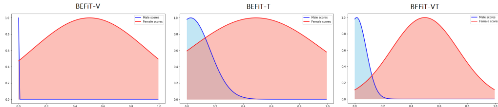
Figure 5.4: Scores distribution for male and female classes for gender classification via BEFiT model.
