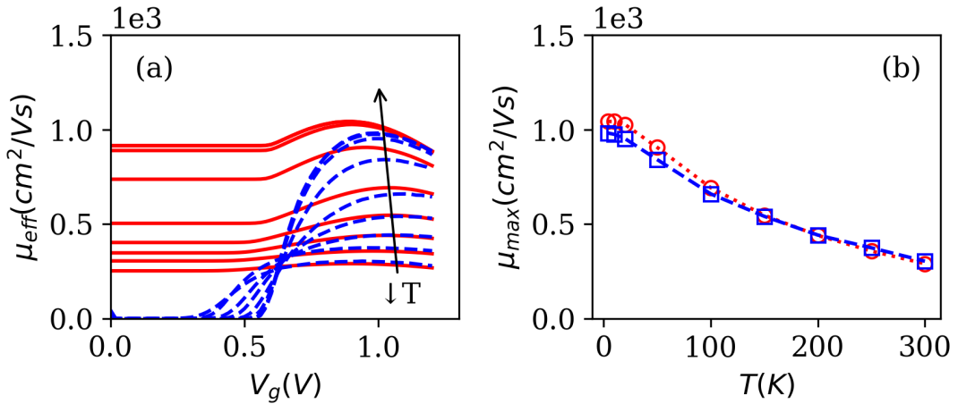
Figure 3.22: (a) \mu_{\text{eff}} variations with V_g and (b) maximum \mu_{\text{eff}} variations with temperature as obtained from Lambert-W function fits (red lines) and split C-V technique (blue dashed lines). ( V_d = 50 mV, W_g = L_g = 10 \mu\text{m} ) [129]
