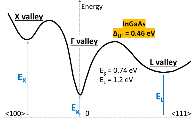
Figure 4.14: Band structure of InGaAs [56]
