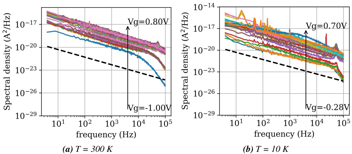
Figure 4.11: Power spectral density of a device with W_g = 5 \mu\text{m} and L_g = 500 \text{ nm}
