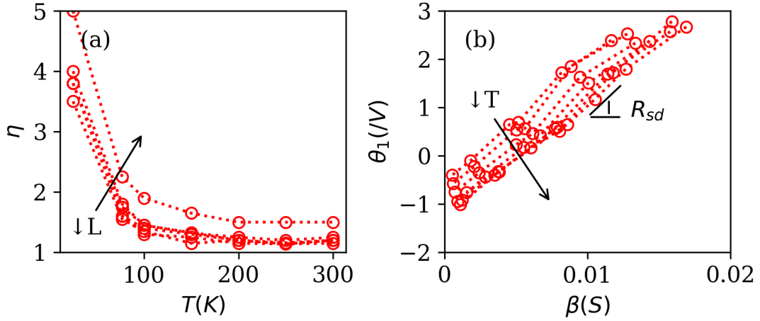
Figure 3.28: (a) \eta parameter variations with temperature for various gate lengths L (nm) = 30, 60, 90, 120, 300 and 1000. (b) \theta_1 parameter variations with \beta = W \cdot C_{ox} \cdot \mu_0 / L gain factor for various temperatures T (K) = 25, 77, 100, 150, 200, 250 and 300 ( W_g = \mu m ) [129]
