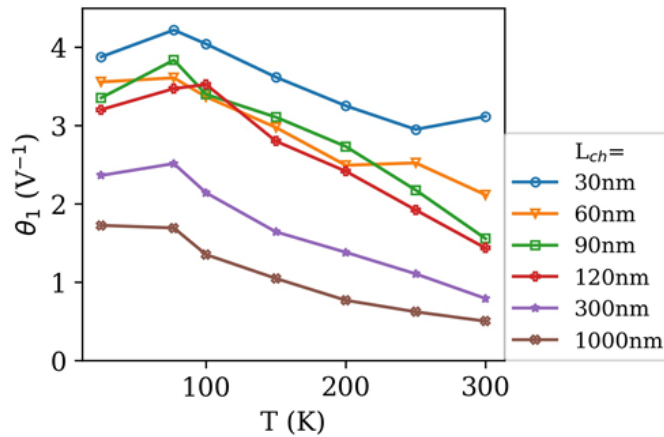
Figure 3.12: Extracted first-order attenuation factor \theta_1 for all measured devices, with respect to temperatures [121]
