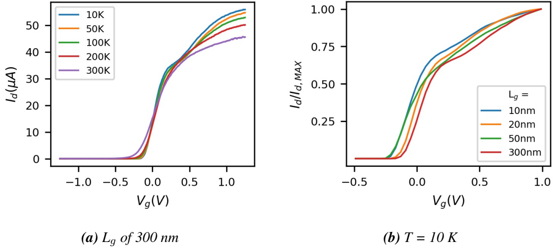
Figure 4.15: Transfer characteristics in linear region of operation ( V_d = 30 mV)
