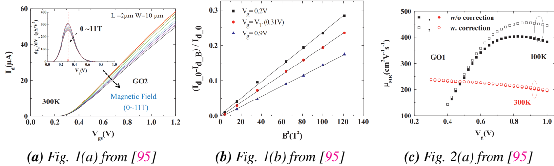
Figure 1.12: (1.12a) Transfer characteristic at linear region for different B values at 300 K for a ( W = 10 \mu\text{m} and L = 2 \mu\text{m} ) device. (1.12b) Relative drain current variation versus B^2 at V_{gs} = 0.2 \text{ V}, 0.31 \text{ V}, 0.9 \text{ V} . (1.12c) \mu_{MR} without/with R_{SD} correction in ( L_g = 300 and 120 \text{ nm} ) devices as function of gate voltage at 100 K and 300 K
