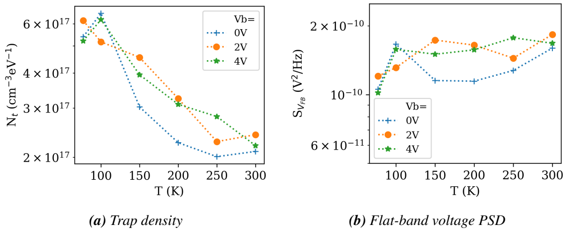
Figure 3.17: Extracted noise parameters for FDSOI 28 nm
