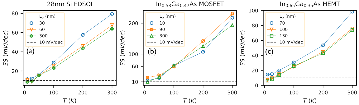
Figure 6.6: Extracted subthreshold swing with respect to temperature; (a) F.3.11; (b) F.4.5; (c) F.5.3b
