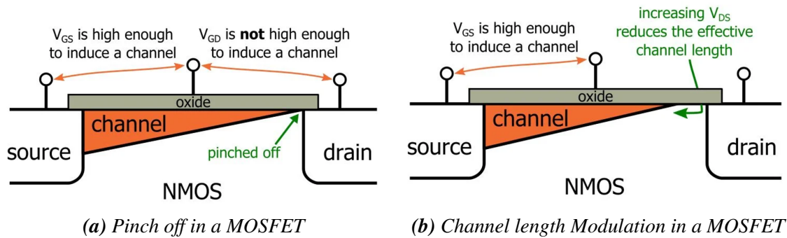
Figure 1.6: MOSFET saturation [31]
