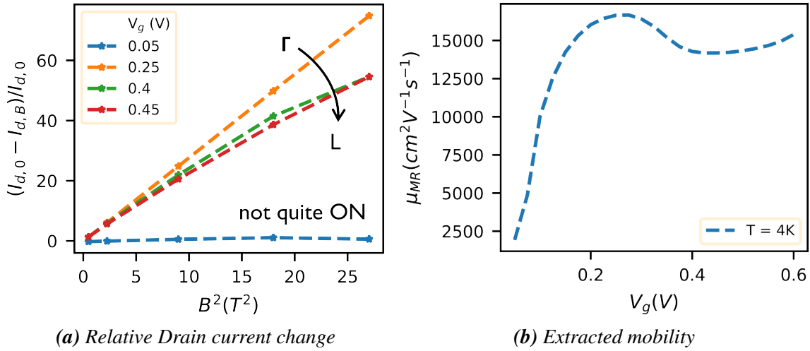
Figure 5.25: 4 K magnetoresistance processing for a HEMT device with W_g = 100 \mu m and L_g = 100 nm
