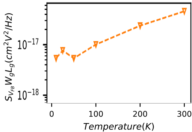
Figure 4.13: Normalized PSD of flat-band voltage with respect to W_g L_g
