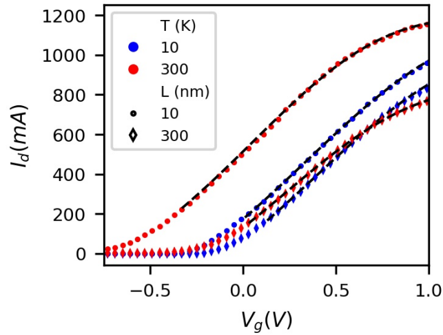
Figure 4.7: . Drain current versus gate voltage at V_d = 1 V for L = 10 and 300 nm at T = 10 and 300 K. the dashed line shows the fit reconstructed with the parameters extracted thanks to the Y function [149]
