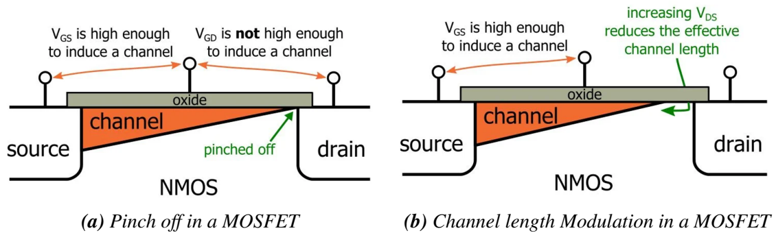
Figure 1.6: MOSFET saturation [31]
