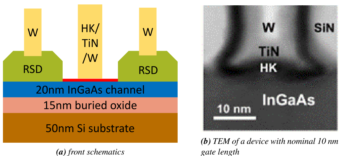
Figure 4.1: Structure of the InGaAs-OI MOSFETs under study. Courtesy of IBM Zurich [146, 147]
