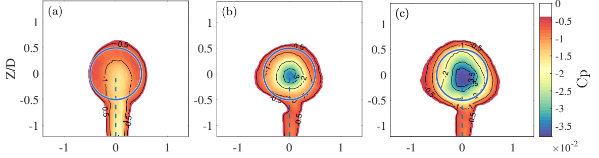
Figure 4.12: Reconstructed pressure coefficient C_P for (a) the \alpha = 0^\circ case, (b) the \alpha = 15^\circ case and for (c) the \alpha = 25^\circ case evaluated at X = 2D . Solid blue line: porous disc edges, dashed blue line: mast outline.
