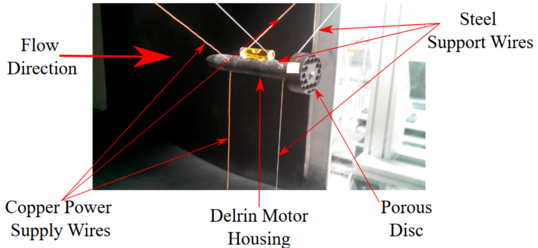
Figure 3.3: Experimental set-up of the porous disc generating a swirling wake used in the work of Holmes and Naughton (2022).
