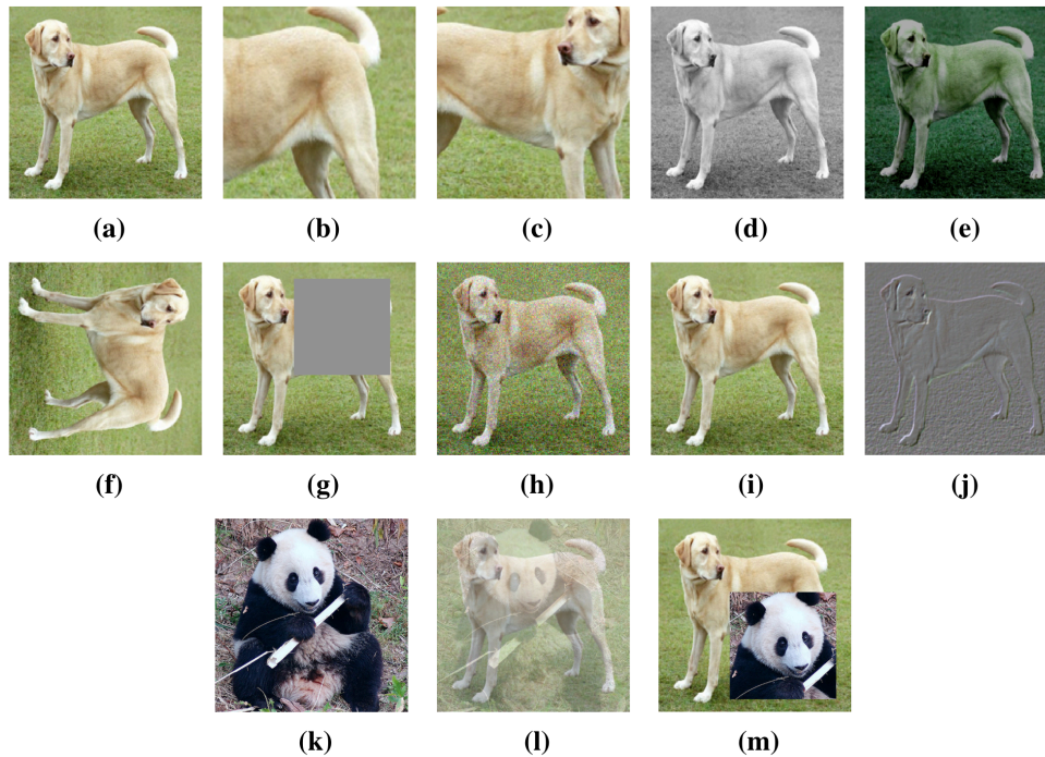
Figure 2.9 – Illustrations of the various data augmentation used in self-supervised learning. Given an example image in (a), the label-preserving augmentations from (b) to (j) are: (b) Crop + resize, (c) Crop + resize + flip, (d) Color distortion (channel drop), (e) Color distortion (jitter), (f) Rotation, (g) Cutout, (h) Gaussian noise, (i) Gaussian blur and (j) Sobel filtering. Provided another image in (k), semantic transformations of (a) and (k) are (l) MixUp and (m) CutMix. Each augmentation operation has one or more parameters determining the output image. The images in (a) to (j) are taken from [Chen, 2020b], and the image in (k) is from ImageNet [Russakovsky, 2015].
