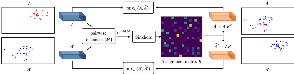
Figure 3.2 – Feature tensor alignment and interpolation. Cost matrix M contains pairwise distances of feature vectors in tensors \mathbf{A}, \mathbf{A}' . Assignment matrix R is obtained by Sinkhorn-Knopp [Knight, 2008] on similarity matrix e^{-M/\epsilon} . \mathbf{A} is aligned to \mathbf{A}' according to R , giving rise to \tilde{\mathbf{A}} . We then interpolate between \mathbf{A}, \tilde{\mathbf{A}} . Symmetrically, we can align \mathbf{A}' to \mathbf{A} and interpolate between \mathbf{A}', \tilde{\mathbf{A}}' . \mathbf{A}, \mathbf{A}' on the left (toy example of 16 points in 2D) shown semi-transparent on the right for reference.
