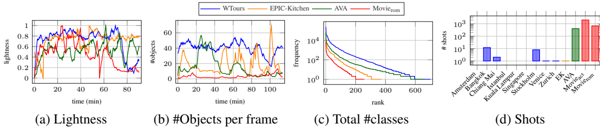
Figure 6.2 – Dataset analysis of a WTours video compared with videos from Epic-Kitchens [Damen, 2022], AVA [Gu, 2018] and two entire movies, concatenated or cropped to match the duration of the WTours video. (a) Lightness vs. time. (b) Number of objects per frame vs. time. (c) Frequency of classes in entire video. (d) Number of shots. Objects detected by Detic [Zhou, 2022b], trained on ImageNet-21k.
