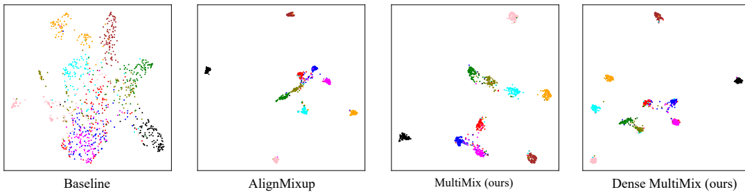
Figure 5.3 – Embedding space visualization for 100 test examples per class of 10 randomly chosen classes of CIFAR-100 with PreActResnet-18, using UMAP [McInnes, 2018].
