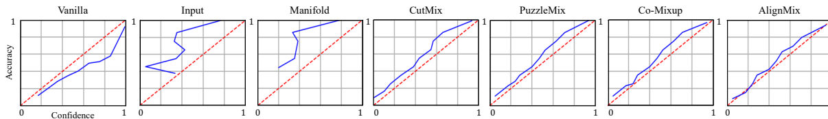
Figure 3.4 – Calibration plots on CIFAR-100 using PreActResnet18: near diagonal is better. Baseline is clearly overconfident while Input and Manifold mixup are clearly underconfident. AlignMixup has the best calibrated predictions.
