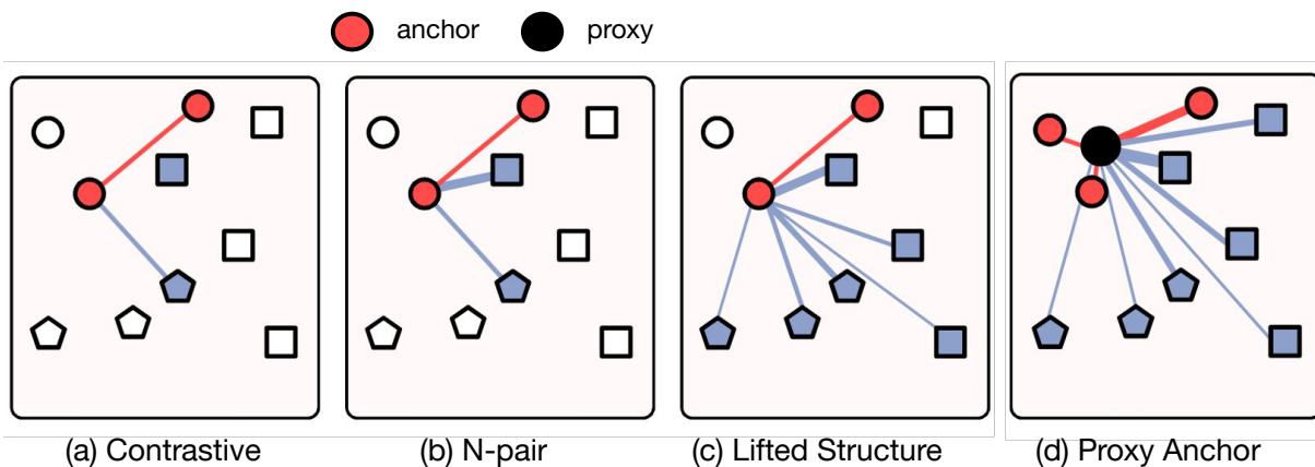
Figure 2.6 – A visual comparison of different pair-based losses (contrastive, N-pair and Lifted Structure) and Proxy based loss (Proxy Anchor) in deep metric learning. The thickness of the lines denotes the strength of the similarity between the examples. The images were adapted from [Kim, 2020c]
