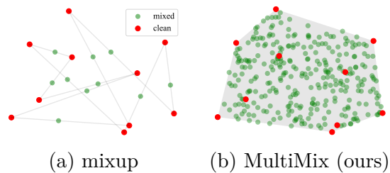
Figure 5.1 – Data augmentation in a mini-batch B of b = 10 points in two dimensions. (a) mixup : sampling n = b points on linear segments between b pairs of points using the same interpolation factor \lambda . (b) MultiMix : sampling n = 300 points in the convex hull of B .
