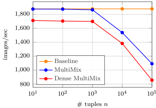
Figure 5.5 – Training speed (images/sec) of MultiMix and its variants vs. number of tuples n on CIFAR-100 using R-18. Measured on NVIDIA RTX 2080 TI GPU, including forward and backward pass.
