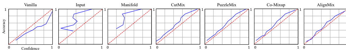
Figure 3.4 – Calibration plots on CIFAR-100 using PreActResnet18: near diagonal is better. Baseline is clearly overconfident while Input and Manifold mixup are clearly underconfident. AlignMixup has the best calibrated predictions.
