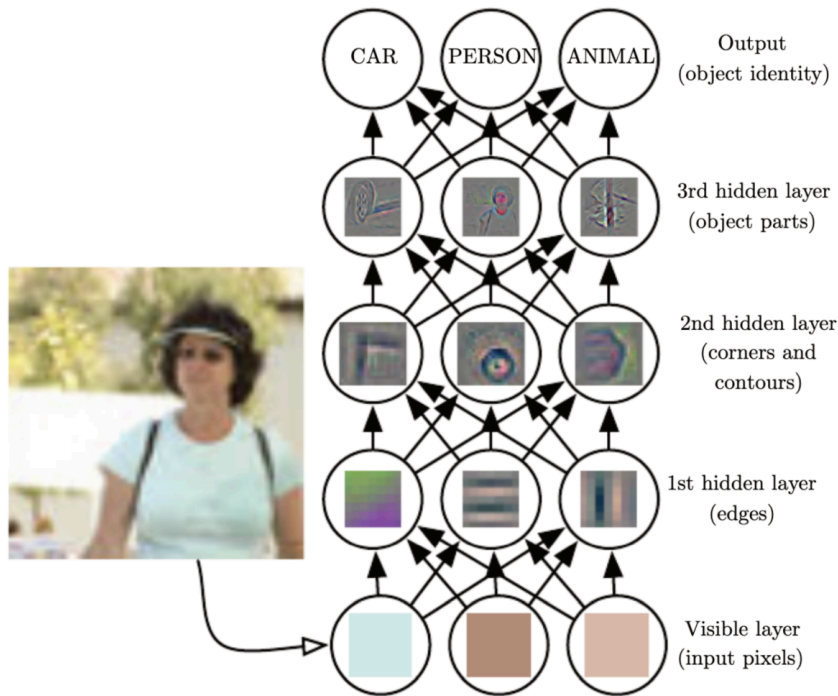
Figure 1.1 – Illustration on the ability of deep neural networks to learn hierarchical representations of images. Given input images composed of pixels, low-level representations (e.g., edges) are encoded first, which are combined to form higher-level representations (e.g., object parts) that can be used to solve the task at hand, e.g., image classification. Figure adapted from [Goodfellow, 2016]
