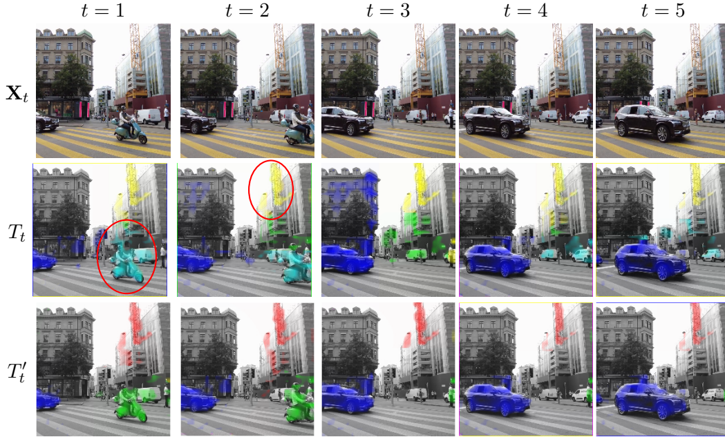
Figure 6.4 – For each input frame t of a video clip (top), cross-attention map T_t \in \mathbb{R}^{k \times n} (6.3) (middle) and refined cross-attention map T'_t \in \mathbb{R}^{k \times n} (6.6) (bottom), using Sinkhorn-Knopp algorithm. For each object, one row of T_t or T'_t is reshaped as h/p \times w/p and upsampled to an h \times w attention map overlaid on the input frame for k = 3 objects encoded in blue, red and green channel. Mixed colors yellow and cyan for T_t (middle, in red circle) indicate spatial overlap of two objects, while T'_t (bottom) yields three well separated objects shown in primary colors blue, red and green.
