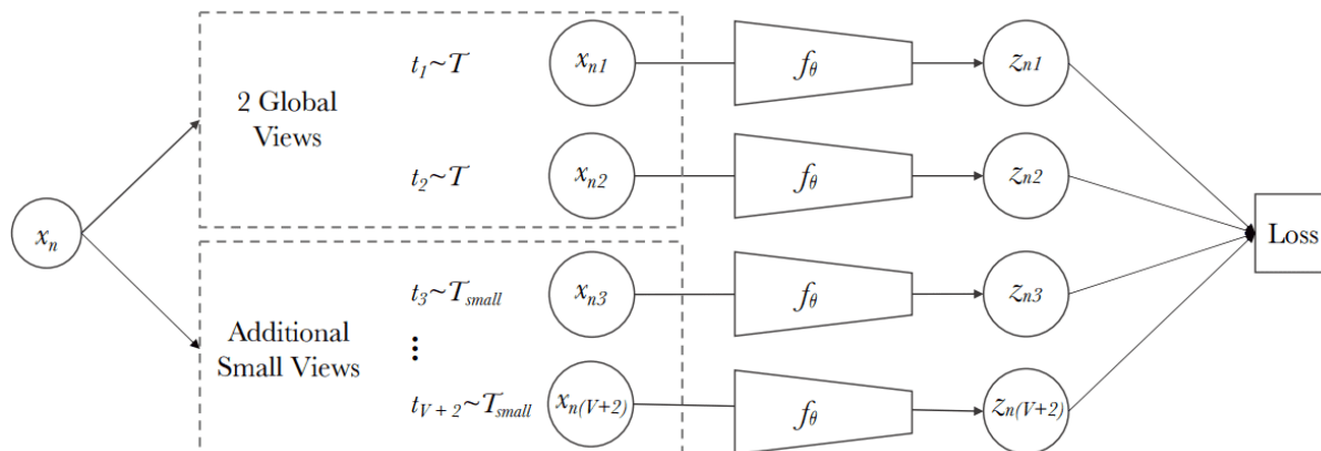
Figure 2.10 – The multi-crop strategy for data augmentation in self-supervised learning. The image x_n is transformed into V + 2 views: two global views and V small resolution zoomed views. This strategy has been widely adopted in DINO, IBoT etc. Image source [Caron, 2020].
