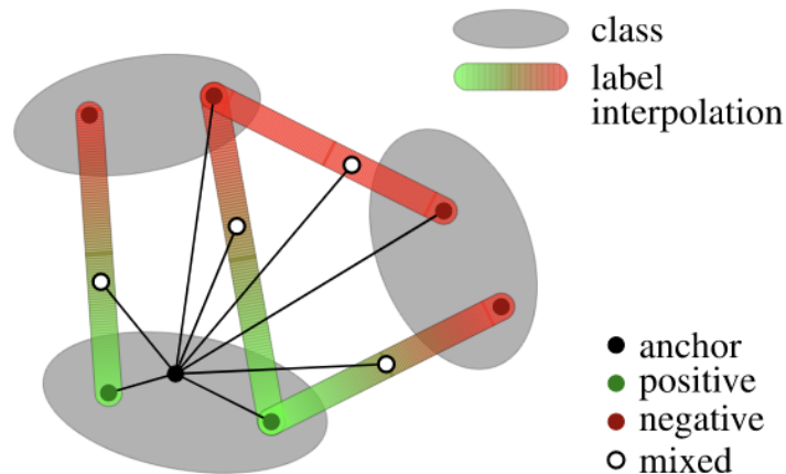
Figure 4.1 – Metrix (= Metric Mix ) allows an anchor to interact with positive (same class), negative (different class) and interpolated examples, which also have interpolated labels.
