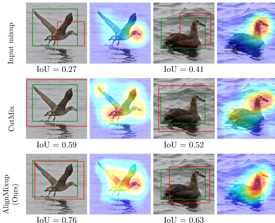
Figure 3.5 – Localization examples using ResNet-50 on CUB200-2011. Red boxes: predicted; green: ground truth.
