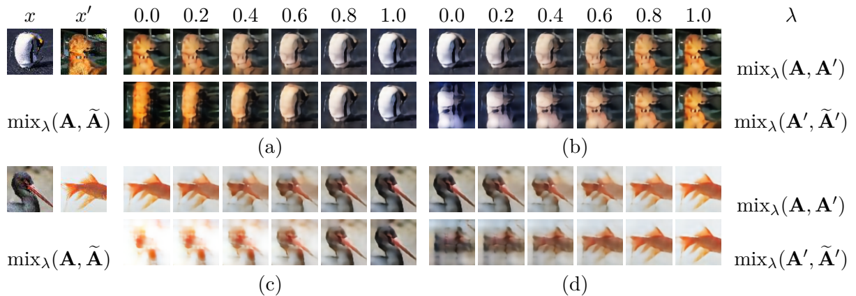
Figure 3.3 – Visualizing alignment . For different \lambda \in [0, 1] , we interpolate feature tensors \mathbf{A}, \mathbf{A}' without alignment (top) or aligned feature tensors (bottom) of two images x, x' and then we generate a new image by decoding the resulting embedding through the decoder D . (a), (c) We align \mathbf{A} to \mathbf{A}' and mix with (3.12). (b), (d) We align \mathbf{A}' to \mathbf{A} and mix with (3.13). Only meant for illustration: No decoded images are seen by the classifier at training.
