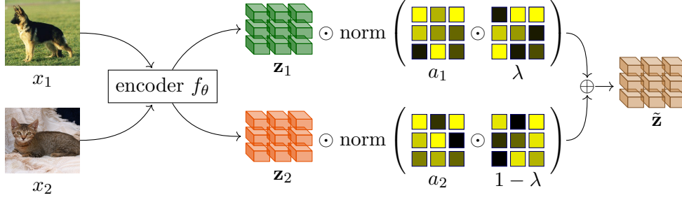
Figure 5.2 – Dense MultiMix (subsection 5.3.3) for the special case m = 2 (two examples), n = 1 (one interpolated embedding), r = 9 (spatial resolution 3 \times 3 ). The embeddings \mathbf{z}_1, \mathbf{z}_2 \in \mathbb{R}^{d \times 9} of input images x_1, x_2 are extracted by encoder f_\theta . Attention maps a_1, a_2 \in \mathbb{R}^9 are extracted (5.9), multiplied element-wise with interpolation vectors \lambda, (1 - \lambda) \in \mathbb{R}^9 (5.10) and \ell_1 -normalized per spatial position (5.11). The resulting weights are used to form the interpolated embedding \tilde{\mathbf{z}} \in \mathbb{R}^{d \times 9} as a convex combination of \mathbf{z}_1, \mathbf{z}_2 per spatial position (5.12). Targets are interpolated similarly (5.13).
