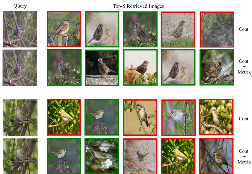
Figure 4.3 – Retrieval results on CUB200 using Contrastive loss, with and without mixup. For each query, the top-5 retrieved images are shown. Images highlighted in green (red) are correctly (incorrectly) retrieved images.
