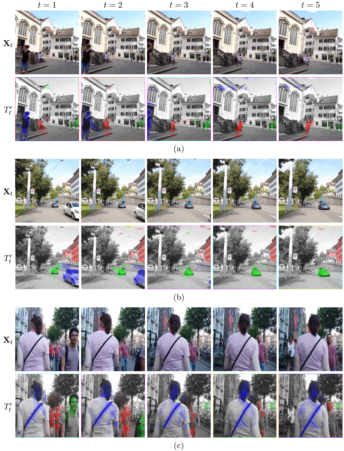
Figure 6.6 – For each input frame X_t of a video clip, refined cross-attention map T'_t \in \mathbb{R}^{k \times n} (6.6), using Sinkhorn-Knopp. For each object, one row of T'_t is reshaped as h/p \times w/p and upsampled to an h \times w attention map overlaid on the input frame for k = 3 objects encoded in blue, red and green channel. T'_t fields three well separated objects shown in blue, red and green.
