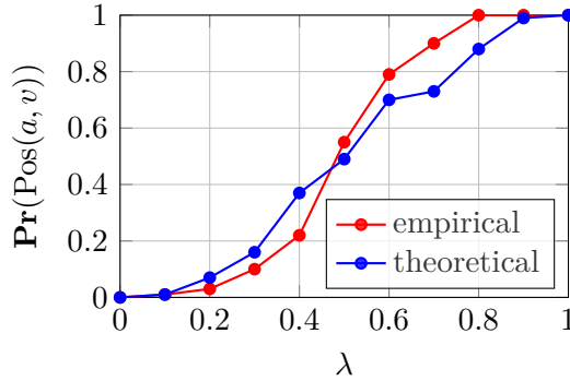
Figure 4.2 – “Positivity” of mixed embeddings vs. \lambda . We measure \Pr(\text{Pos}(a, v)) empirically as \Pr(\partial \tilde{\ell}_{\text{MS}}(a; \theta) / \partial s(a, v) \leq 0) and theoretically by (4.14), where F_\lambda is again measured from data. We use embedding mixup on MS (4.2) on CUB200 at epoch 0, based on the setup of subsection 4.4.1.
