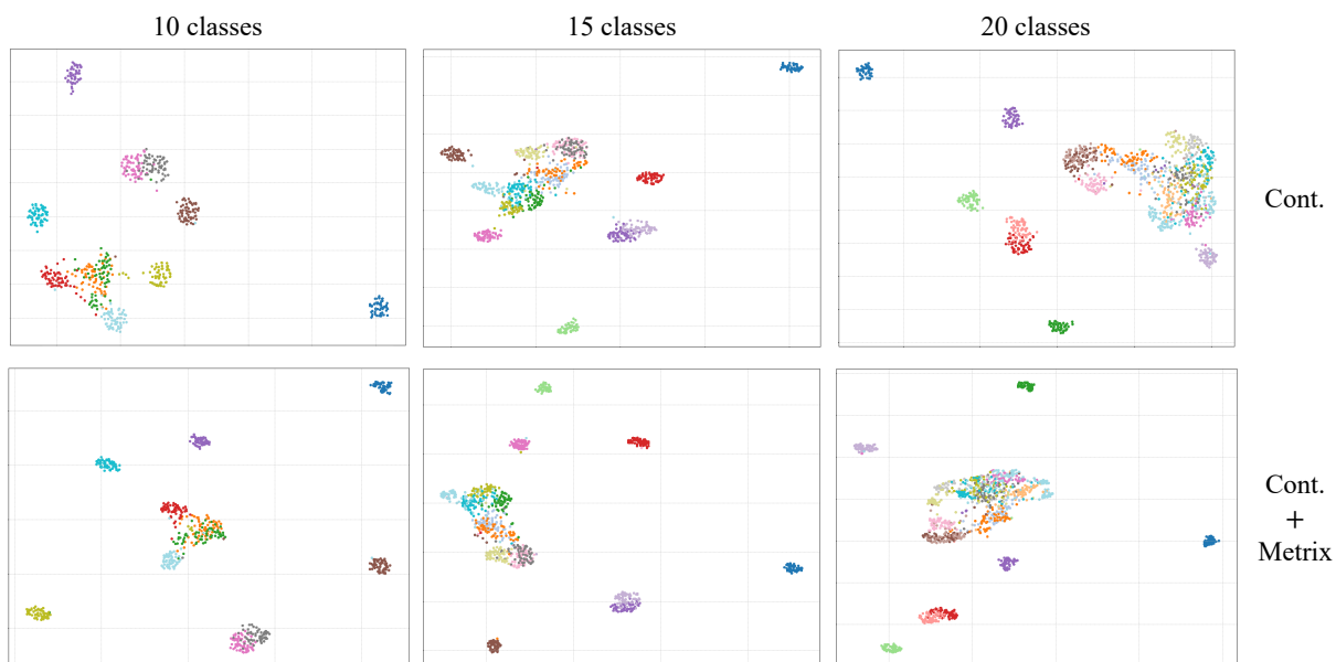
Figure 4.4 – Embedding space visualization of CUB200 test examples of a given number of classes using Contrastive loss, with and without mixup.
