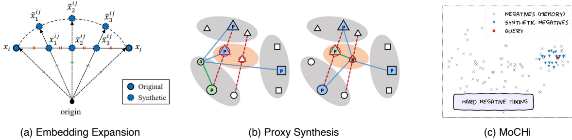
Figure 2.8 – Different methods that perform mixup in the embedding space to generate more synthetic negatives for metric learning. The images were adapted from [Ko, 2020], [Kalantidis, 2020] and [Gu, 2021].
