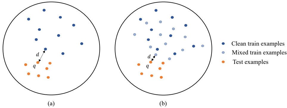
Figure 4.5 – Exploring the embedding space when using (a) only clean examples (b) clean and mixed examples. Given a query q , the distance d to its nearest training embedding (clean or mixed) is smaller with mixup (b) than without (a).
