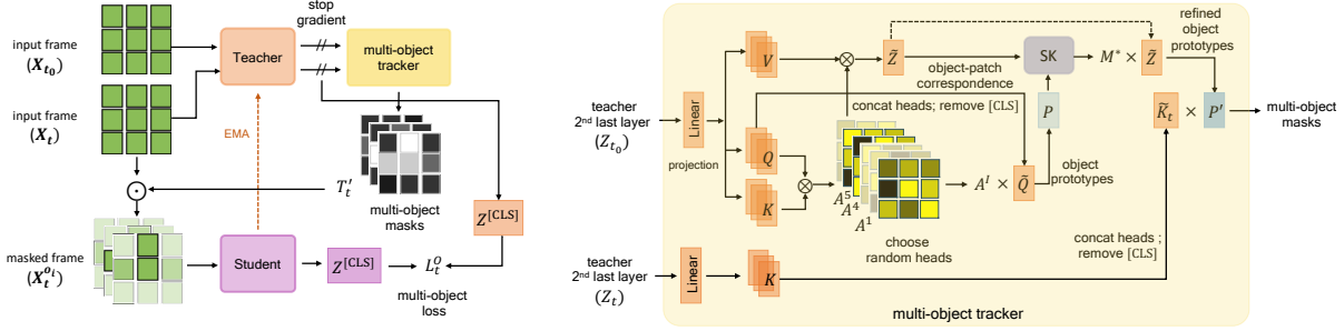
Figure 6.3 – DORA , our self-supervised image pretraining method from video. (Left) From an input frame \mathbf{X}_{t_0} , the output of the second-last layer of the teacher model is used by a multi-object tracker to generate cross-attention maps T'_t with frame \mathbf{X}_t . We use those to mask \mathbf{X}_t (6.7), feed it to the student model and apply a distillation loss L_t^O between [CLS] token embeddings (6.8). (Right) In the tracker, we obtain the query Q , key K and output Z embeddings. From the multi-head attention maps A^i (6.1), we draw a subset \mathcal{I} of k heads and form object prototypes P by pooling over patch queries \tilde{Q} (6.2). We refine them into P' to discover distinct objects , using Sinkhorn-Knopp (SK) to establish correspondences M^* between P and patch embeddings \tilde{Z} (6.4) and pooling over \tilde{Z} (6.5). We then track the objects over frames \mathbf{X}_t by cross-attention T'_t with patch key embeddings \tilde{K}_t (6.6).
