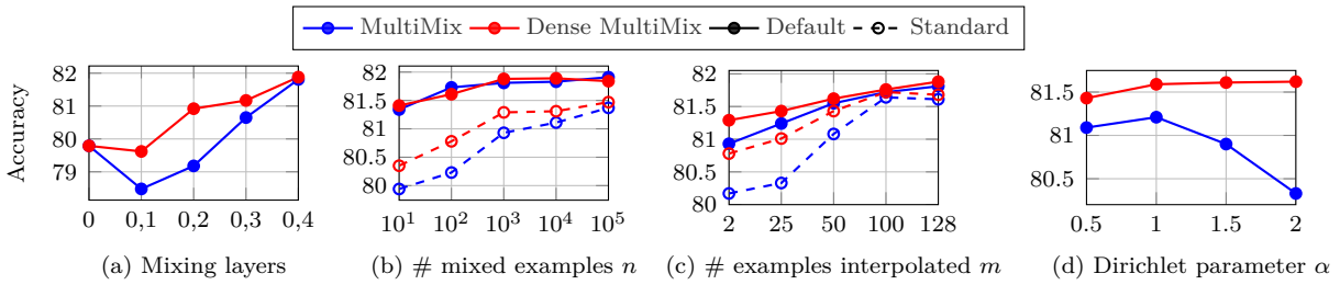
Figure 5.4 – Ablation study on CIFAR-100 using R-18. (a) Interpolation layers (R-18 block; 0: input mixup). (b) Number n of interpolated examples per mini-batch with m = b (Default) and m = 2 (Standard). (c) Number m of examples being interpolated, with n = 1000 (Default) and n = 100 (Standard). (d) Fixed value of Dirichlet parameter \alpha .
