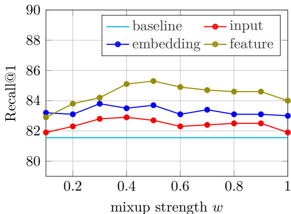
Figure 4.6 – Effect of mixup strength for different mixup types using contrastive loss and R-50 with embedding size d = 512 on Cars196. Recall@ K (%): higher is better.
