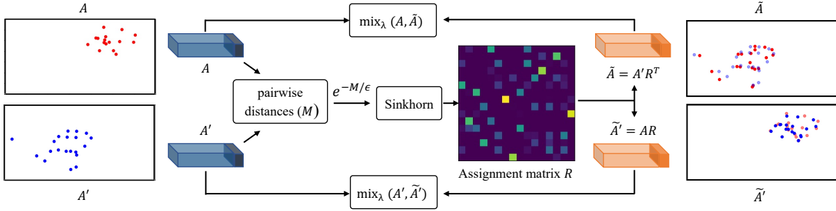
Figure 3.2 – Feature tensor alignment and interpolation. Cost matrix M contains pairwise distances of feature vectors in tensors \mathbf{A}, \mathbf{A}' . Assignment matrix R is obtained by Sinkhorn-Knopp [Knight, 2008] on similarity matrix e^{-M/\epsilon} . \mathbf{A} is aligned to \mathbf{A}' according to R , giving rise to \tilde{\mathbf{A}} . We then interpolate between \mathbf{A}, \tilde{\mathbf{A}} . Symmetrically, we can align \mathbf{A}' to \mathbf{A} and interpolate between \mathbf{A}', \tilde{\mathbf{A}}' . \mathbf{A}, \mathbf{A}' on the left (toy example of 16 points in 2D) shown semi-transparent on the right for reference.
