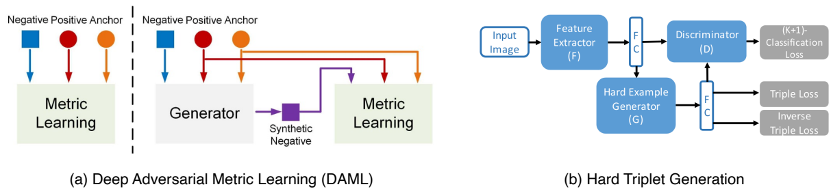
Figure 2.7 – A visual comparison of different methods that generate synthetic samples using generative models for metric learning. The images were adapted from [Zhao, 2018] and [Zhao, 2018].
