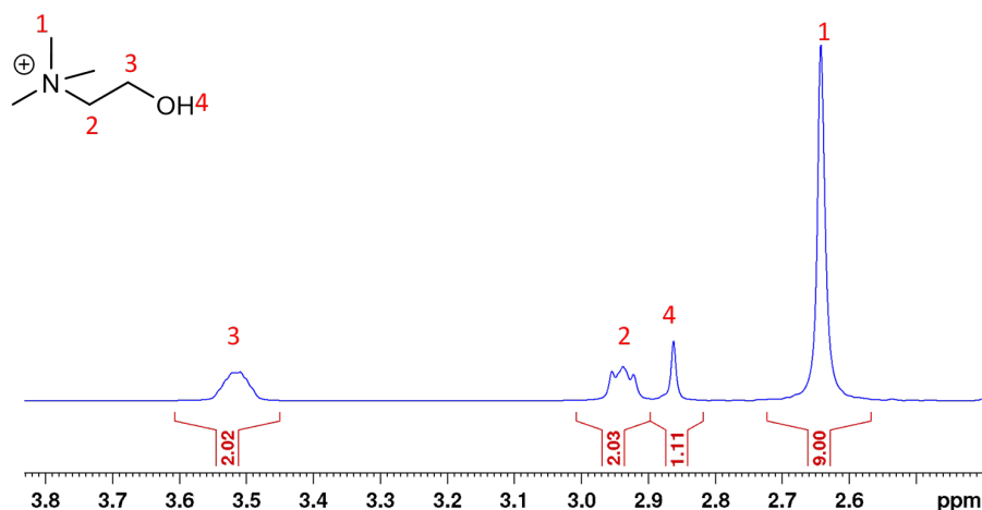
Figure 4.12: ^1\text{H} NMR spectrum of dry [Chol][TFSI] at 40 °C, with a capillary of DMSO- \text{D}_6 , resonance assignments are indicated by the numbers in red above the spectrum.
