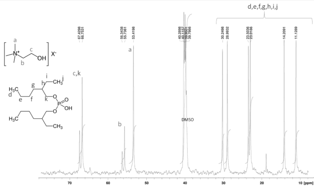
Figure A.3: ^{13}\text{C} NMR spectrum of [Chol][D2EHP] in DMSO. ^{13}\text{C} NMR (500 MHz, [D 6 ]DMSO, TMS): 11.12 (4CH 3 ), 13.66 (2CH 3 ), 14.01 (2CH 3 ), 19.71 (4CH 2 ), 23.14 (2CH 2 ), 23.32 (2CH 2 ), 24.07 (4CH 2 ), 29.06 (2CH 3 ), 30.12 (2CH 2 ), 40.43 (2CH), 58.70 (3NCH 3 ), 53.41 (OCH 2 ), 56.35 (NCH 2 ), 67.27 (2OCH 2 )
