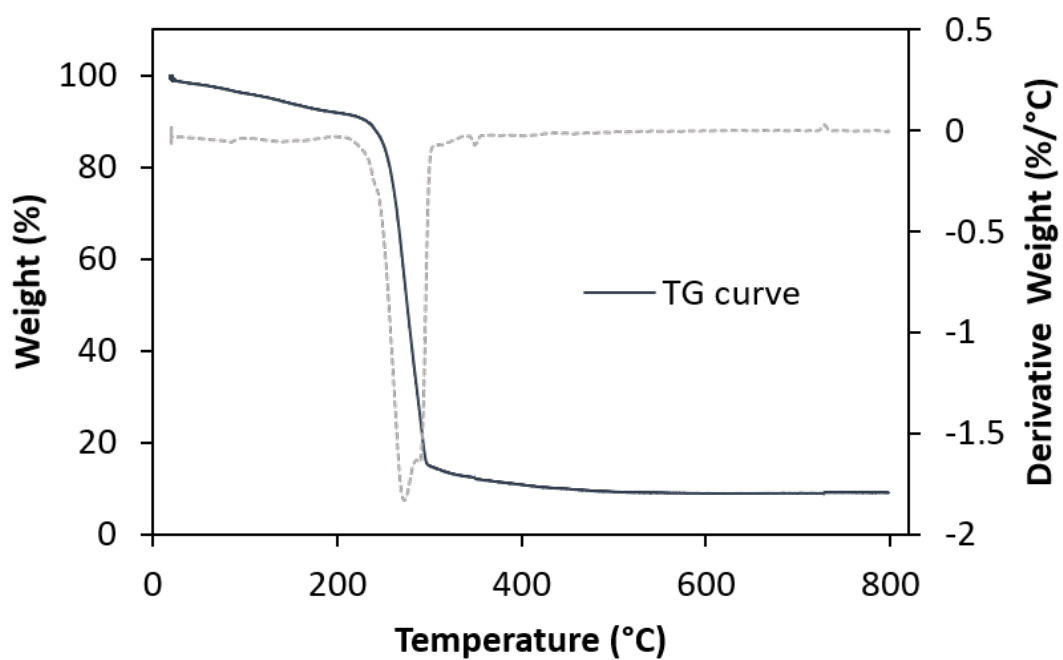
Figure A.4: Thermal gravimetric analysis (TGA) of [Chol][D2EHP] (20°C to 800 °C, 2 °C/min, in N 2 atmosphere).
