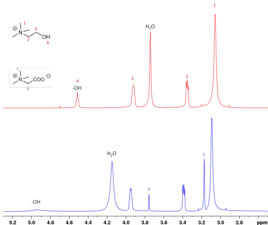
Figure 4.16: ^1\text{H} NMR spectra for (a) (top) [Chol][TFSI] saturated in \text{H}_2\text{O} (b) (bottom) ionic liquid phase after extraction with the initial parameters: \text{IL}:\text{aq} = 2:1 , [\text{Li}]_{\text{aq}}^0 = 1 \text{ M} , [\text{betaine}]_{\text{aq}}^0 = 24\% \text{ w/w} .
