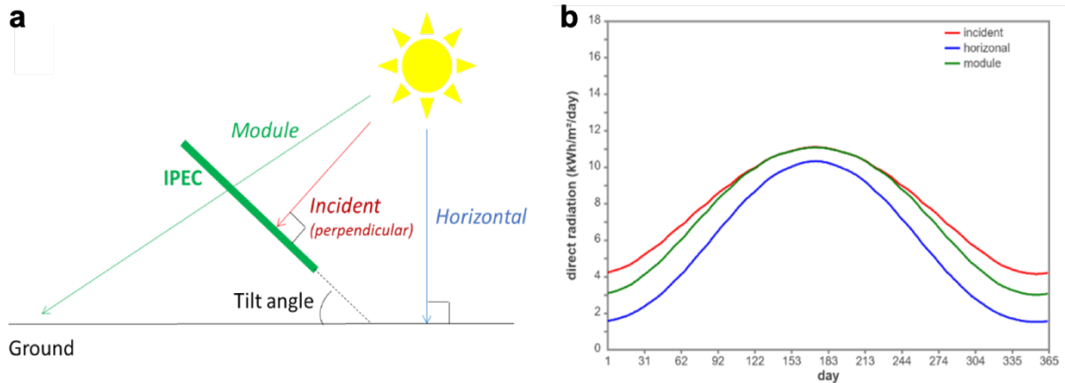
Figure 56. Direct radiation striking a tilted plane. a) Schem of the IPEC modules, tilted 25^\circ against the horizontal. b) Calculated direct radiation on the IPEC modules (in green), on the horizontal plane (in blue), and on the plane always perpendicular to the sun thanks to a light tracker. The latitude was 45^\circ N. Day on the abscissa is the number of days since January 1 st . The ratio of irradiances used to correct the GHI for STH^* calculation is 0.9. Figure and calculations adapted from 208 .
