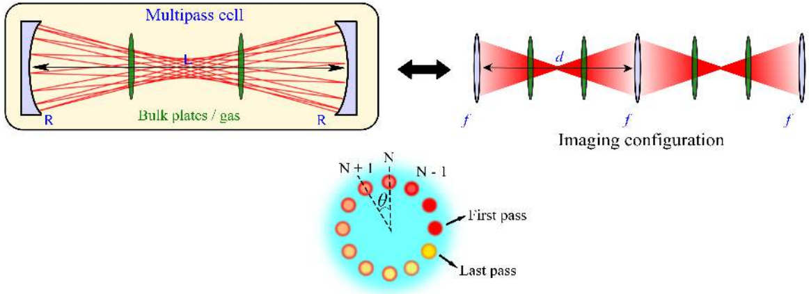
Figure 3.2: MPC geometry
