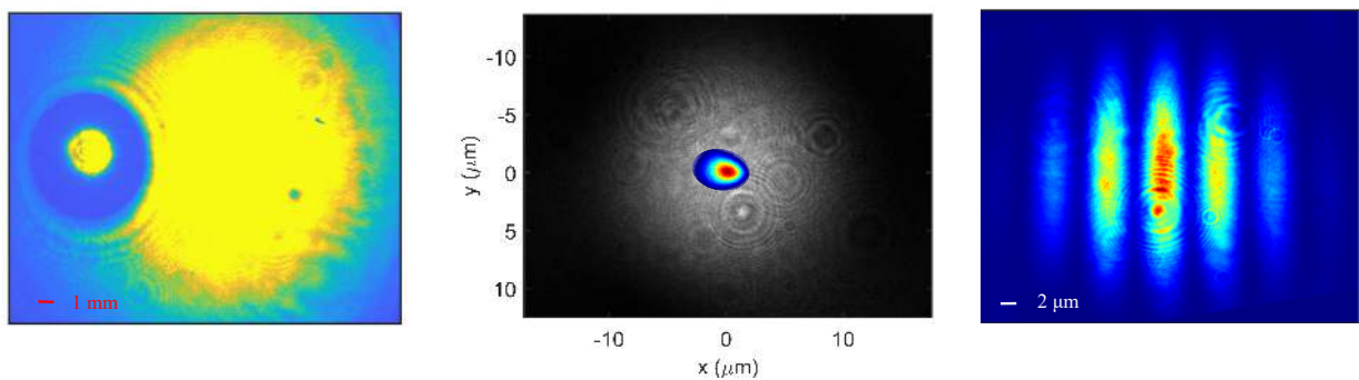
Figure 5.2: A near-field snapshot of the recombined Prepulse and Main pulse (left), on-target Pre-pulse (gray-scale) and Main-pulse (color scale) spatial beam profiles (center), and the interference fringes observed when the Main-pulse and Prepulse overlap in space and time in-focus (right).
