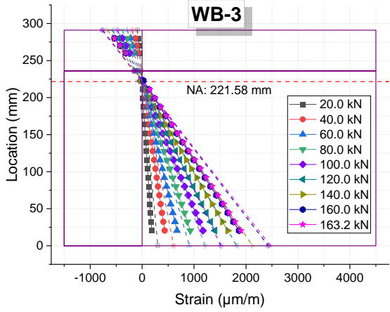
Fig. 3-12 Bending strain distribution of the composite beams at the mid-span cross-section
