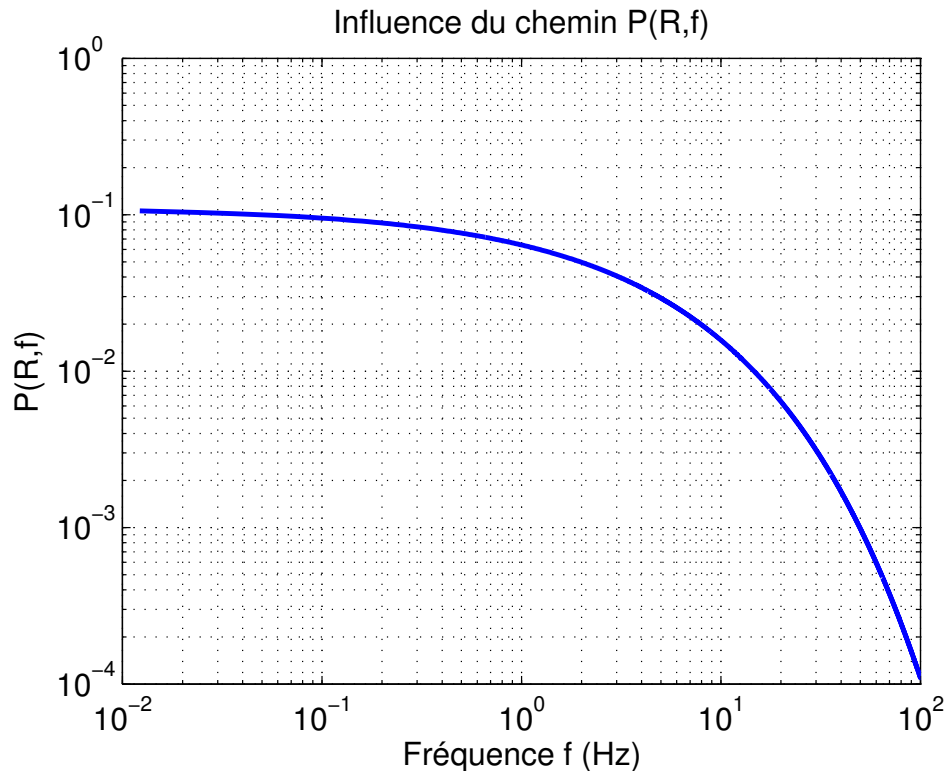
Figure A.2 - Influence du chemin, R = 9 km
