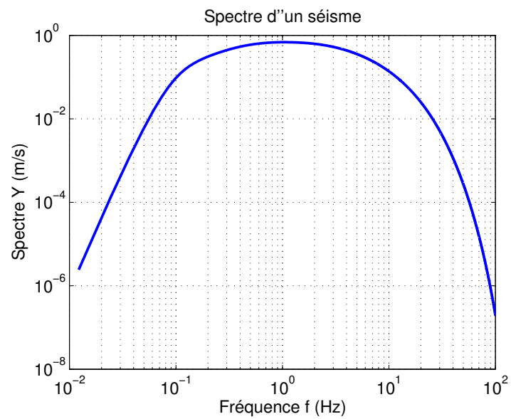
Figure A.4 - Spectre pour M = 7 et R = 9 km
