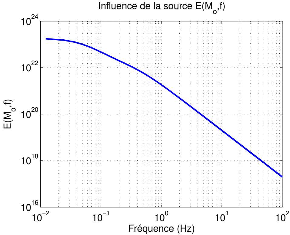
Figure A.1 – Influence de la source, M = 7
