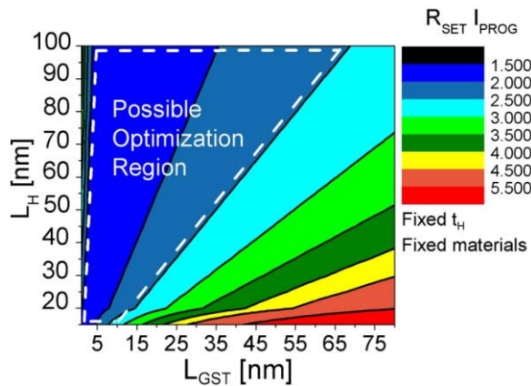
Fig. 1.8 Contour plot of R_{SET} \cdot I_{PROG} as a function of heater height (LH) and GST thickness ( L_{GST} ) with the dash defined area highlighting the optimization area for lower power consumption [41]
