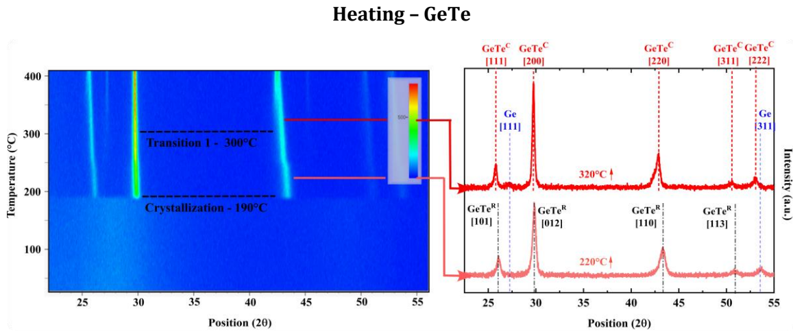
Fig. 4.22. Left: XRD map for in-situ annealing of GeTe during the heating ramp, Right: XRD patterns at 220 and 320°C annealing temperature extracted from the XRD map. PDF card information: c-Ge (04-016-2396), rhombohedral GeTe - GeTe R (01-080-8422), cubic GeTe - GeTe C (04-006-1927)
