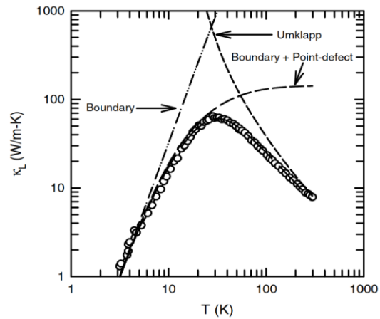
Fig 2.6 The lattice thermal conductivity versus temperature of a \text{CoSb}_3 sample. The dots and the solid line represent the experimental data and the theoretical, respectively. The dashed curves are the theoretical limits imposed on the phonon heat transport by boundary scatterings, a combination of boundary plus point-defect scatterings, and Umklapp scatterings [125]
