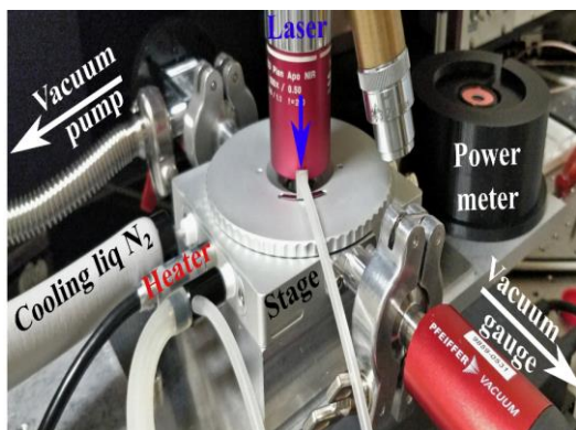
Fig 3.9 Heating/ cooling stage from Linkam – connections showing vacuum gauge, liquid N2 cooling and heater attachment. A Si-photo diode power meter from Thorlabs
