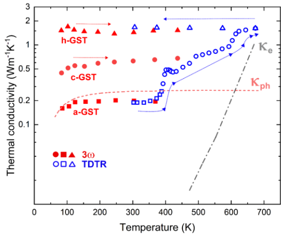
Fig. 5.17 Evolution of thermal conductivity of GST-225 as a function of temperature. Data in blue represents transition of as-deposited material through phase transitions [113], and in red presents data of thermal cycling for pre-annealed samples [114]. Dash and dot-dash lines present the lattice and electronic contribution
