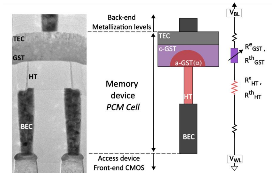
Fig. 1.3 Transmission electron microscopy (TEM) image 6 of PCM cells and an illustration of the PCM cell with GST and heater (HT) sandwiched between top electrode contact (TEC) and bottom contact electrode (BEC) controlled by word line (WL) and bit line (BL). A resistor scheme is presented alongside – GST acts as a variable resistor depending on the phase of the material. \alpha – fraction of material switched
