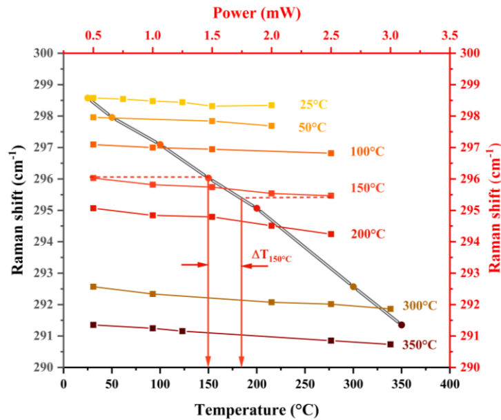
Fig. 5.8. Temperature calibration plot (black axes) with data points connected by double black lines and power calibration plot (red axes) where the colored data points are connected by colored lines (color gradient representing the respective temperature). The power calibration colored data points at 0.5mW align with the temperature calibration data points along the black line. A representative example of local temperature rise caused by a 2.5mW input power for an in-situ measurement performed at 150^\circ\text{C}
