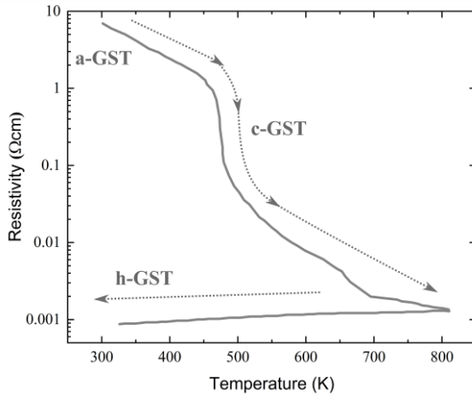
Fig 2.3 Electrical resistivity \rho of GST-225 as a function of temperature with phase transitions [107]
