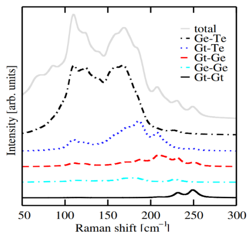
Fig. 4.17. Projection of contribution from different bond and structural configurations on the reduced Raman spectrum of GeTe. [211]
