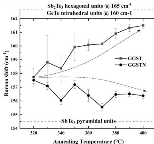
Fig. 4.8. Influence of temperature on the SbTe vibrations in GGST and GGSTN. The dashed arrows present the difference in influence of temperature on these vibrations towards different structural motifs as indicated.
