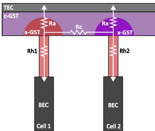
Fig 2.1 Schematic of phase-dependent thermal resistances involved in 2 neighboring PCM cells
