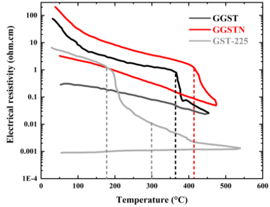
Fig. 4.4. Electrical resistivity vs temperature measurements GGST, GGSTN and GST-225 with phase transitions indicated by dashed lines.
