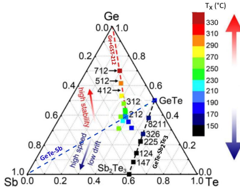
Fig. 1.14: Ge-Sb-Te ternary diagram presenting the crystallization temperature of different compositions ( Ge_xSb_yTe_z - GST-XYZ) as a function of crystallization temperature. The dashed lines present compositions investigated along different pseudo-binary lines [64]
