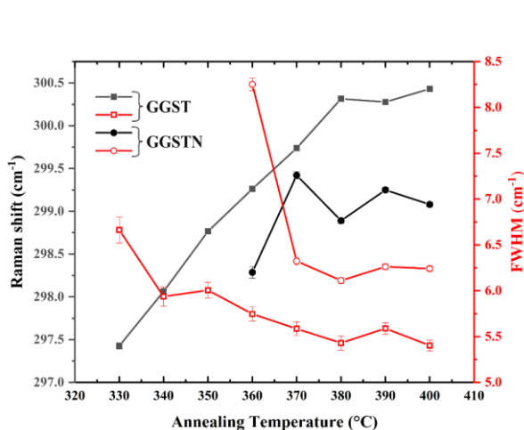
Fig. 4.7. Raman shift and FWHM behavior of the c-Ge peak for GGST and GGSTN examined with increasing annealing temperature
