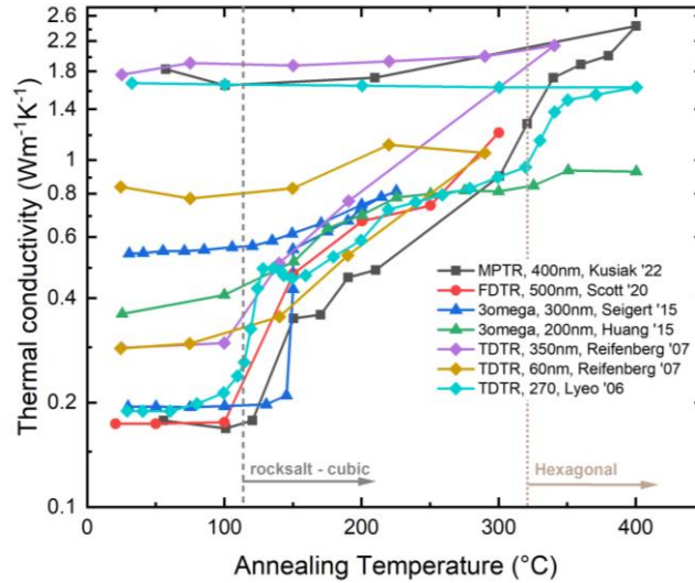
Fig 2.7 Temperature dependent thermal conductivity data collected from various articles to present a comparison of characterization techniques and thickness dependence, with details in the inset. Refs - Kusiak'22 [127], Scott '20 [128], Seigert '15 [119], Huang ' 15 [129], Reifenberg '07 [58], Lyeo '06 [113]
