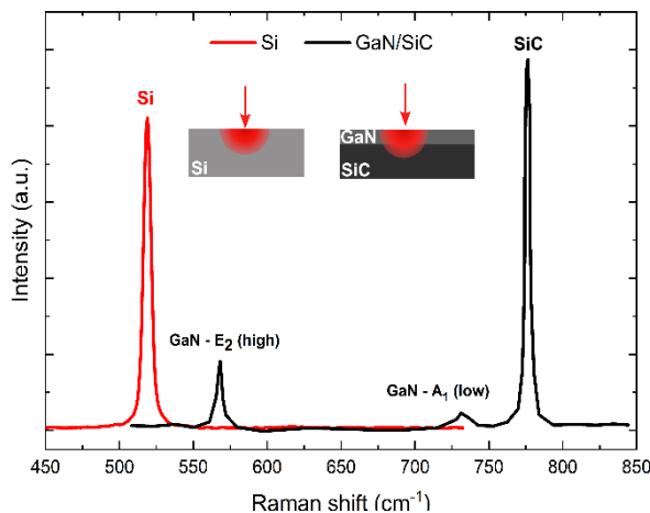
Fig 3.4 A typical Raman signal for a single substrate Si in red, and for GaN on SiC in black consisting of apparent Raman scattering peaks from phonon mods of both GaN and SiC [166]
