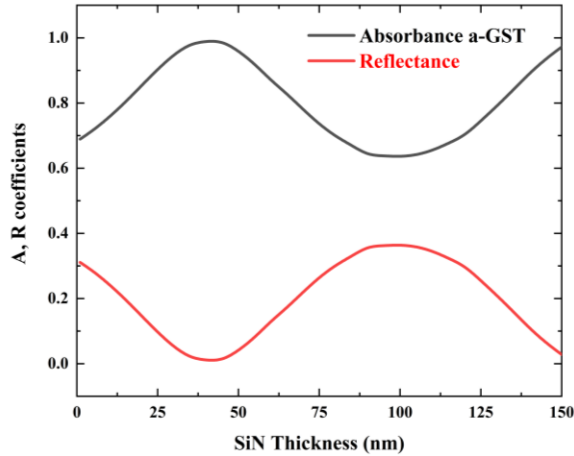
Fig 3.17 Absorption and reflection coefficients of 473.15 nm laser in a stack with varying SiN x thickness and GST thickness fixed at 200nm
