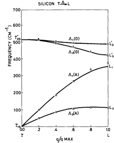
Fig 3.3 Dispersion curve for Si calculated along the symmetry line \Gamma -L [177]
