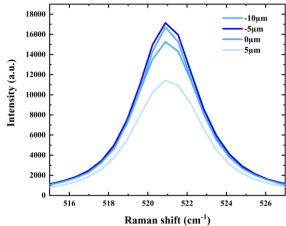
Fig 3.22 Change in intensity of acquired signal due to change of focus in z-direction. 0 \mu\text{m} focus is for the microscopic image whereas the laser focuses to maximum intensity at -5 \mu\text{m}
