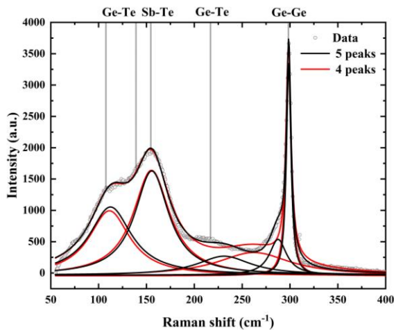
Fig. 5.1. Raman spectrum of c-GGSTN (grey circles) is fitted with 4 peaks (red) and 5 peaks (black) Lorentzian fitting procedure highlighting the difference in the fitted curve.
