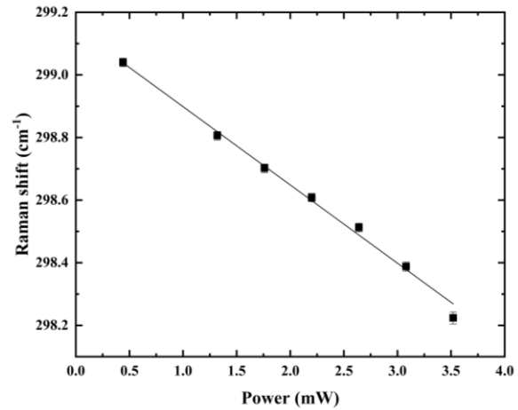
Fig 3.25 Power calibration curve of c-Ge phonon mode at 299 cm -1 for GGST
