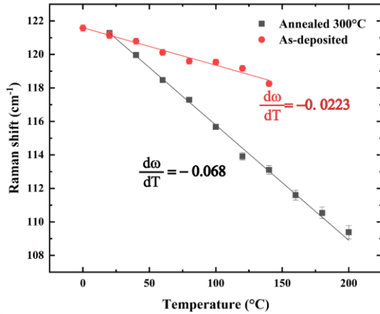
Fig. 5.21 Temperature calibration curve of as-deposited a-GeTe and annealed c-GeTe presented as Raman shift vs temperature. Significant difference in the sensitivity of the bonds is evident from the calibration coefficients
