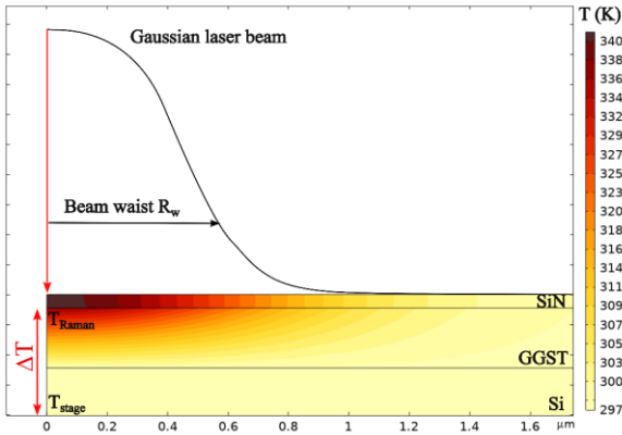
Fig 3.26 Schematic of FEM in COMSOL. Thin film stack with an incident Gaussian laser, \Delta T presents the local temperature difference between hotspot ( T_{Raman} ) and stage temperature ( T_{stage} ) due to incident laser
