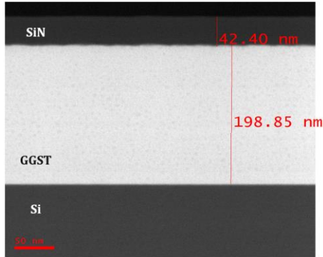
Fig. 4.3. TEM cut of the GGST deposited on a Si substrate and capped with a SiN layer
