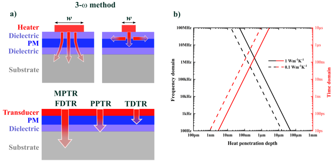
Fig 2.10 a) A schematic representation of different characterization techniques with red arrows indicating the investigated heat penetration depth. b) A map detailing the heat penetration depth of laser for characterization of 1 and 0.1 Wm -1 K -1 material depending on frequency domain or time domain technique
