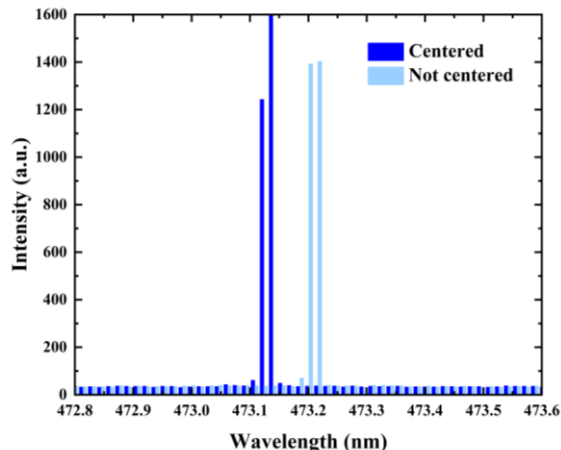
Fig 3.20 Schematic comparing the position of 473.12 nm laser for centered and not centered spectrometer.
