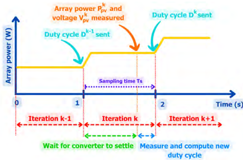
Figure 2.34: Time diagram showing the power evolution of the PV array when MPPT is active.
