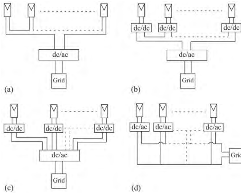
Figure 3.2: Distributed MPPT architectures: the conventional central inverter architecture (a), series-connected DC-DC to a central inverter (b), parallel-connected DC-DC to a central inverter (c), and micro-inverters (d). Figure extracted from [79].
