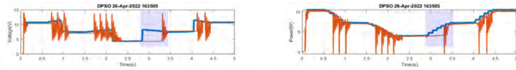
Figure 3.17: An example of where the irradiance perturbation detection mechanism failed in our tests with DPSO. On the left is the voltage of the array during experiment in orange and the expected voltage at GMPP in blue. On the right is the power of the array during experiment in orange and the expected power at GMPP in blue. We highlighted the region where the GMPP suddenly jump to another voltage operating point and optimal power is changing but the algorithm did not catch the variation at its current operating point.
