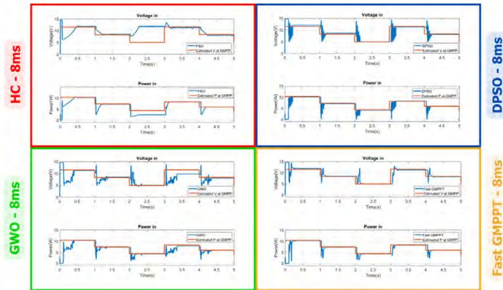
Figure 3.29: Sequence of irradiance steps results of four algorithms in experiment : HC, DSPO, GWO and fast GMPPT. The sampling time are given to put each algorithm's response time in perspective.
