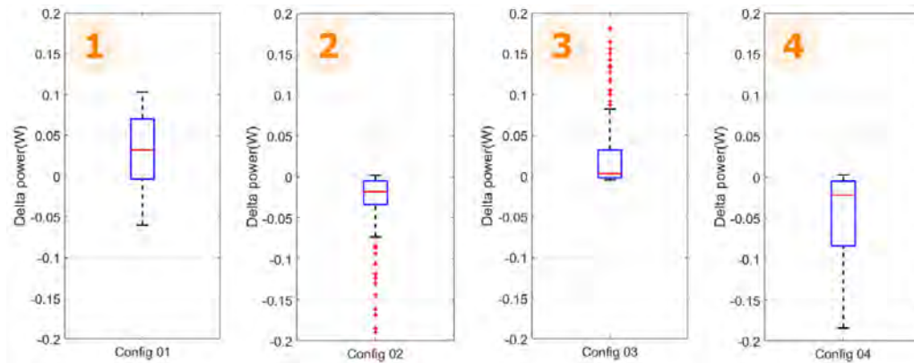
Figure 2.19: Dispersion of difference between the measured power minus the simulated power at each voltage of four solar panels.
