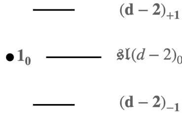
Figure 2.12: Decomposition of \mathfrak{sl}(d-1) under \mathfrak{sl}(d-2) \times \mathfrak{gl}(1) . The subscripts denote the R^+ charges which establish the vertical grading. At level 0 one finds the algebra of \mathfrak{sl}(d-2) \times \mathfrak{gl}(1) while level 1 and -1 contain an \mathfrak{sl}(d-2) vector and a dual vector, respectively [70].
