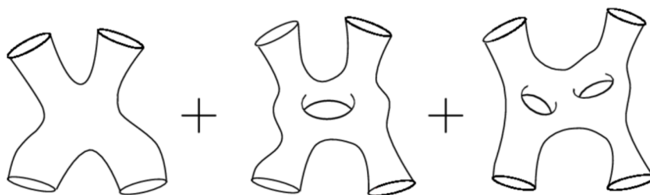
Figure 2.8: Examples of String Theory diagrams, each has a different genus [43].
