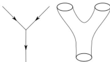
Figure 2.7: Lines in Feynman diagrams (left) are replaced by tubes on the String Theories scattering amplitude diagrams.
