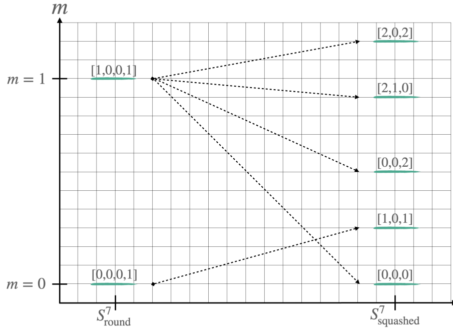
Figure 3.11: Schematic representation of the space invader scenario for the first two levels of the gravitini. All massless fields in the [0, 0, 0, 1] representation on S^7_{\text{round}} become massive on S^7_{\text{squashed}} and one massive field in [1, 0, 0, 1] at \ell = 1 on S^7_{\text{round}} becomes massless on S^7_{\text{squashed}} .
