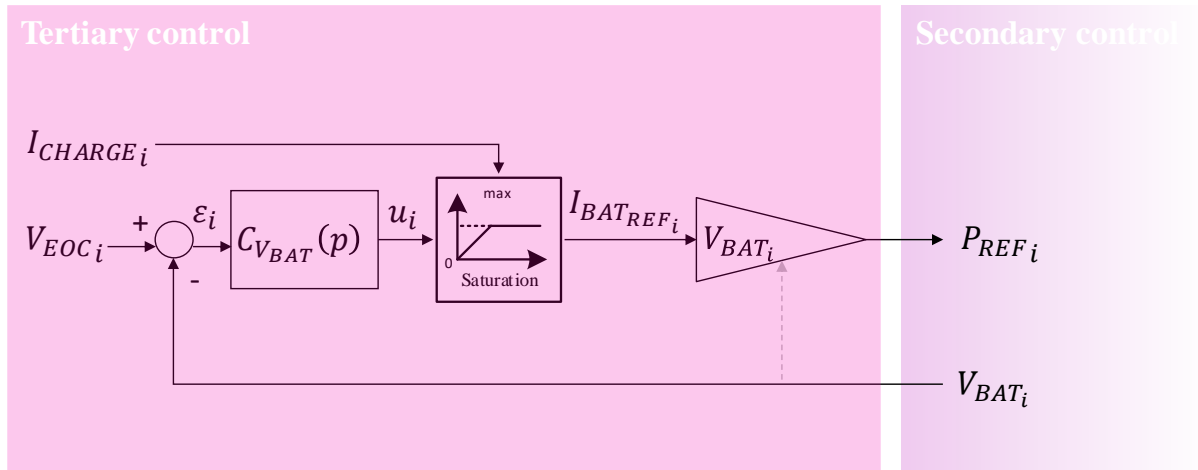
Figure 6.13 – Individual battery charge regulation loop on battery voltage.
