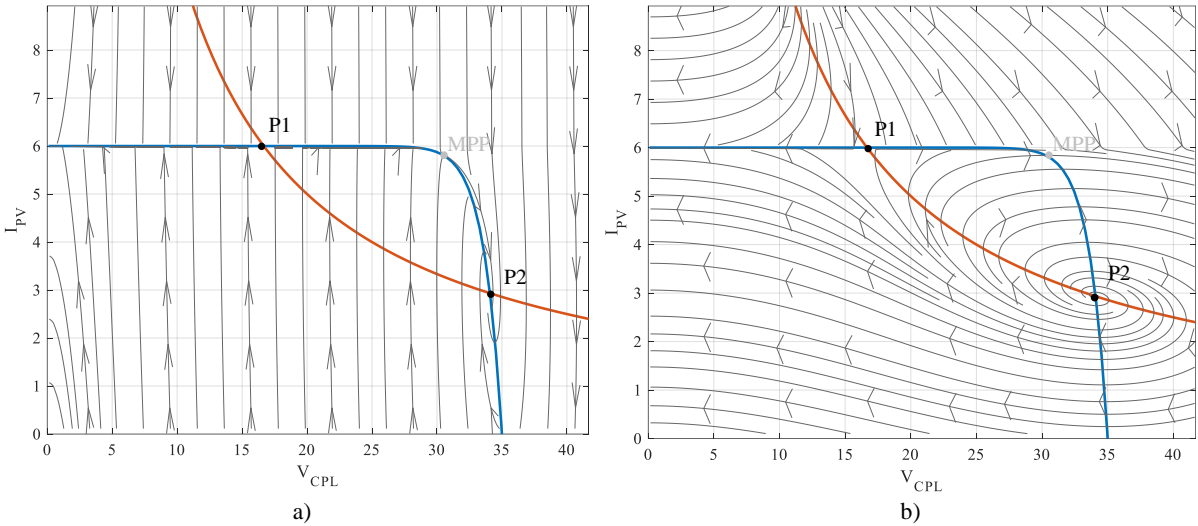
Figure 3.8 – State-plane trajectories in two configurations: (a) P2 is a stable node ( C = 380\mu F, L = 10\mu H ). (b) P2 is unstable ( C = 380\mu F, L = 2mH ).
