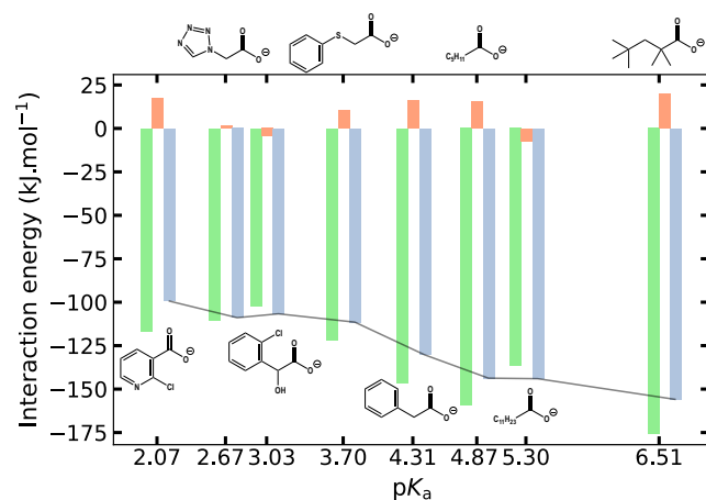
Figure 7 Comparison of the — electrostatic, — dispersion and — total interactions between all the ILs (ranked following the basicity of the carboxylate anion) and 1 SO 2 molecule. The solid line is a guideline to show the variation of the electrostatic interaction energy as a function of the pK a of the conjugated carboxylic acid in water.
