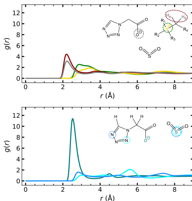
Figure 6. Site-site radial distribution functions, g(r) , calculated at 343 K in [P_{4,4,4,4}][TetrazC_1COO] . (Top) yellow line, P^+ , and gray line, H_\alpha of the cation in the presence of SO_2 , and green line, P^+ , and red line, H_\alpha of the cation around the carboxylate head O_{COO^-} the anion without gas. (Bottom) S_{SO_2} around green line, O_{COO^-} , light blue line, N2, and dark blue line, N4.
