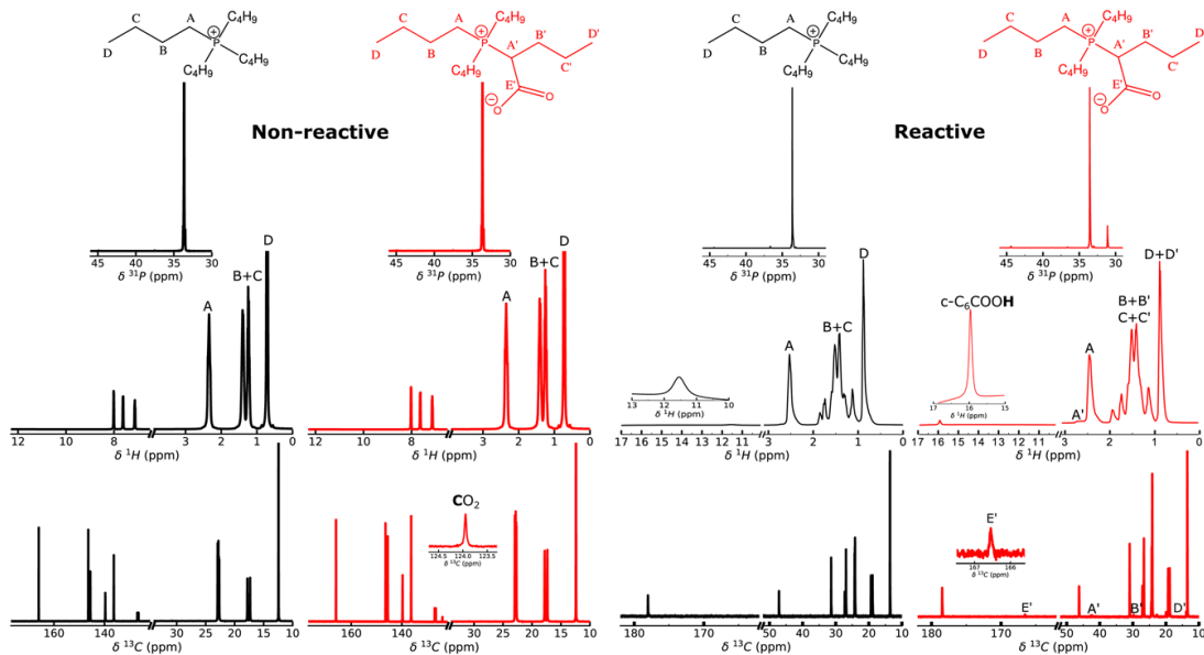
Fig. 3 ^{13}\text{C} , ^1\text{H} and ^{31}\text{P} NMR spectra of (left) [\text{P}_{4,4,4,4}][2\text{-ClPyCOO}] and (right) [\text{P}_{4,4,4,4}][\text{c-C}_6\text{COO}] before (—) and after (—) \text{CO}_2 absorption at 343 K. For the sake of clarity, only the signals related to the cation and the newly formed zwitterion have been highlighted here.
