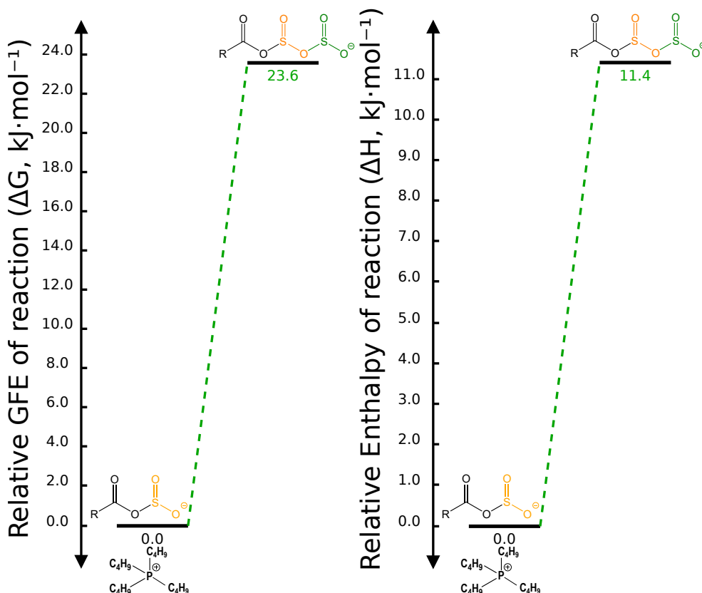
Figure S26 – Relative GFE and Enthalpy of the reactions leading to the chemical capture of a second \text{SO}_2 with a 1:1 stoichiometry ( \text{IL}:\text{SO}_2 ) in [\text{P}_{4,4,4,4}][\text{TetrazC}_1\text{COO}-\text{SO}_2] at 343 K.
