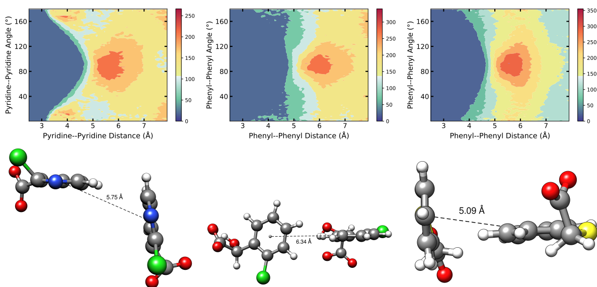
Figure S10 – CDFs of the angle between (left) two adjacent pyridine rings in [P_{4,4,4,4}][2-\text{CIPyCOO}] , two adjacent phenyl rings (middle) in [P_{4,4,4,4}][2-\text{CIPhC}_1\text{OHCOO}] and (right) in [P_{4,4,4,4}][\text{PhSC}_1\text{COO}] as a function of the RDF between their center of mass at 343 K. (Bottom) Snapshots from the molecular simulation box showing the most probable spatial configuration of two neighbour anions.
