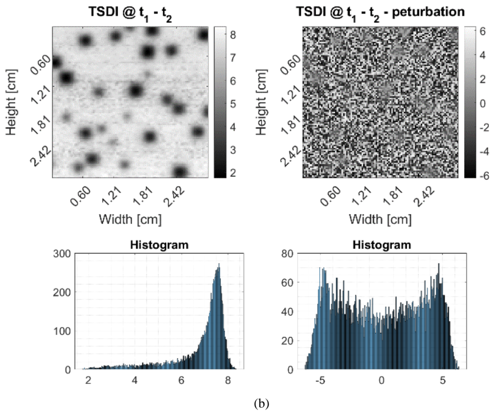
Figure 2-7. Time slices difference images in ideal and noisy context: (a) between maximum peak and first reflection; (b) between first and second reflection;
