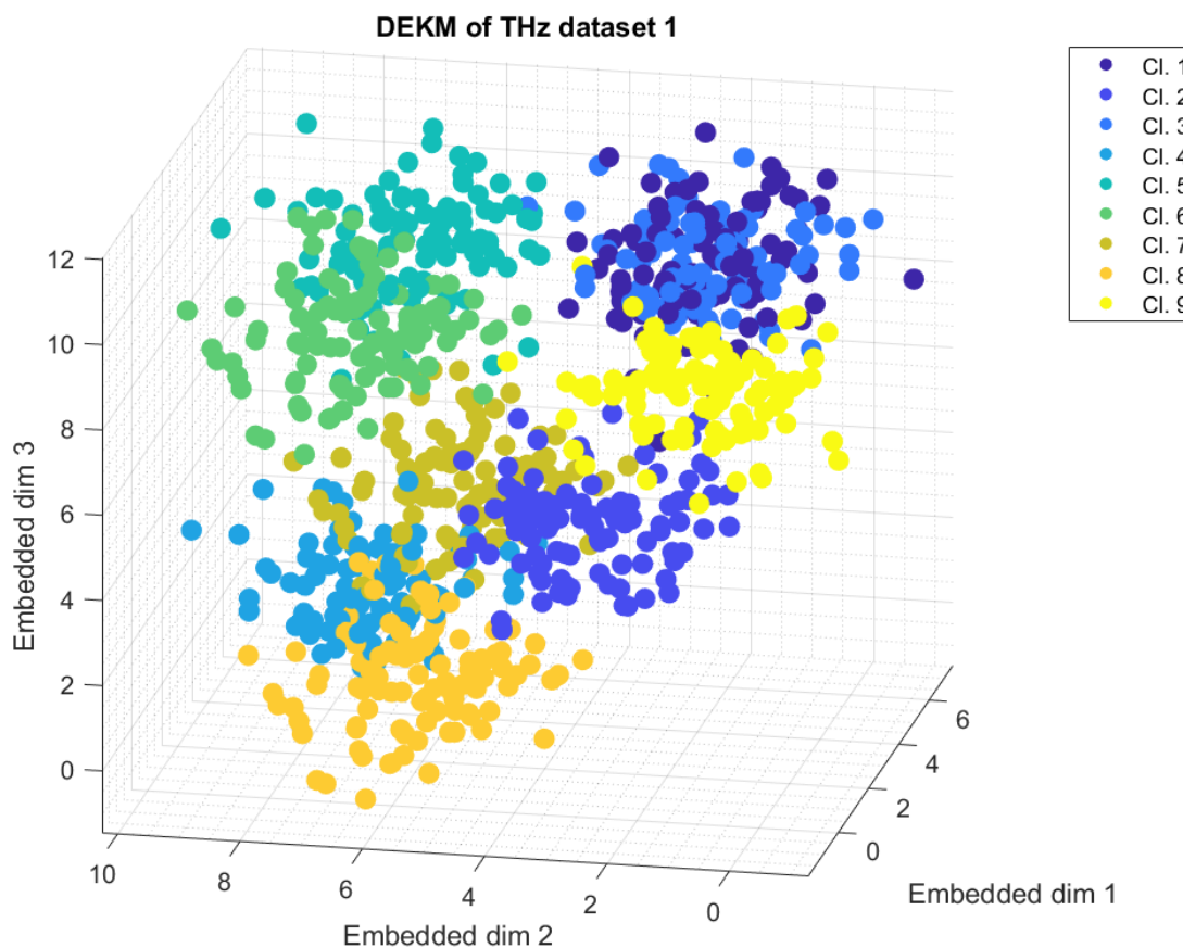
Figure 5-18. DEKM clusters
