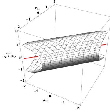
Figure 1.4: Tri-component representation of threshold surface of 2D Von Mises criterion for \sigma_{lim} = 1 .
