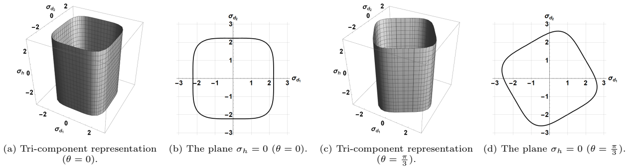
Figure 3.4: The TW4's surface with only \|\mathbb{E}^{8,4}\| = 0.3, \alpha^{8,4} = 0.8 . The surface is \mathcal{G}_S^{3D} = D_4 \otimes Z_2^c
