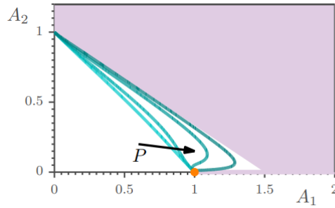
Figure 4.10: The boundaries of the relaxed feasible domain of the bar-truss problem with respect to a varying parameter [186].
