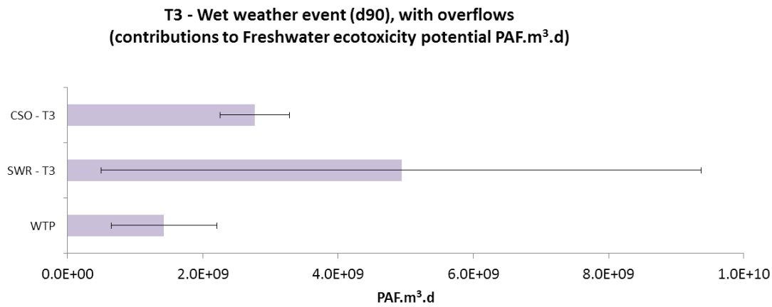
Figure S12. Contributions to the Freshwater ecotoxicity impacts (PAF.m 3 .d) of urban dry- and wet-weather flows at event scale (d90)
