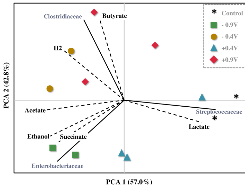
Fig. 4-3: Principal component analysis (PCA) based on microbial population distribution
