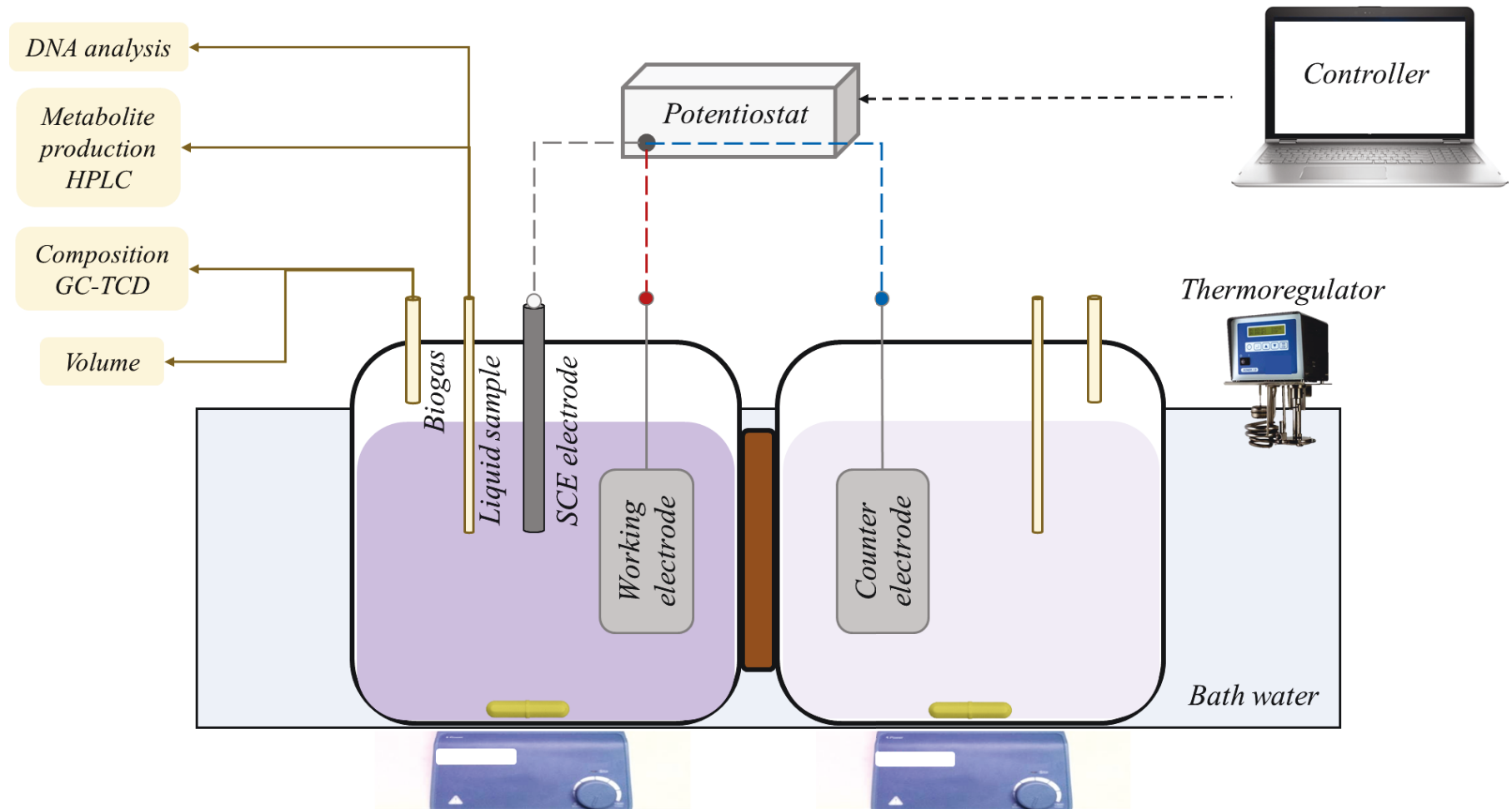
Fig. 2-3: Schematic diagram of experimental start-up for electro-fermentation tests performed in dual-chamber reactors
