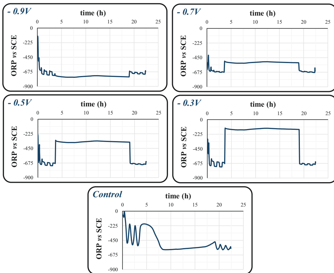
Fig. 3-8: ORP measurement in the fermentation bulk during electro-fermentation tests at different potential applied on the working electrode using single chamber reactors
