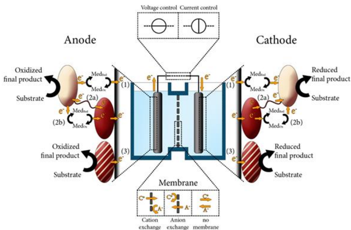
Fig. 1-6: Process configurations of electro-fermentation system including possible interactions between electrode and fermentation medium
