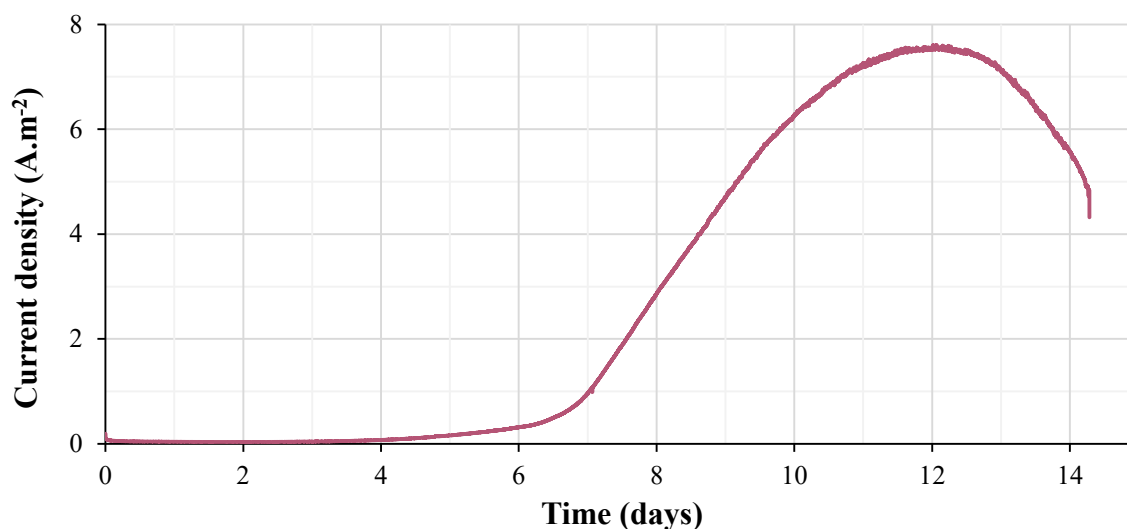
Fig. 2-4: Typical curve of current production during electrode colonization by G. sulfurreducens
