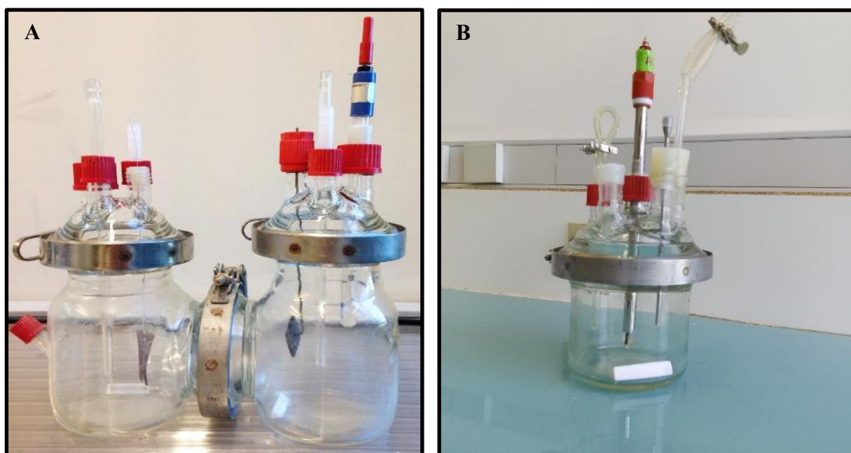
Fig. 2-1: Referential image showing reactors design used during this thesis
