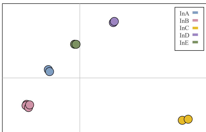
Fig. 5-11: Non-metric multidimensional scaling (NMDS) performed with Bray Curtis Similarity index from inoculum data.
