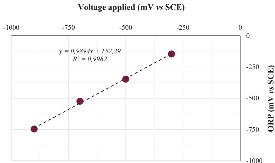
Fig. 3-9: Linear correlation between ORP measured in fermentation bulk and potential applied at working electrode
