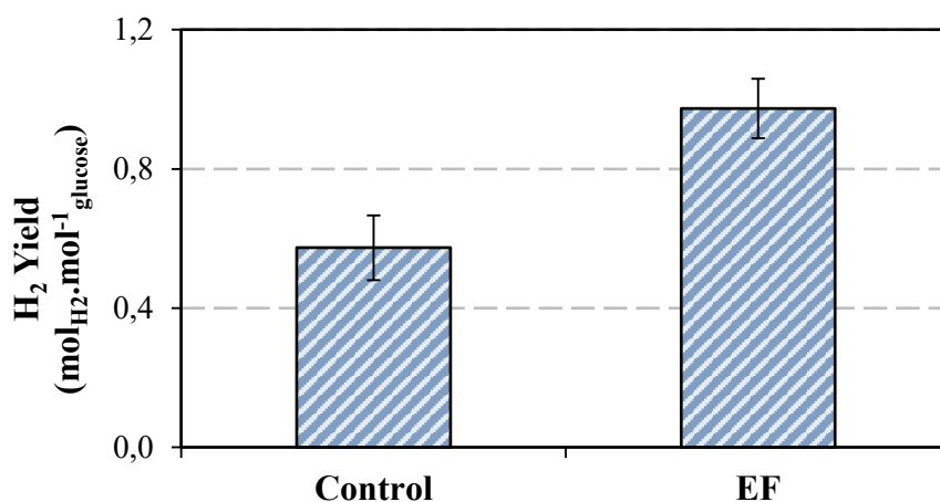
Fig. 3-2: Hydrogen yield observed in fermentation control and electro-fermentation tests using single chamber reactors and Pt-Pt electrodes.
