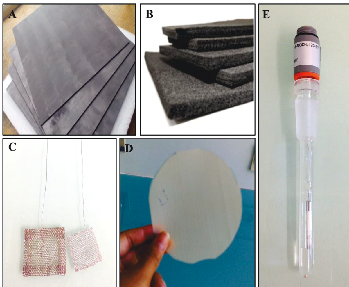
Fig. 2-2: Materials used to equip electro-fermentation reactors in this thesis
