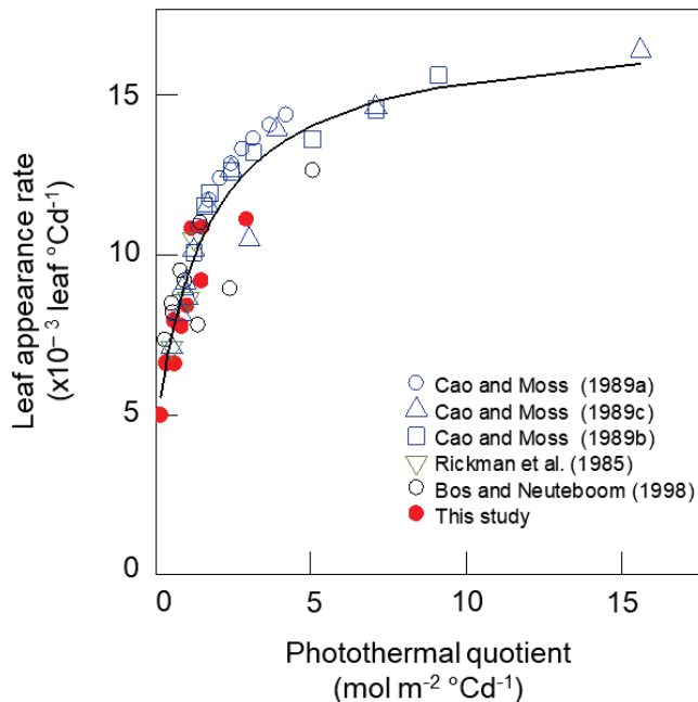
Figure 1.4. Relationship between leaf appearance rate and photothermal quotient for several wheat cultivars grown in controlled conditions with different combinations of temperature, irradiance, and photoperiod. Closed symbols are all treatments from experiment 1 to 3 at ambient air CO 2 concentration (Table 1.1). Open symbols are data from the literature (Supplementary Table S1.2), solid line is Eq. 1.4 fitted to all data points ( LAR = 0.004996 [\pm 0.000731] + ((0.002364 [\pm 0.0007] - 0.04996 [\pm 0.000731]) \times PTQ) / (1.9807 [\pm 0.5803] + PTQ) ).
