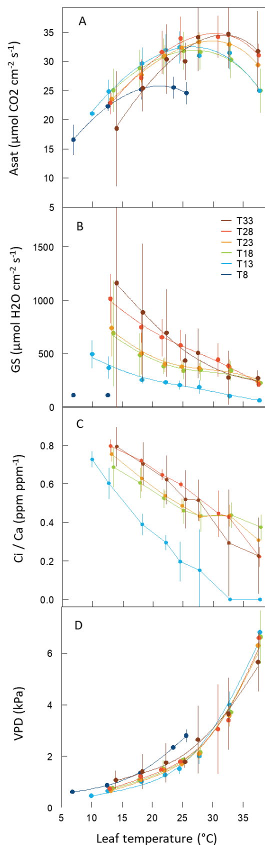
Figure 2.4. Effect of temperature on carbon assimilation, stomatal conductance, leaf intern CO 2 concentration ratio to external CO 2 concentration ( C_i/C_a ) and VPD at saturating light for the spring wheat cultivar Paragon grown in controlled conditions at different temperatures. (A) Leaf assimilation rate at saturating light ( A_{sat} ) versus T_{leaf} . (B) Stomatal conductance ( g_s ) versus T_{leaf} . (C) C_i to C_a ratio versus T_{leaf} . (D) VPD versus T_{leaf} . Treatments are detailed in Table 1 (Experiment 1). Lines in (A) are non-linear curves fitted to the data using Eq. 2. Values of the fitted parameters are given in Table 2.3. Lines in (B) and (D) are non-parametric spline curves fitted to the data. Measurements were taken on leaf 5 15°Cd to 50°Cd after its ligulation. Data are mean \pm 1 s.d. for n = 3 independent replicates.
