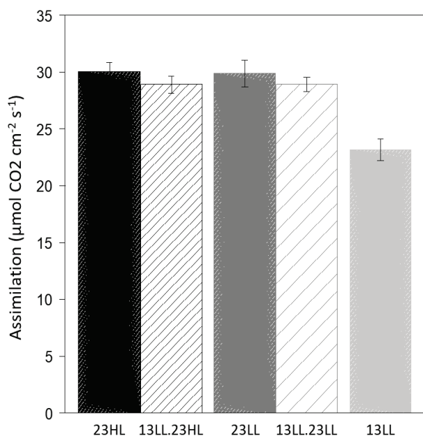
Figure 2.10. Leaf assimilation rate at saturating light ( A_{\text{sat}} ) for the spring wheat cultivar Paragon grown in controlled conditions with two irradiances (LL, 250 \mu\text{mol m}^{-2} \text{ s}^{-1} ; HM, 400 \mu\text{mol m}^{-2} \text{ s}^{-1} ) and two temperatures ( 13, 13/9^\circ\text{C} day/night; 23, 23/19^\circ\text{C} ). In treatments 23HL, 23LL and 13LL plants experienced the same growth conditions during the whole experiment while in treatments 13LL->23HL and 13LL->23LL plants were transferred from treatment 13LL to 23HL and from 13LL to 23LL at Haun stage 3.5. Treatment details are given in Table 1 (experiment 1). A_{\text{sat}} here is the average of A_{\text{sat}} measured several times on leaf 4 from its ligulation to the ligulation of leaf 5. Data are mean \pm 1 s.d. for n = 5 independent replicates
