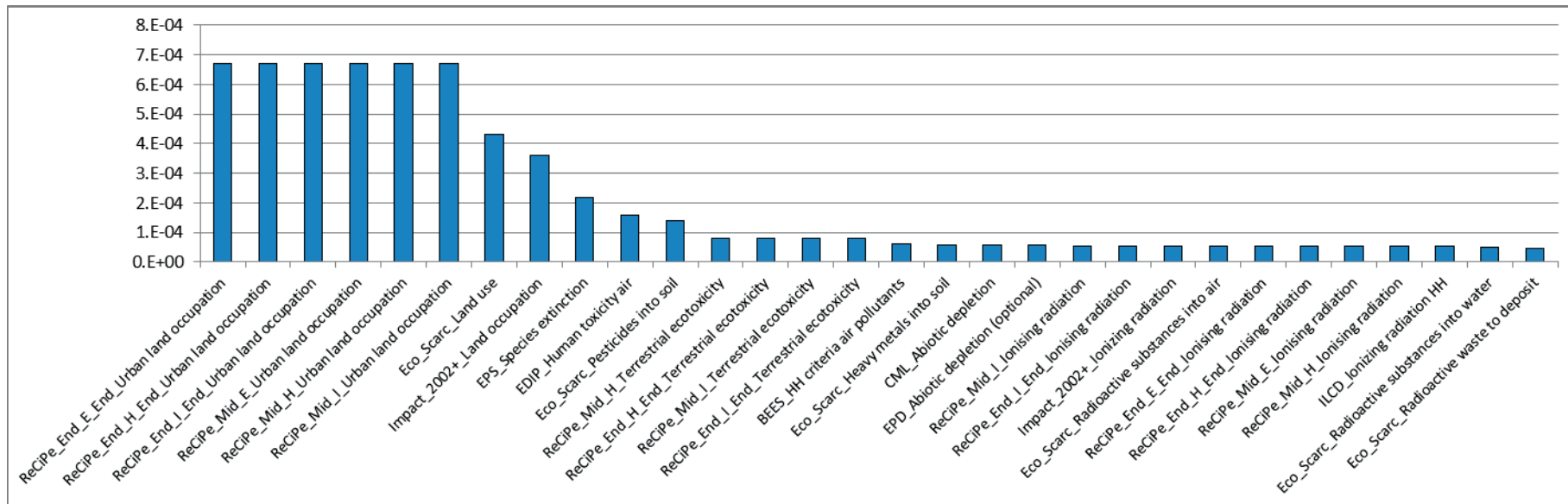
Figure S 22. Impact category RI screening for the global LCI
