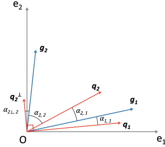
Figure 19. Illustration of the correlation issue and orthogonalization of q_2 regarding q_1
