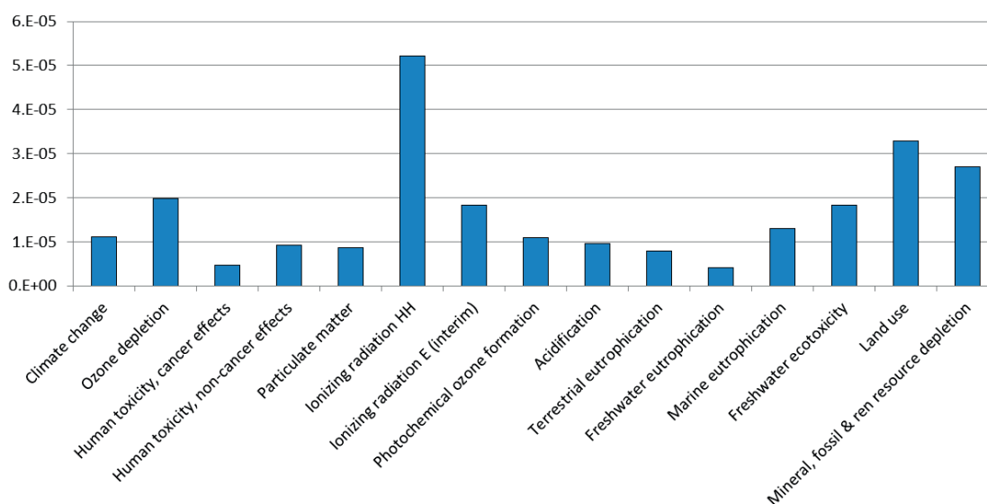
Figure 31. RI results of the entire LCI result
