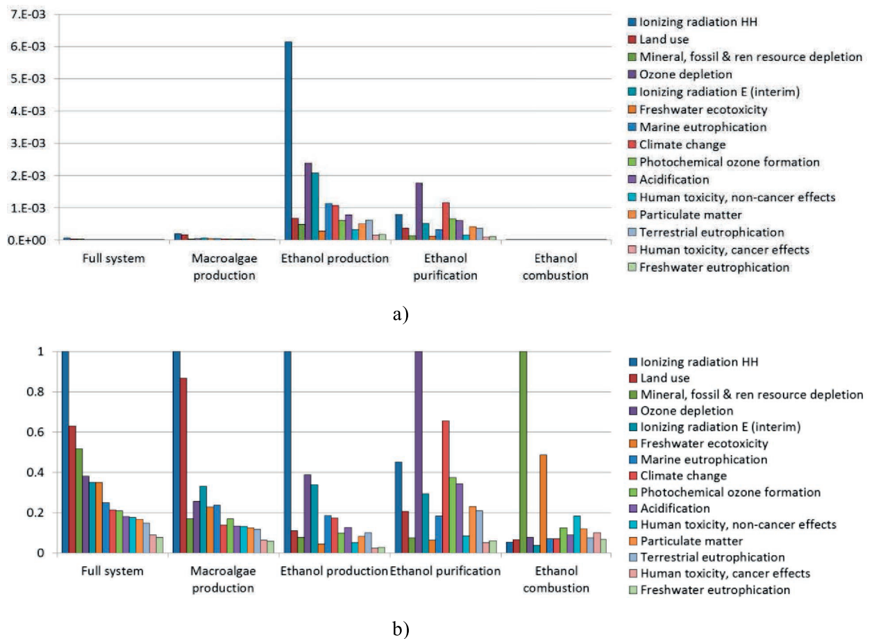
Figure 32. a) RI results of the ILCD impact categories (ranking by decreasing RIs of the whole LCI result). b) Normalization by the highest RI is applied for each LCI result due to the different magnitude.
