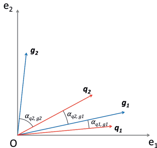
Figure 18. Representation of two standardized LCI result vectors g_1 and g_2 , two standardized impact category vectors q_1 and q_2 , and three of the angles used to measure RIs. The vector space is spanned by two basis vectors representing standardized elementary flows, such as CO_2 and NO_x .
