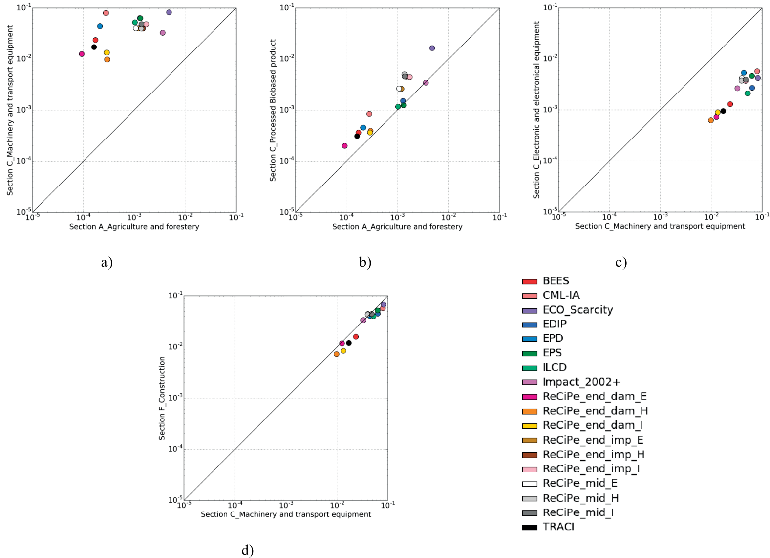
Figure 27. Comparison of the medians of LCIA method RIs
