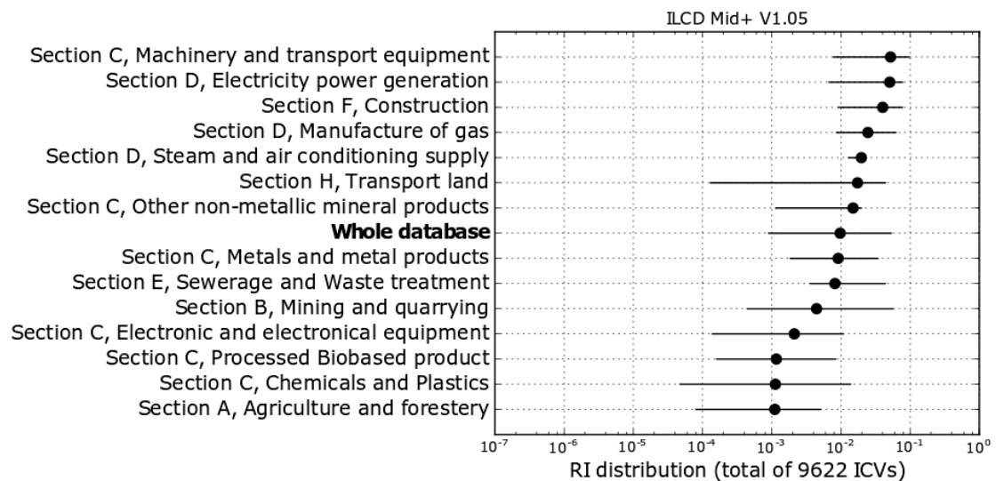
Figure 25. Global RI distributions for fields of activity and the whole database (black dots are the medians, first and third quartiles are represented by the bars. Fields of activity are classified according to their median)
