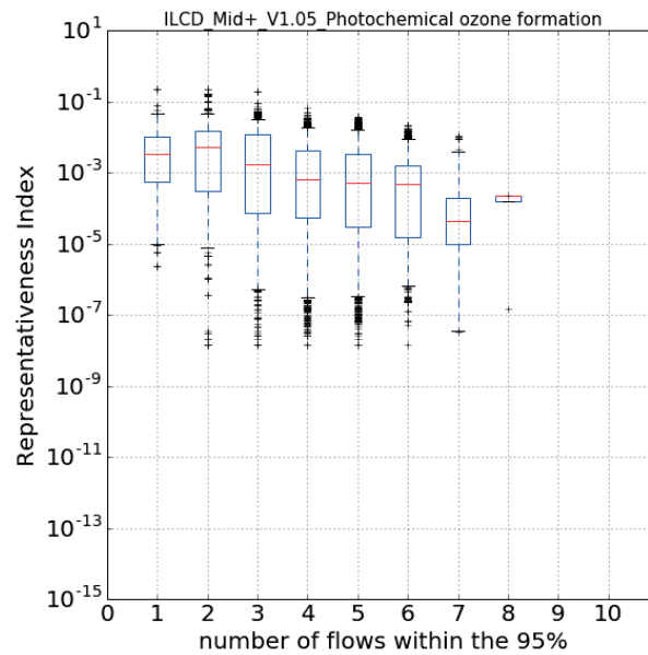
Figure 23. Boxplot of RI distributions according to the amount of dimensions per combination to represent 95% of the information.
