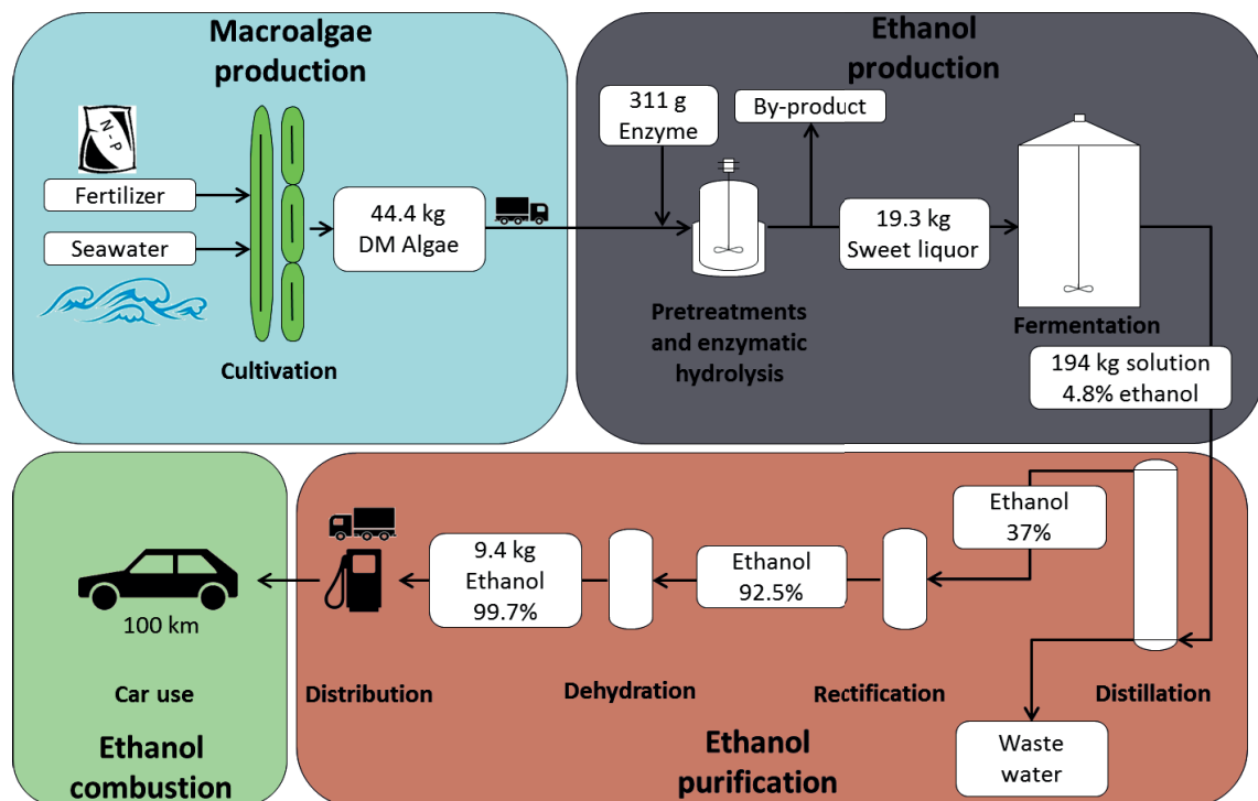
Figure 29. Schematic representation of the values chain
