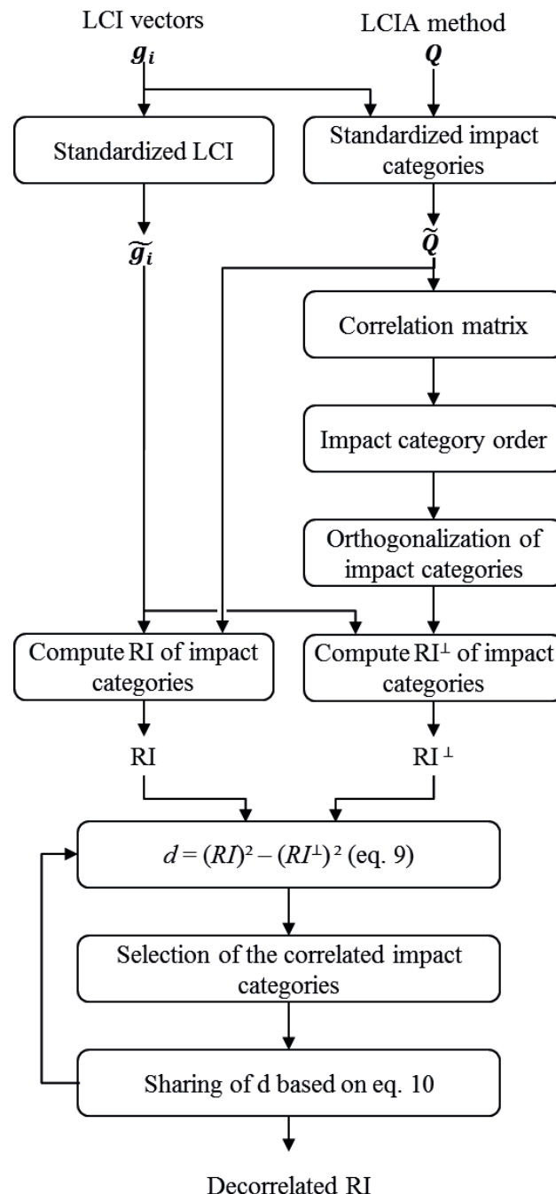
Figure 20. Schematics of the proposed algorithm
