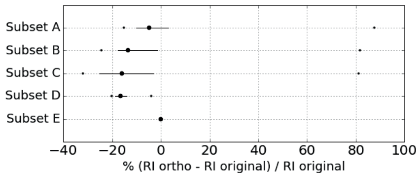
Figure 24. Analyses of the redistribution of RI values (figured are: the median (large black dot), the first and third quartiles (black segment), the 5% and 95% values (small black dot))
