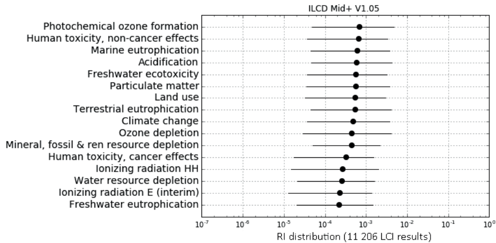
Figure 22. Range of RI values of the ILCD impact categories regarding the LCI results ofecoinvent. Figured are: the median (black dot), the first and third quartile (black segment). Impact categories are classified according to their median.
