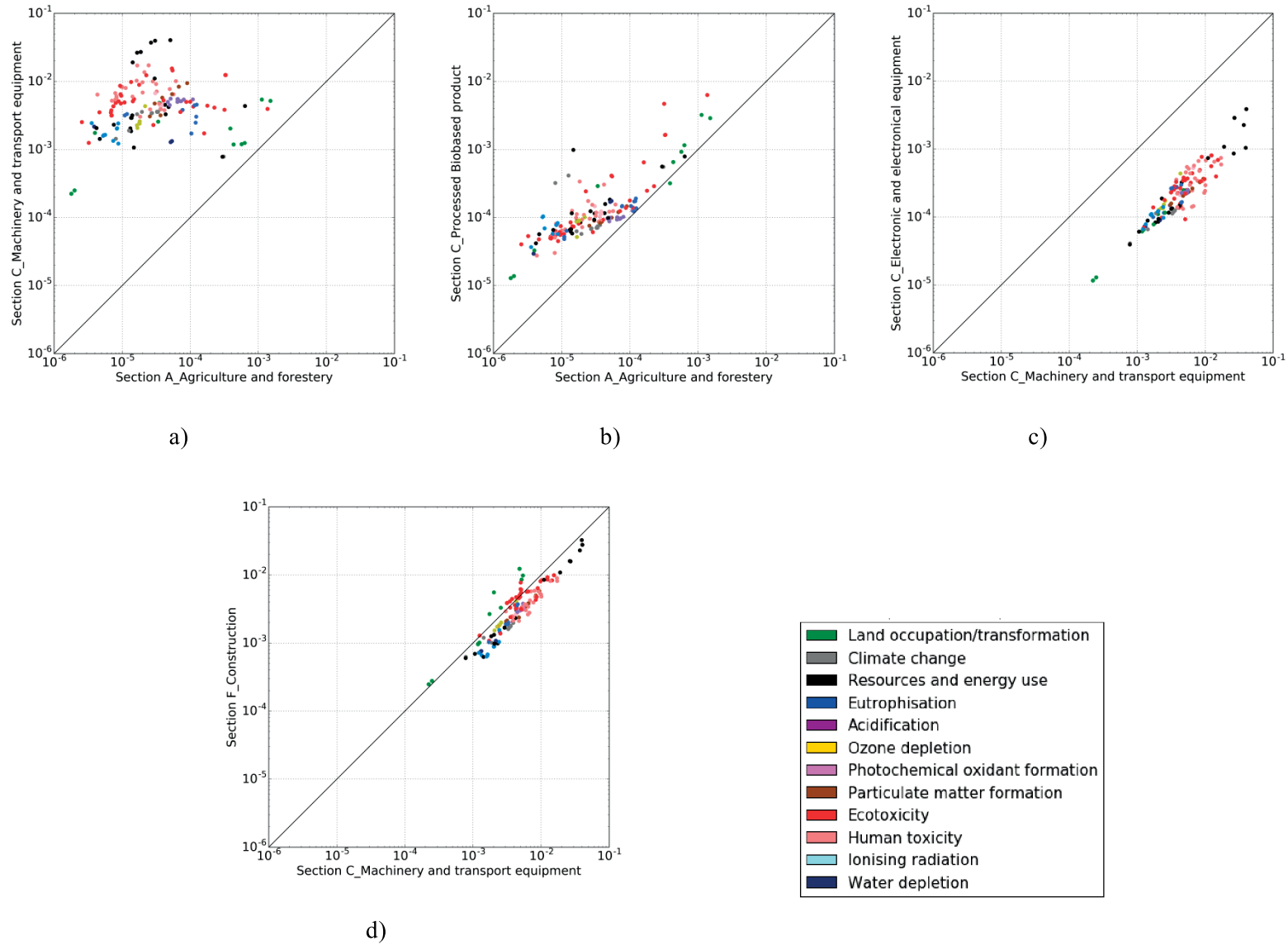
Figure 28. Comparison of the medians of impact category RIs
