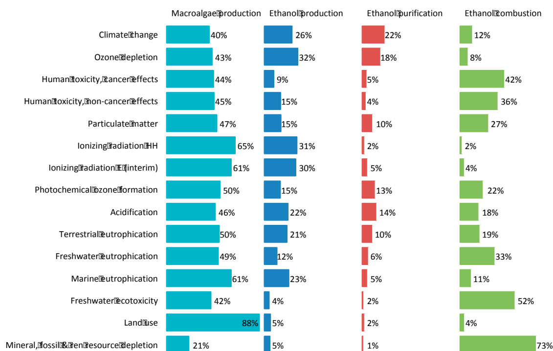
Figure 30. Process contribution analysis
