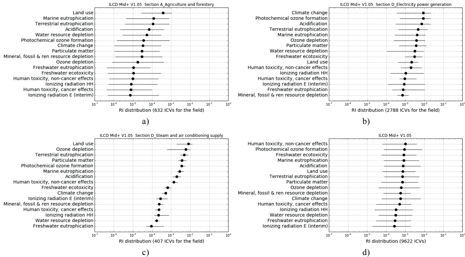
Figure 26. RI distributions for three fields of activity and the whole database (black dots are the medians, first and third quartiles are represented by the bars. Impact categories are classified according to their median)
