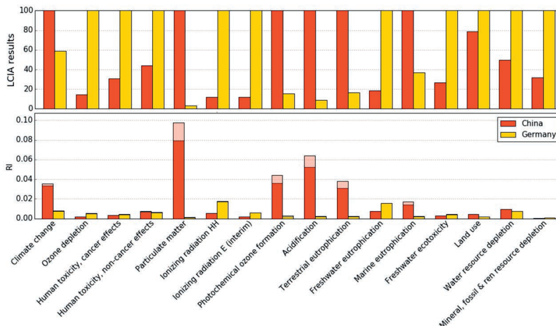
Figure 21. LCIA results and RIs of the LCI results of the Chinese and German electricity mixes from the ILCD method. Bright colours correspond to decorrelated RIs while pastels colours represent the differences between original and decorrelated RI.
