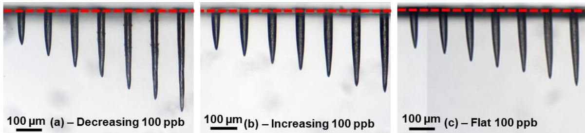
Figure 3.12. Microscope images of the holes drilled in sodalime with 100 pulses GHz-bursts of 200 \mu\text{J} with a number of bursts in a range from 200 to 800 for a decreasing burst shape (a), for an increasing burst shape (b) and for a flat burst shape (c) [136].
