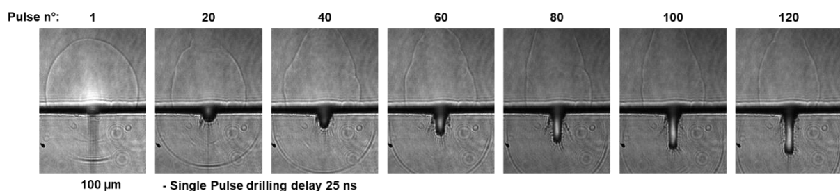
Figure 3.36. Pump-probe imaging in AF 32 in single pulse regime with pulses of 200 \mu J at a repetition rate of 200 Hz from pulse number 1 to 120 and a delay between the pump and the probe of 25 ns.
