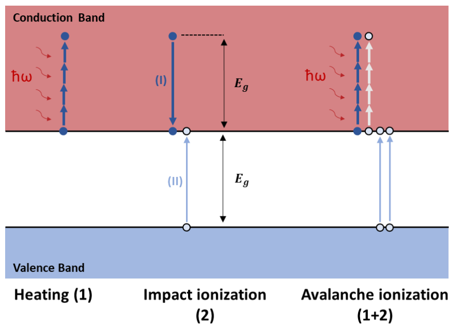
Figure 1.5. Schematic representation of the avalanche ionization. The first step is the heating of the free electrons through inverse Bremsstrahlung, the second is impact ionization leading to an exponential increase of the free carrier population ( 1 \rightarrow 2 \rightarrow 4 \rightarrow 8 \dots ).
