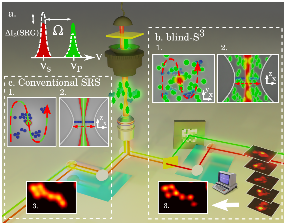
Figure 3.2: Principle of blind-S 3 . Schematic of the setup to achieve super resolution using the SRS process stimulated Raman Gain (SRG) (a) based on a single-pixel SIM scheme. Transverse (b1) and longitudinal (b2) planes of the scanning Stokes beam trajectory (red dash) over the stationary Raman-active specimen (blue) and structured Pump (green), in this case a speckle pattern. For every speckle realization, an SRS image is acquired forming an image stack that is passed to a SIM algorithm to reconstruct a super-resolved image (b3). (c) Conventional SRS, consisting in raster scanning co-propagating Pump and Stokes beams, is used as a control to demonstrate the increase in resolution when compared to standard imaging. Transverse (c1) and longitudinal (c2) planes of the Stokes and focused Pump beams (green and red dash) scanning trajectory over the stationary Raman-active specimen (blue).
