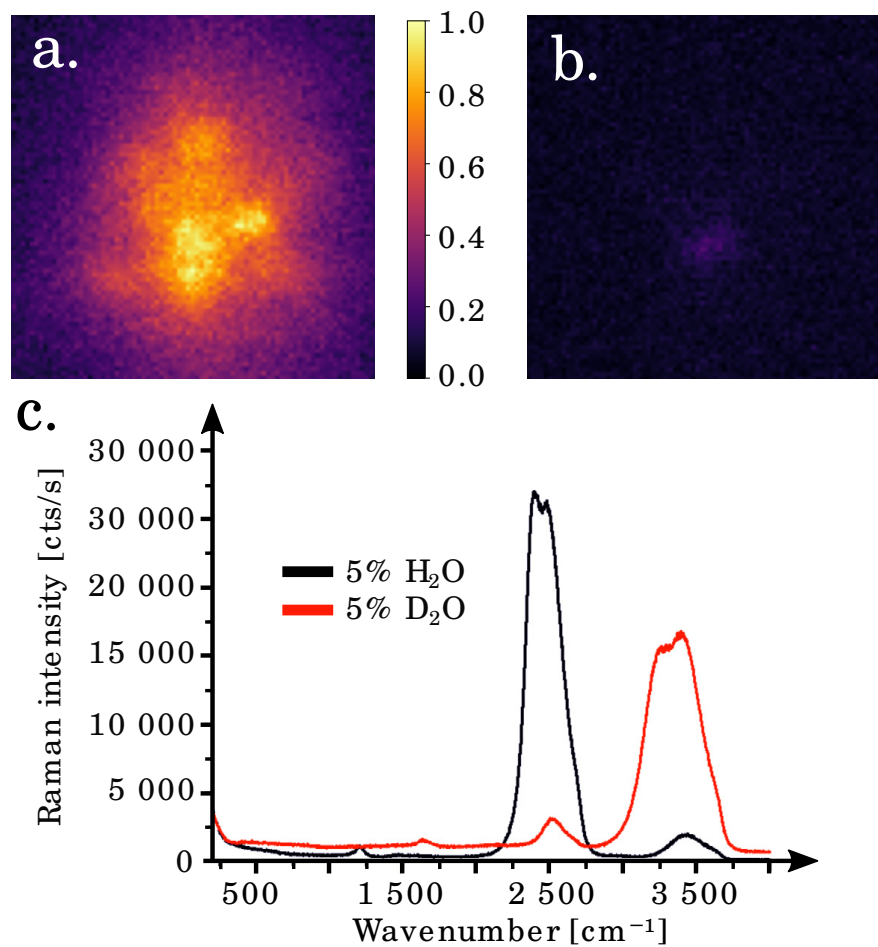
Figure 2.5: Comparison between water and heavy water SRS signal. a. Deionized water signal normalized from a speckle pattern. b. Heavy water signal from a speckle pattern. Normalized by the maximum of deionized water signal. c. Spontaneous Raman spectra of 5% H 2 O diluted in D 2 O (black line) and 5% D 2 O diluted in H 2 O (red line), adapted from [94]
