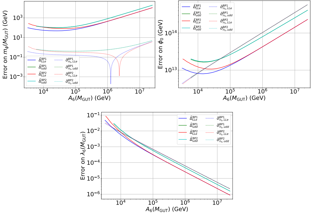
Figure 11.6: Systematic biases - \tilde{\Delta} 's as defined by Eq. 11.57 in solid lines - and statistical uncertainties - \tilde{\sigma} 's as defined by Eq. 11.58 in dotted lines - on the determination of the inflationary potential parameters as a function of A_6(M_{\text{GUT}}) : on the upper-left panel for m_\phi(M_{\text{GUT}}) , on the upper-right panel for \phi_0 , and on the lower panel for \lambda_6(M_{\text{GUT}}) . BP1 ( resp. BP2) is illustrated in dark blue ( resp. red) for an LLe inflaton, and in green ( resp. light blue) for udd .
