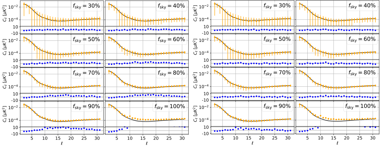
Figure 8.11: Preliminary! LEFT: EE auto QML power spectra (orange) and associated residuals (blue) for various sky fractions, RIGHT: cross QML spectra. They are based on the baseline complexity + \text{wn} + 1/f simulations, as compared with the input signal. The residuals in per cent are normalised by \sqrt{N_{\text{sim}}} = \sqrt{200} and compared to the \pm 1 grey contour that represents the statistical fluctuation range.
