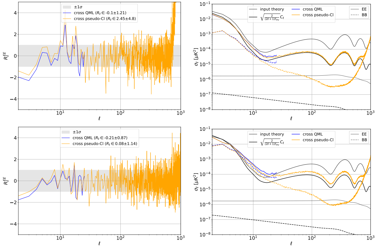
Figure 8.16: Preliminary! The two panels contain similar figures as Fig. 8.2 representing the biases and variances in the EE and BB estimates for QML and PCI, with 200 wn + 1/ f + d1s1 HILC simulations. The upper panels focus on the f_{\text{sky}} = 70\% setup, while the lower ones illustrate the f_{\text{sky}} = 30\% setup.
