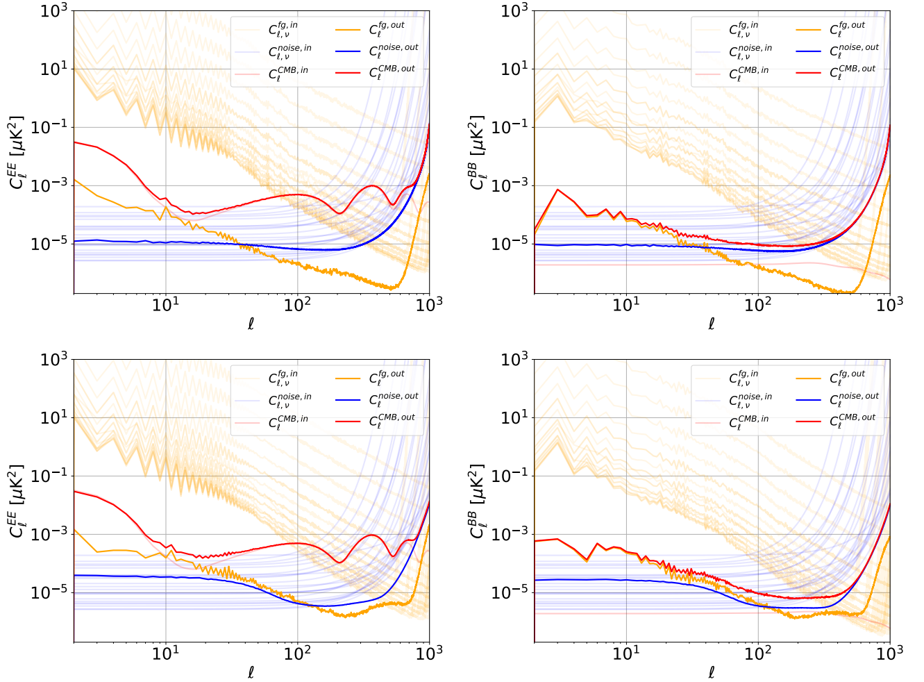
Figure 7.13: Preliminary! Summary figure for TOP-LEFT: EE TOP-RIGHT: BB . The clear curves represent the power spectra estimated from the full-sky HILC map, itself derived from the 22 input d1s1 maps (each corresponding to a LiteBIRD frequency channel). The spectra are coloured by component type: Galactic foregrounds in orange, noise in blue, CMB signal in red. The opaque curves represent the power spectra after HILC cleaning for the three components (associated with the same colours as before). BOTTOM: same with high-complexity foregrounds.
