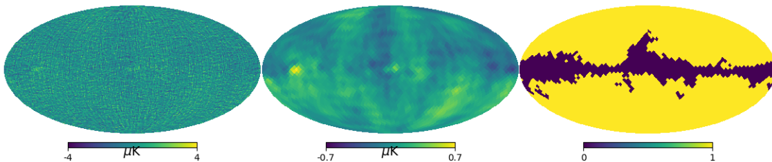
Figure 8.9: Preliminary! LEFT: particular simulation of a Q HILC map at N_{\text{side}} = 512 (wn1f + d1s1), MIDDLE same map downgraded to N_{\text{side}} = 16 (explanations in the text), RIGHT realistic binary mask we use to estimate the QML spectra.
