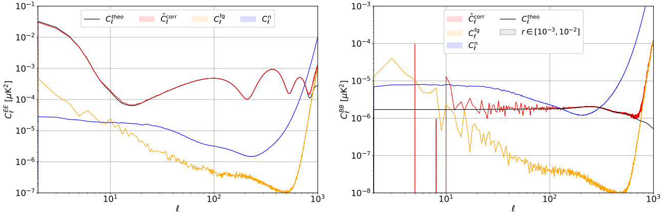
Figure 8.14: Preliminary! Pseudo power spectrum estimation averaged over 200 wnlf + baseline simulations, cleaned with HILC ( N_m = 400 , \sigma_{w_\ell} = 35 ), with an ideal mask. The theoretical spectrum is displayed in black curves, the noise-corrected output spectrum with the associated 68% region in red (see the core of the text), and the noise and the foreground residuals, respectively represented in orange and blue. LEFT: EE with f_{\text{sky}} = 90\% RIGHT: BB with f_{\text{sky}} = 50\% . The r \in [10^{-3}, 10^{-2}] theoretical region is displayed as a grey contour.
