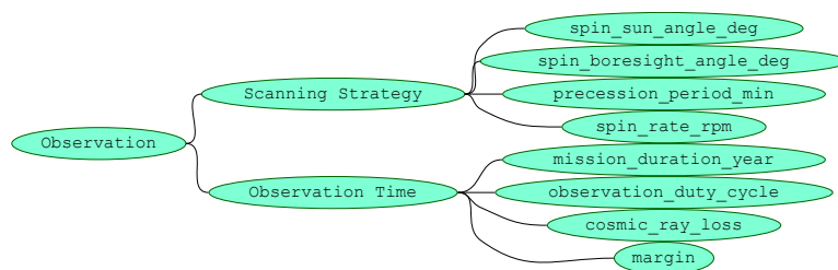
Figure 2.1: IMo tree architecture for the observation level.
