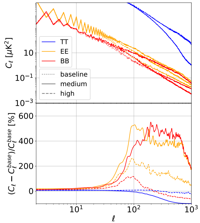
Figure 3.2: Refer to caption of Fig. III.2. This figure is similar but obtained for the H3-402 frequency channel observing at a central frequency of 402 GHz, a dust-dominated regime.
