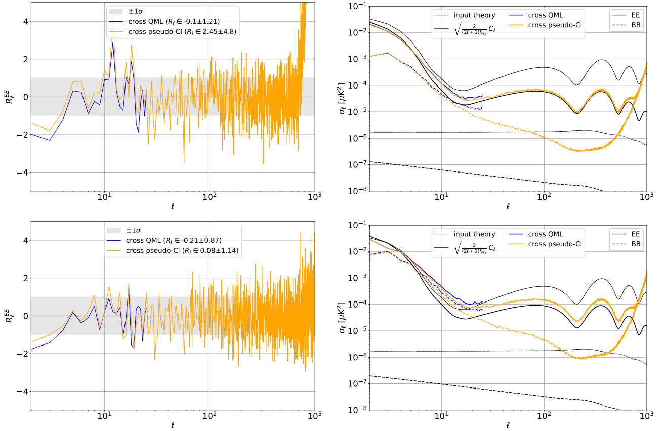
Figure 8.16: Preliminary! The two panels contain similar figures as Fig. 8.2 representing the biases and variances in the EE and BB estimates for QML and PCI, with 200 wn + 1/f + d1s1 HILC simulations. The upper panels focus on the f_{\text{sky}} = 70\% setup, while the lower ones illustrate the f_{\text{sky}} = 30\% setup.
