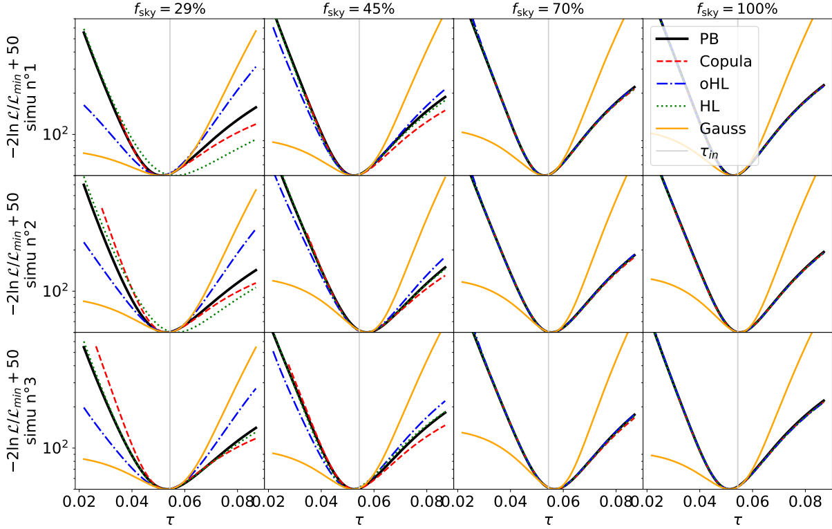
Figure 9.7: Shape of -2 \log -likelihood for three different realisations (from top to bottom) and for four different f_{\text{sky}} , 29%, 45%, 70%, 100% (from left to right). The black curve represents the reference (exact) \mathcal{L}_{\text{PB}} , \mathcal{L}_{\text{cop}} in dashed-red, \mathcal{L}_{\text{oHL}} in dashed-dotted-blue, \mathcal{L}_{\text{HL}} in dotted-green, \mathcal{L}_{\text{gauss}} in orange. The input \tau is represented by a vertical grey line. The minimum of the log-likelihood is fixed at 50. The setup is base input theory, low SNR regime, with auto QML spectra and empirical covariance matrix described in Sec. 9.3.1.1
