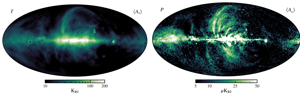
Figure 4.5: Synchrotron amplitude maps from Planck as obtained by the COMMANDER component separation. LEFT: total intensity map at 30 GHz, from [51], RIGHT: total polarisation map at 30 GHz, from [118].
