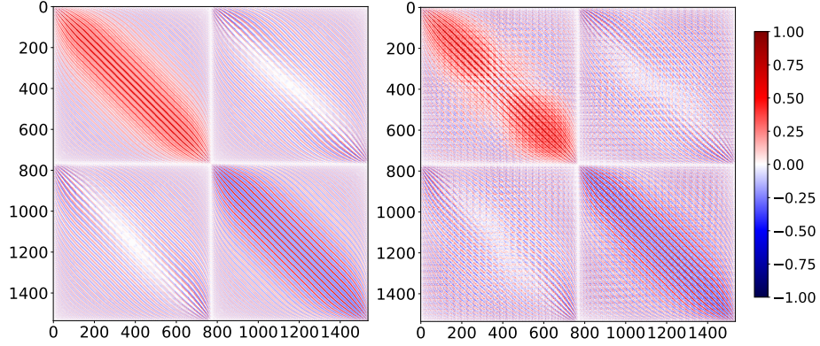
Figure 8.10: Preliminary! LEFT: Analytical signal covariance matrix \mathbf{S} from the simulation-input C_\ell , RIGHT: Empirical total covariance matrix \hat{\mathbf{M}} estimated on the \text{dls1} + \text{wn} + 1/f HILC-cleaned simulations, inaccurate and not invertible due to lack of statistics. Both are obtained for a full sky at N_{\text{side}} = 16 .
