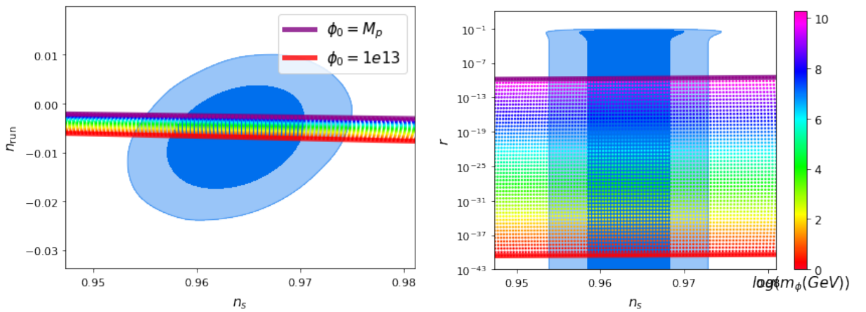
Figure 6.1: Predicted cosmological observables for potentials selected to produce A_s as currently measured by Planck, for a grid of \phi_0 and \alpha_s .
