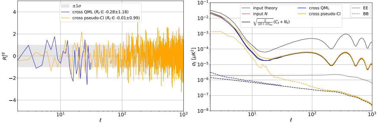
Figure 8.2: LEFT: Empirical normalised residuals, see Eq. 8.23, for the two EE cross power spectrum estimation methods (in blue cross QML, in orange, cross pseudo-Cl) as compared with the \pm 1\sigma region. For this particular set of realisations, we display in the legend the averages and standard deviations of the residuals for both methods, estimated over the \ell -range of the figure. RIGHT: standard deviation for the same methods (associated with the same colours), for EE (plain curves) and BB (dashed curves), as compared with the formula Eq. 2.49, which is an approximation to the theoretically optimal standard deviation. The empirical curves are estimated over 1000 simulations, which have been generated from the fiducial parameters of Tab. 4.1, with no foregrounds and high signal-to-noise regime (white noise with \sigma = 0.01 \mu\text{K}\cdot\text{arcmin} ), and an f_{\text{sky}} = 72\% mask. The noise curve (labelled in red) is below the y-axis range, at 8.5 \times 10^{-12} \mu\text{K}^2\cdot\text{rad}^2 .
