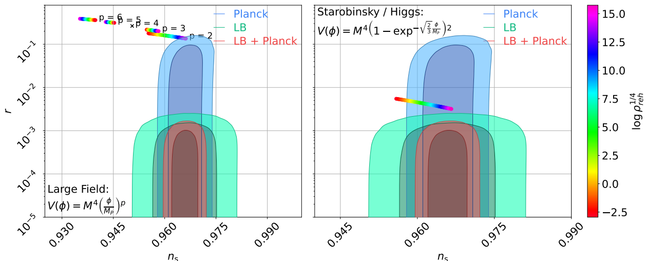
Figure 10.2: LEFT: LFI RIGHT: SHI ( p, \log_{10} \rho_{\text{reh}} ) grid of (n_s, r) predictions. \rho_{\text{reh}} is in \text{GeV}^4 . Fisher ellipses for mock Planck data and mock LiteBIRD data are superimposed, with fiducial \Lambda -CDM + r parameters given in Table 4.1 (and r_{\text{fid}} = 0 ).
