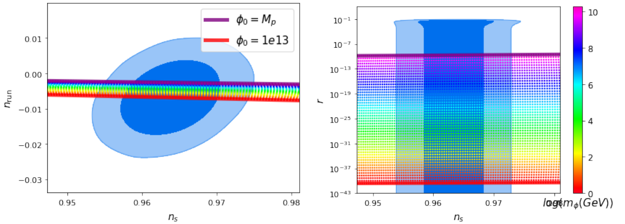
Figure 6.1: Predicted cosmological observables for potentials selected to produce A_s as currently measured by Planck, for a grid of \phi_0 and \alpha_s .
