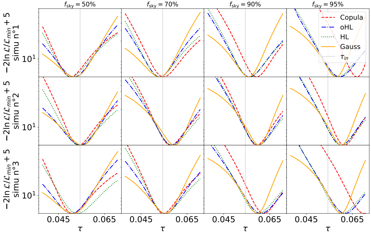
Figure 9.17: Preliminary! Shape of -2 \log\tau -likelihood for three different LiteBIRD \text{wn1f} + high-complexity-foreground realisations (from top to bottom) and for four different sky fractions, 50%, 70%, 90%, 95% (from left to right). \mathcal{L}_{\text{cop}} is represented in dashed-red, \mathcal{L}_{\text{oHL}} in dashed-dotted-blue, \mathcal{L}_{\text{HL}} in dotted-green, \mathcal{L}_{\text{gauss}} in orange. The input \tau is represented by a vertical grey line. For illustration purposes, the minimum log-likelihood is fixed to 5. the setup consists of cross pseudo-power spectra obtained from split HILC-cleaned maps. The covariance matrix is estimated from 200 simulations, and the likelihoods are corrected by Sellentin-Heavens prescription (for Gaussian, HL, oHL) or by the Hartlap factor (for copula). The pixel-based likelihood is not applicable to these unknown-covariance case.
