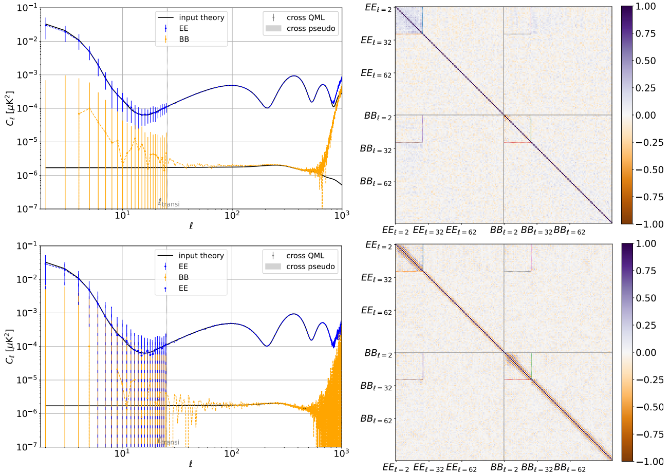
Figure 8.17: Preliminary! Same figures as Fig. 8.6 representing the hybrid spectra, with 200 w_n + 1/f + d1s1 HILC simulations, f_{\text{sky}}=70\% . The upper panels illustrate the f_{\text{sky}} = 70\% setup, while the ones illustrate the f_{\text{sky}} = 30\% setup.
