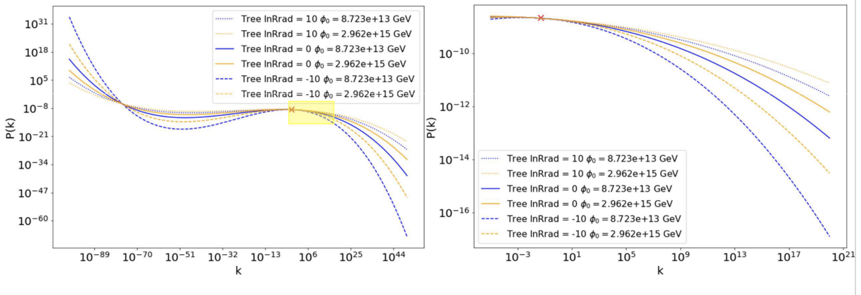
Figure 6.2: Full primordial power spectrum computed at third order in slow-roll on a wide wavelength range for various tree-level eMSSM-inflation configurations. k is given in \text{Mpc}^{-1} and the typical CMB observable window lies between k = 0.0002 and k = 0.2 \text{ Mpc}^{-1} .
