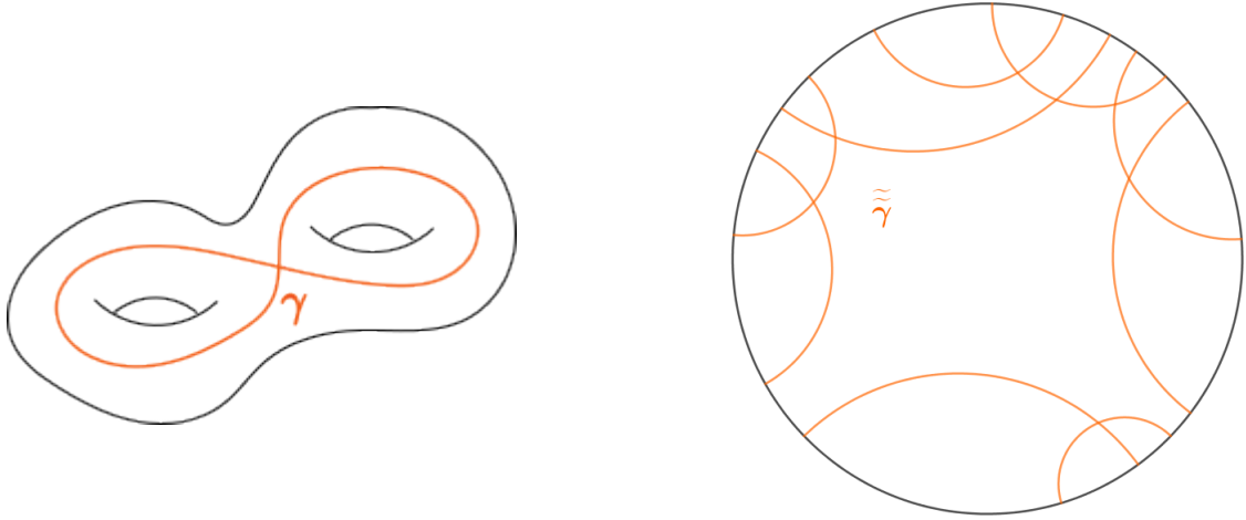
Figure 1.9 – Total lift of a curve to the universal cover
