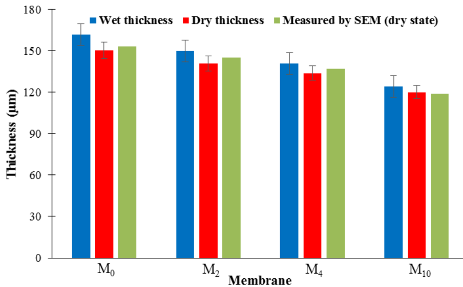
Figure 4.4. Wet and dry thickness of PA6 porous membranes.
