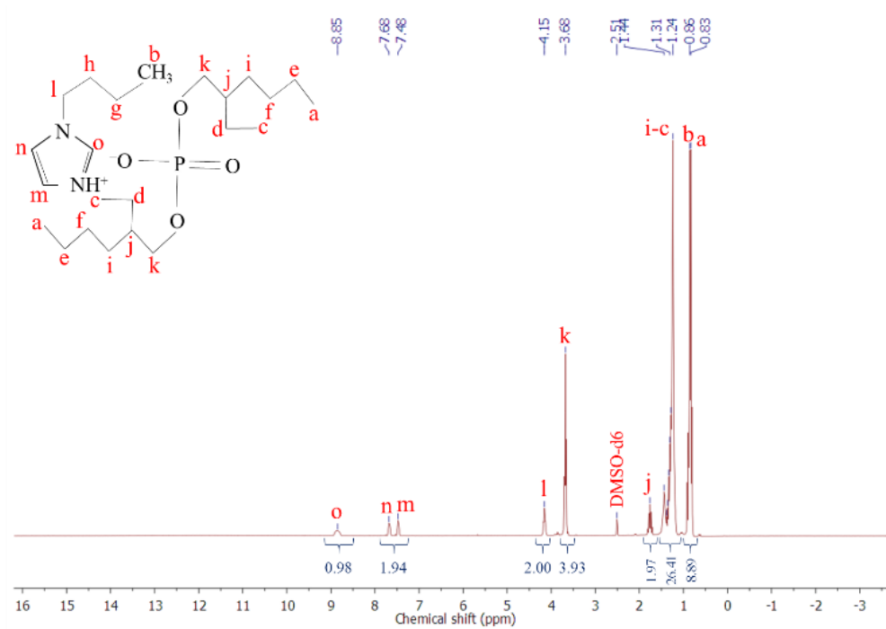
Figure S9. ^1\text{H} NMR spectrum of [BIM][EHPH].
