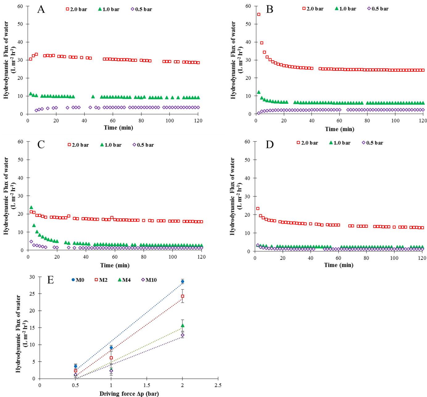
Figure 4.10. Hydrodynamic water flux at different operating pressures of PA6 membranes: A) M_0 ; B) M_2 ; C) M_4 ; D) M_{10} ; and E) as a function of driving force.
