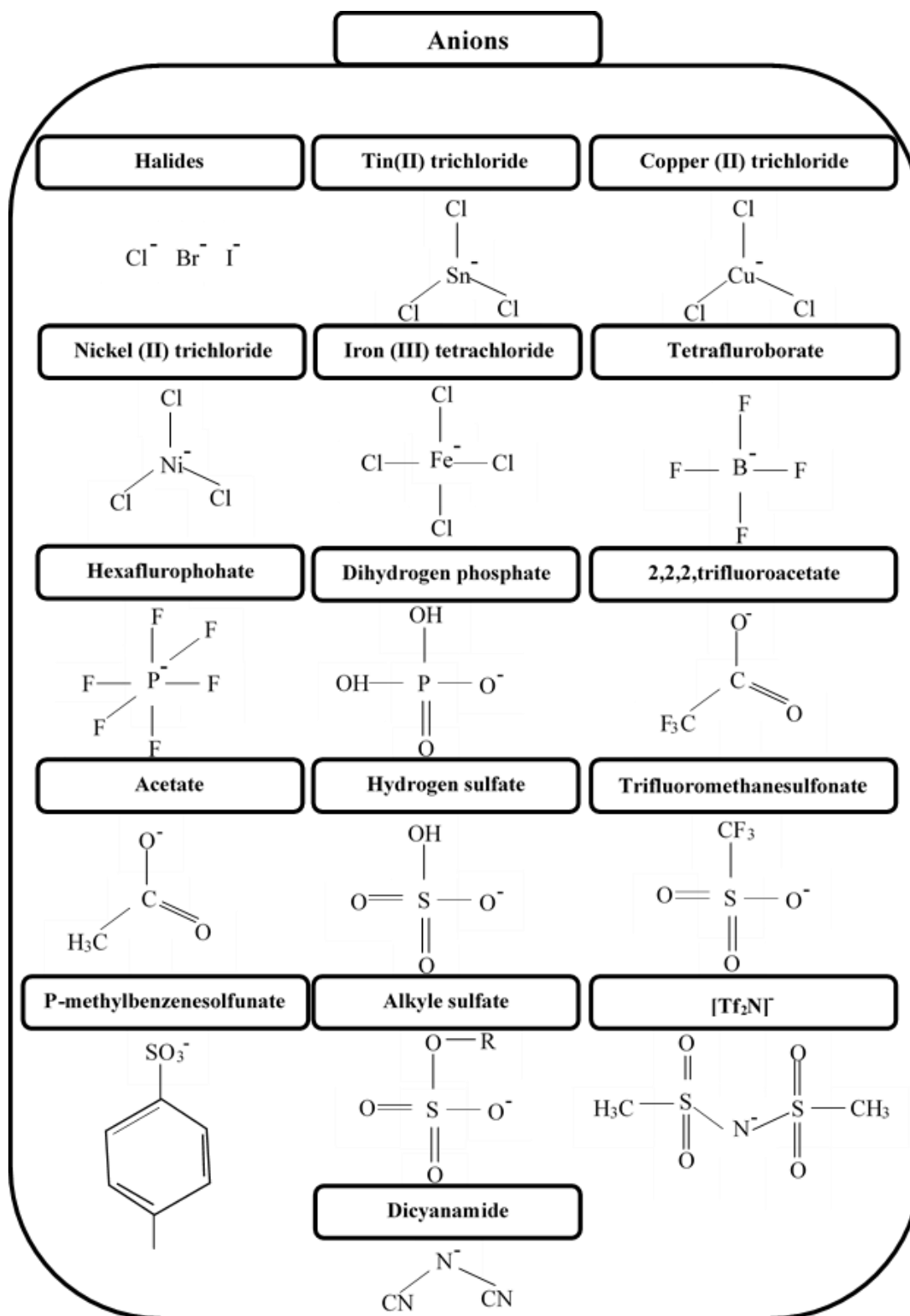
Figure 1.6. Chemical structure of anions commonly used in ILs [22, 24].
