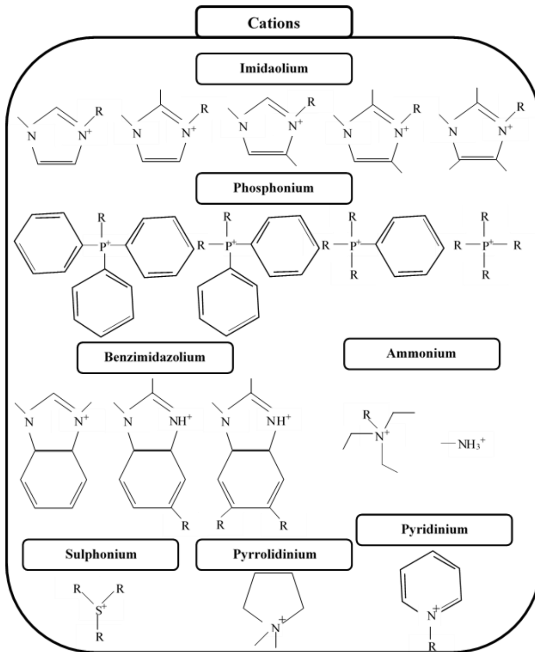
Figure 1.5. Chemical structure of cations commonly used in ILs [22, 24].
