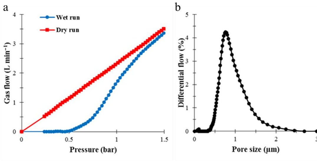
Figure 2.9. Bubble point method: a) gas flux measured during wet and dry runs; b) pore size distribution.
