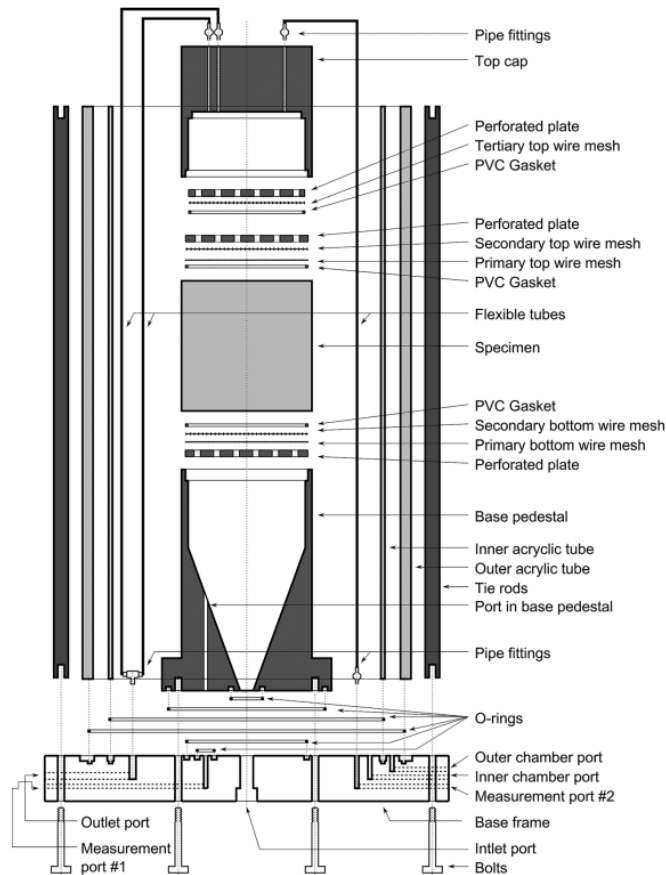
Figure 2.29 Modified triaxial-cell with double-walled design by Slangen and Fannin (2017)
