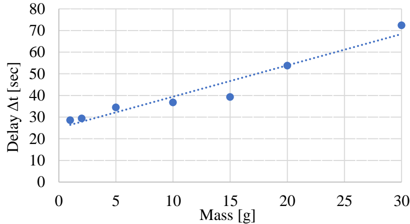
Figure_Appx. A.4 Delay Test without flow condition
