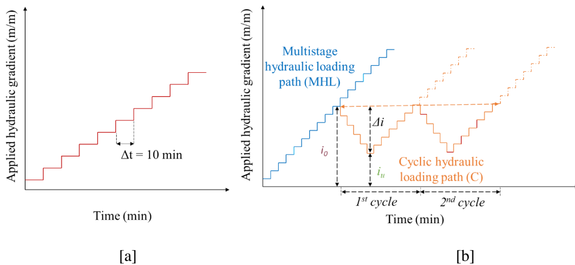
Figure 5.2 (a) Multistage hydraulic loading (b) Cyclic hydraulic loading
