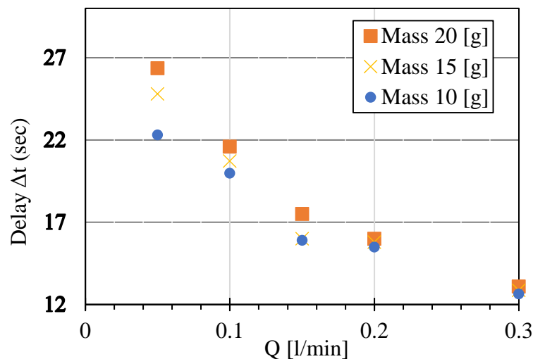
Figure_Appx. A.5 Delay of particle detection as a function of injected flow and eroded mass
