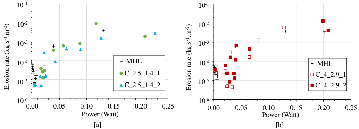
Figure 5.20 Erosion rate versus power, for one and two cycles, with i_0 equals to [a] 2.5 and [b] 4
