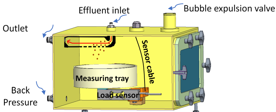
Figure_Appx. A.1 First version of effluent tank
