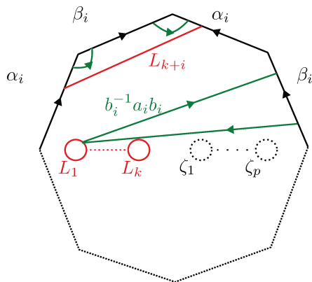
Figure 2.5: The generator b_i^{-1} a_i b_i
