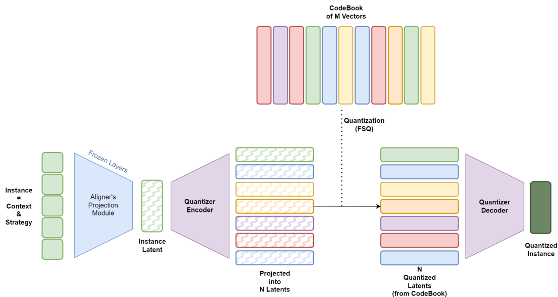
Figure 5.3: Quantization process.
