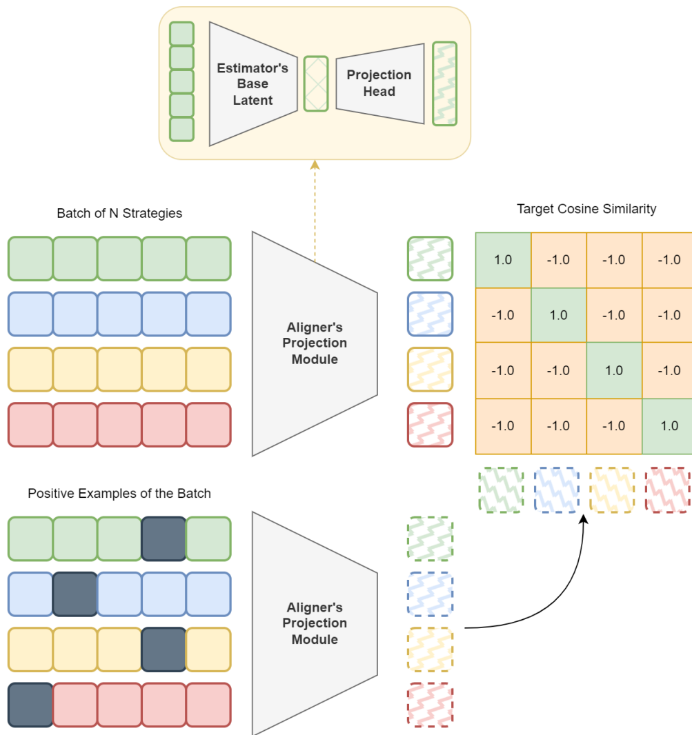
Figure 5.2: Aligner CLIP-like [Radford et al., 2021] contrastive training.
