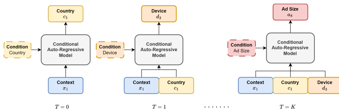
Figure 2.7: Conditional Auto-Regressive Generative Model.
