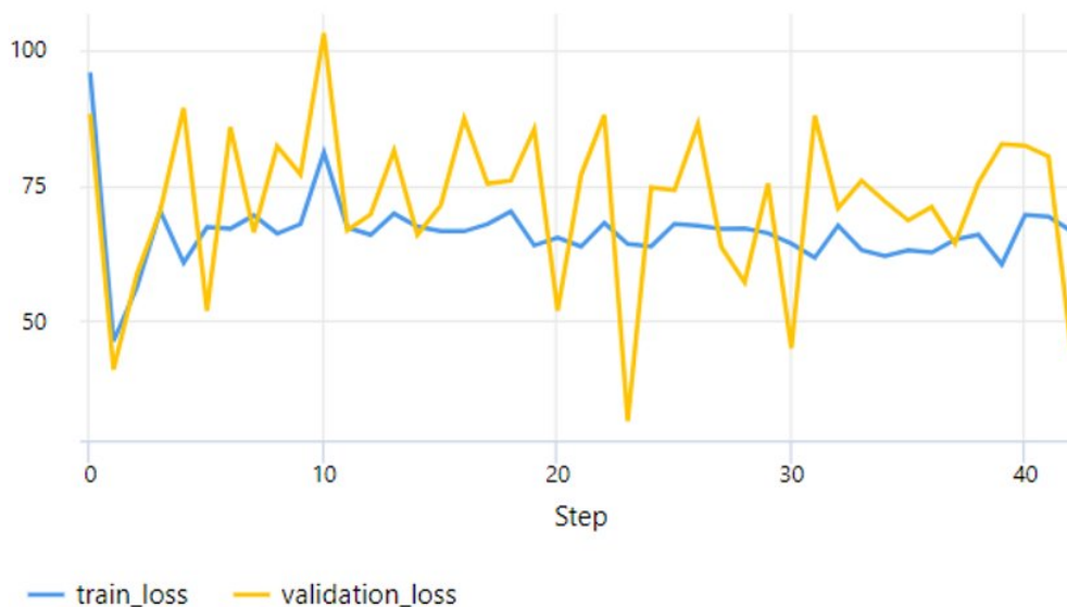
Figure 4.8: Train and validation losses unable to decrease with attention ablation despite the cyclic learning rate scheduler.
