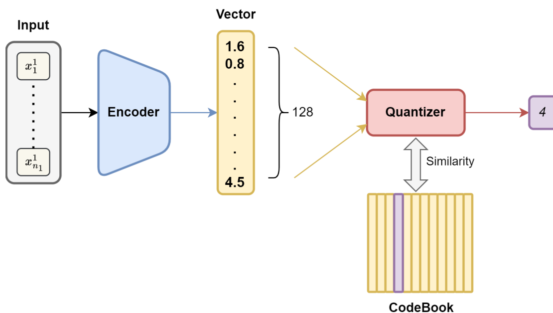
Figure 2.12: Illustration of the quantization process.
