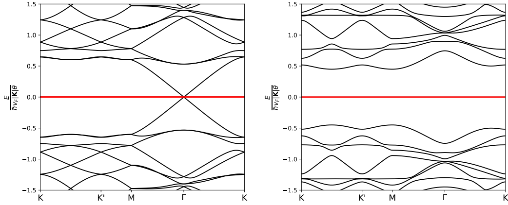
Figure 2.4: In the left panel of the figure, the completely flat bands of AAA-stacked TTG are shown. These flat bands emerge when the interlayer hopping parameter w_{AA} is set to zero, resulting in a chiral limit. The first magic angle for the AAA-stacked configuration is given by a = 0.830 ( \sim 0.77^\circ ). In the right panel of the figure, the completely flat bands of ABA-stacked TTG are depicted. Similarly, these flat bands arise in the chiral limit with w_{AA} = 0 . The first magic angle for the ABA-stacked configuration is given by a = 0.377 ( \sim 1.68^\circ ). These flat bands at the chiral limit and specific twist angles are a fascinating feature of AAA and ABA-stacked TTG structures.
