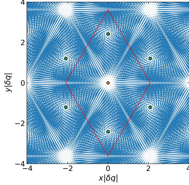
Figure 4.5: The vector field of \mathbf{a}(\mathbf{R}) on the x - y plane. Red line depicts a supermoiré unit cell centered at \mathbf{R} = \mathbf{0} . The supermoiré coordinates restoring C_{3z} symmetry in the local models are also highlighted. The AAA stacked local model is marked with orange color, while the ABA/BAB stacked local models are shown in green.
