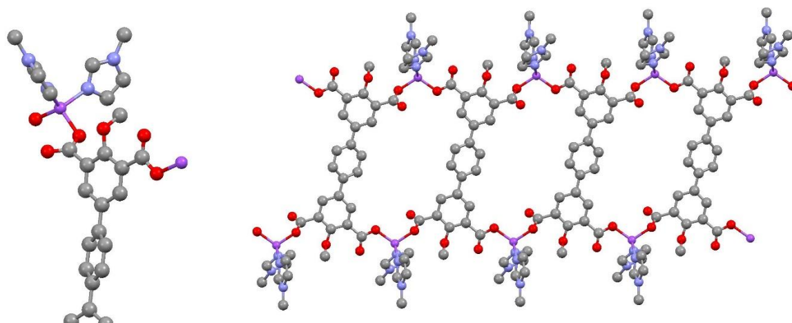
Figure 43. Left-coordination mode; Right- 1D view of LBM-50.
