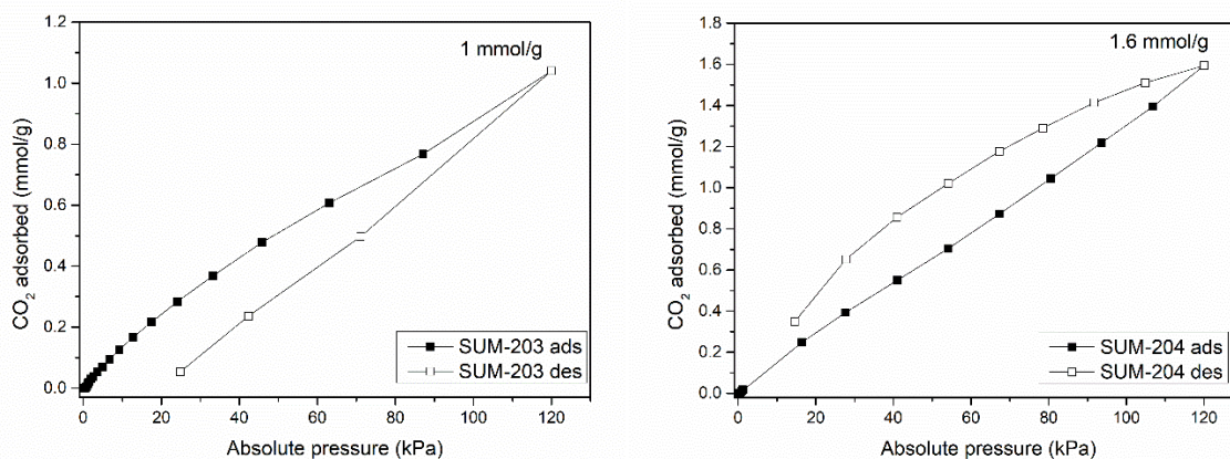
Figure 66. CO 2 adsorptions of SUM-200 series.
