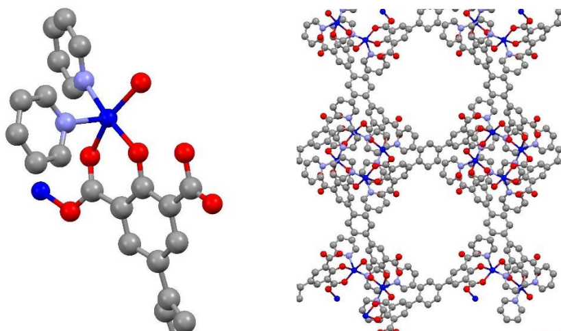
Figure 37. Left- connectivity of tectons; Right- porosity of the LBM-20, view from c-axis.
