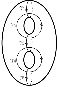
FIGURE 3.3 – Five closed curves on \Sigma_2 along which the Dehn twists generate \text{Mod}_2 . We have chosen their orientations for later use.
