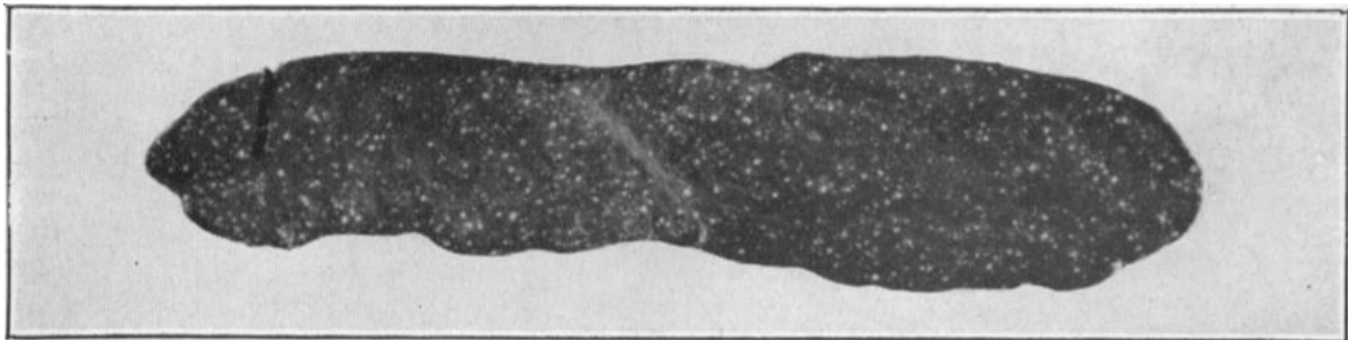
Figure 2. Spleen of a tularaemia-infected rabbit showing white granules, published in a report by Edward Francis in 1937 [4]. In his 1911 study, George McCoy remarked the presence of discrete, distinct granules in the spleen specific to animals infected with B. tularensis [2].
