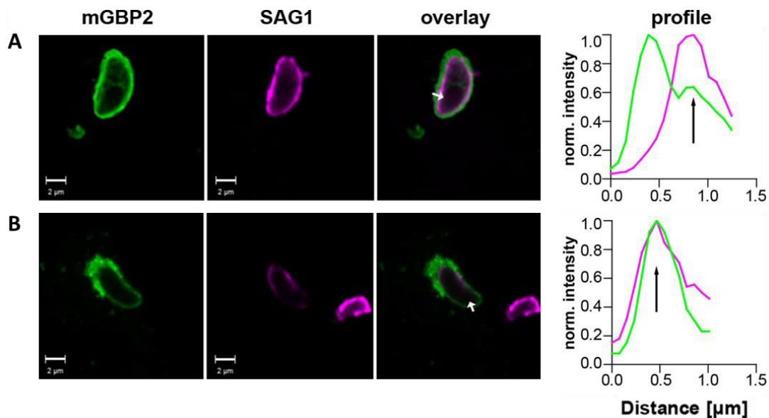
Figure 34. mGbp2 recruitment to the T. gondii parasitophosphorus membrane (A) or the plasma membrane (B) in 37.1% (A) or 61.1% (B) of parasites [391].
