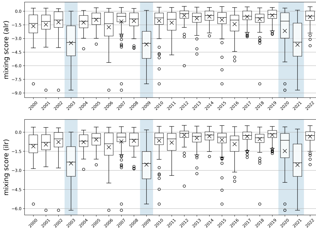
FIGURE 4.10: Comparison of the distributions of the degree of (sub)type mixing over time, calculated under the alr transformation (upper graph) and the ilr transformation (lower graph)
