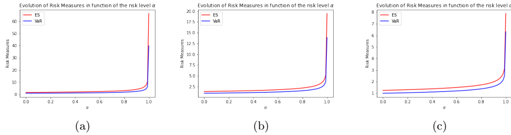
Figure 4.4: \text{VaR}_\alpha and \text{ES}_\alpha as functions of \alpha . (a) \gamma = 2.5 (b) \gamma = 3.5 (c) \gamma = 5 .
