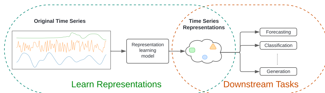
Figure 1.1: Visualization of the time series representation learning pipeline. Stage 1: Learn the time series representation through unsupervised learning. Stage 2: Train a model using this representation to address the downstream task. This graphic is inspired by Trirat et al. (2024) .
