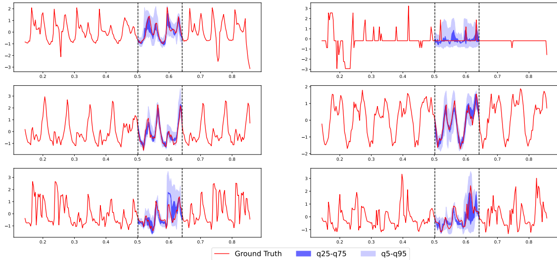
Figure 4.7: Quantifying uncertainty in block imputation of two missing days in the Electricity dataset.
