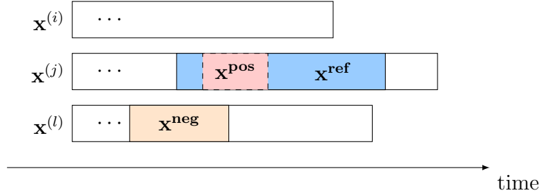
Figure 2.19: Generation of the triplet (\mathbf{x}^{ref}, \mathbf{x}^{pos}, \mathbf{x}^{neg}) in the univariate case, for the T-loss ( Franceschi et al., 2019 ) model.
