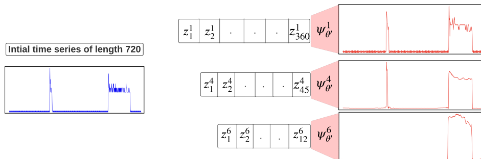
Figure 3.5: Visualization of different reconstructions for different level of representation. We can see that the deeper the architecture, the shorter the representation and the smoother the reconstruction. Computers dataset .
