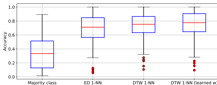
Figure 2.7: Accuracy results of the 1-NN classification methods on the 128 datasets of the UCR time series classification archive. The closer to one, the better.
