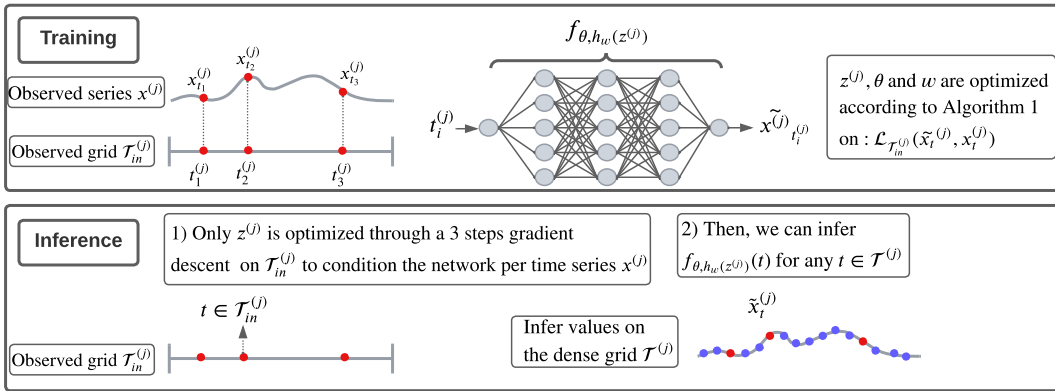
Figure 4.2: Training and inference procedures of TimeFlow for imputation. (i) During training, for each time series \mathbf{x}^{(j)} , our observations (red dots \bullet ) are restricted to the sparsely sampled grid, denoted as \mathcal{T}_{in}^{(j)} . (ii) During inference, our objective is to infer the values over the dense grids \mathcal{T}^{(j)} , on the unobserved t data points (such as the blue dots \bullet on the figure).
