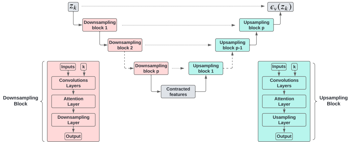
Figure D.2: Simplified overview of the denoiser UNet 1D architecture.
