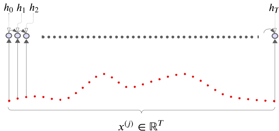
Figure 2.14: Simplified illustration of recurrent layers.
