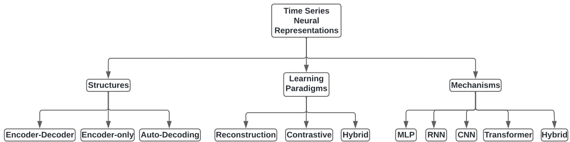
Figure 1.2: Taxonomy of research branches in neural representation learning for time series.
