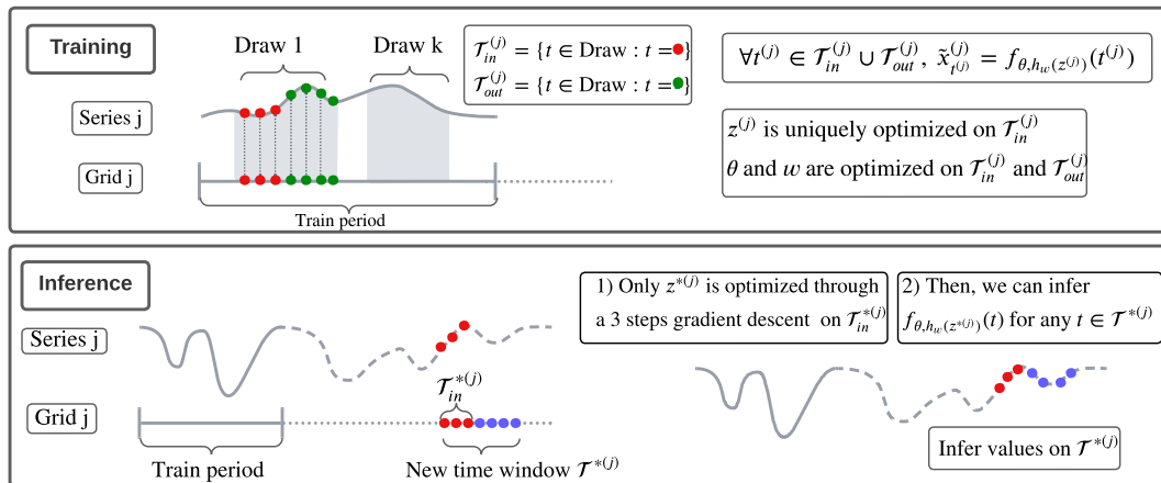
Figure 4.4: Training and inference procedure of TimeFlow for forecasting. (i) During training (top-figure), for each time series x^{(j)} , we observe some look-back window/horizon drawing pairs in the trained period. TimeFlow is trained with Algorithm 1 to predict all observed timestamps in this drawing pairs while being conditioned by the observed look-back window. (ii) Once TimeFlow is optimized, the objective during inference (bottom-figure) is to infer the horizon over new time windows (blue dots \bullet ) while being conditioned by the newly observed look-back window (red dots \bullet ).
