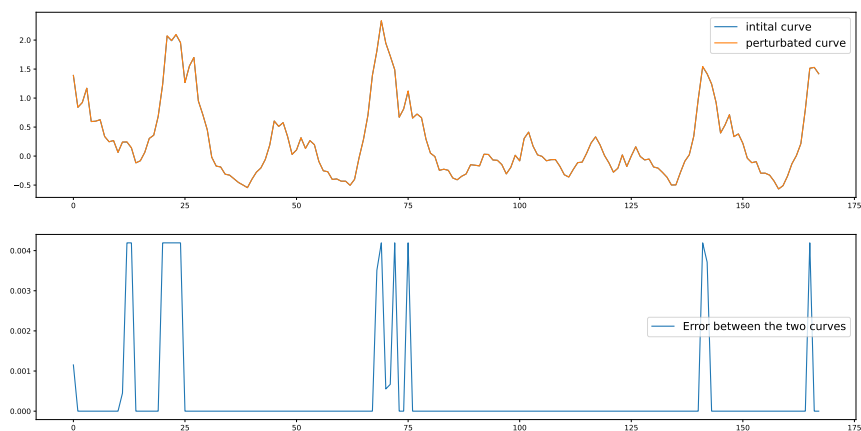
Figure 5.5: Small perturbation to the modulation of the fourth layer, 50th channel.
