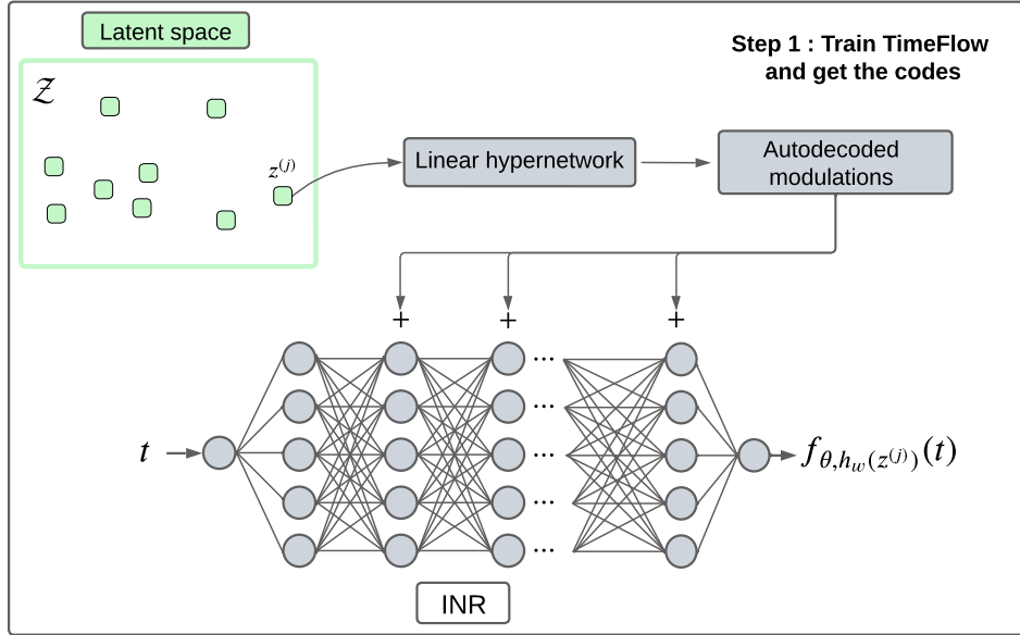
Figure 5.7: Step one. Fit TimeFlow and get codes from the latent space.
