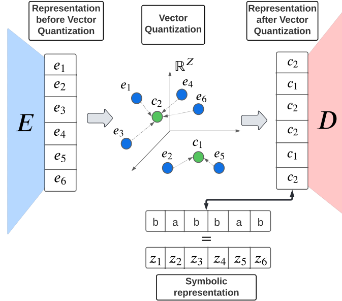
Figure 3.7: Visualization of the vector quantization mechanism in the context of an auto-encoder. E and D stand respectively for Encoder and Decoder.
