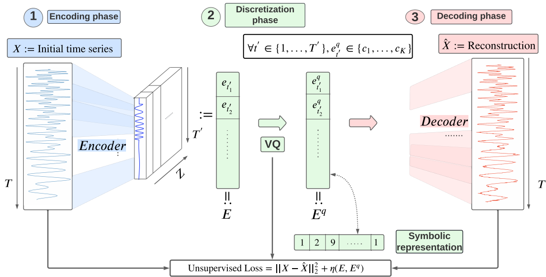
Figure 3.8: Global unsupervised architecture overview. \eta refers the last two terms in Equation (3.2).
