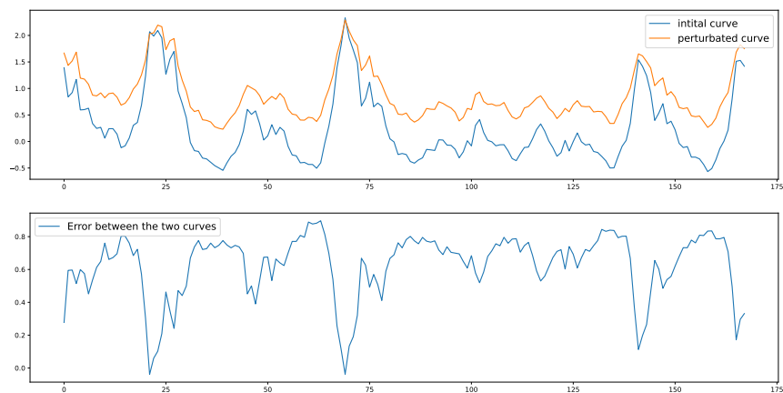
Figure 5.4: Small perturbation to the modulation of the third layer, 51th channel.
