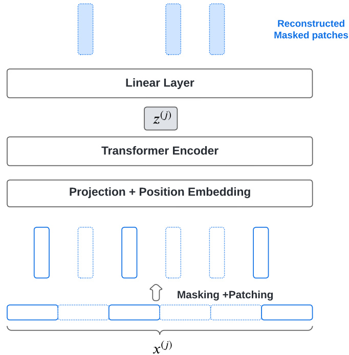
Figure 2.22: PatchTST unsupervised architecture.
