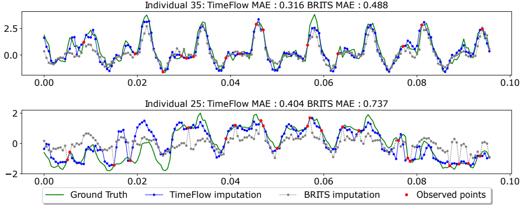
Figure 4.3: Electricity dataset. TimeFlow imputation (blue line) and BRITS imputation (gray line) with 10% of known point (red points) on the eight first days of samples 35 (top) and 25 (bottom).
