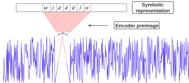
Figure 3.12: Local interpretability for a class 1 (includes triangle) instance.
