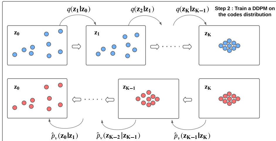
Figure 5.8: Step two. train a DDPM on the latent code distributions
