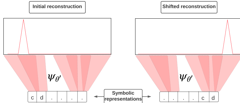
Figure 3.4: Shift equivariance of \psi_{\theta'} . The subsequence c d appear at two different locations in the representation: \psi_{\theta'} should decode the same pattern with a shift in time.
