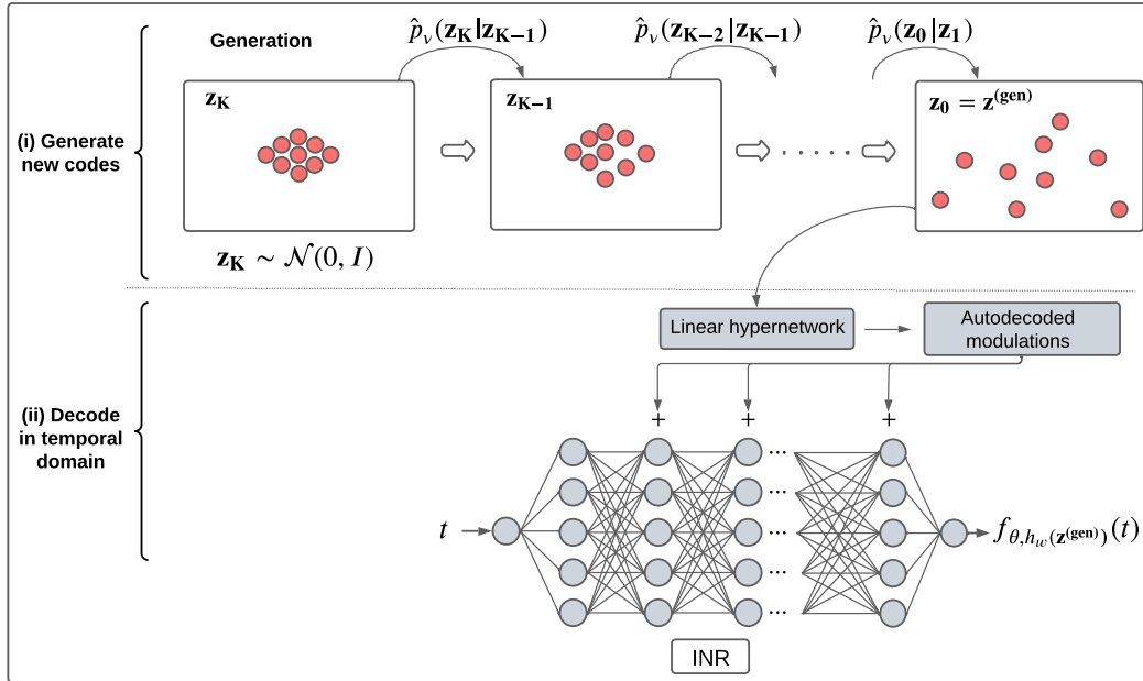
Figure 5.9: Overview of the generation procedure.
