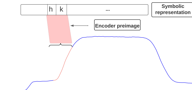
Figure 3.10: Local interpretability for a class 0 (Gun) instance.
