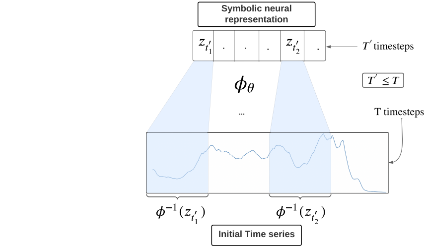
Figure 3.2: Temporal consistency visualization. Coffee dataset .
