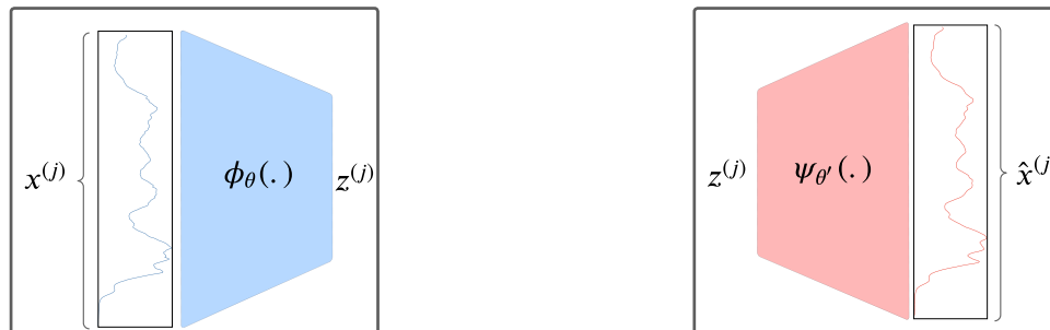
(a) Time series neural representation: encoder-only architecture.
