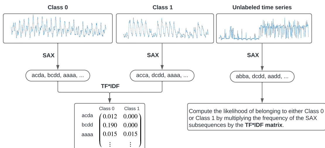
Figure 2.12: Visualization of the SAX-VSM classification decision. This graphic is inspired by Senin and Malinchik (2013).
