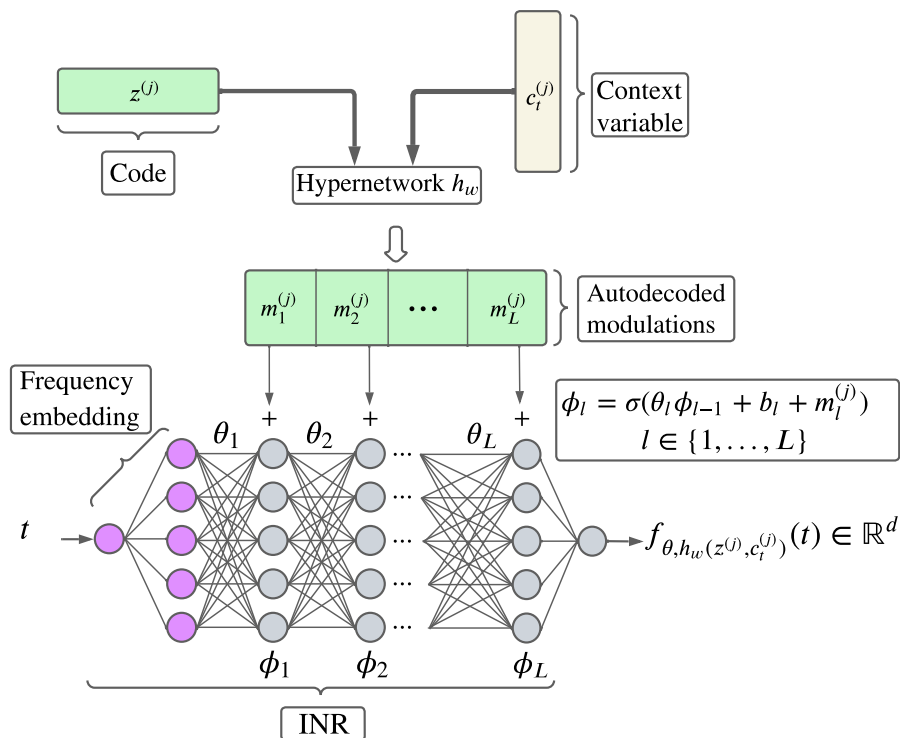
Figure 6.1: TimeFlow architecture conditioned on context variable.
