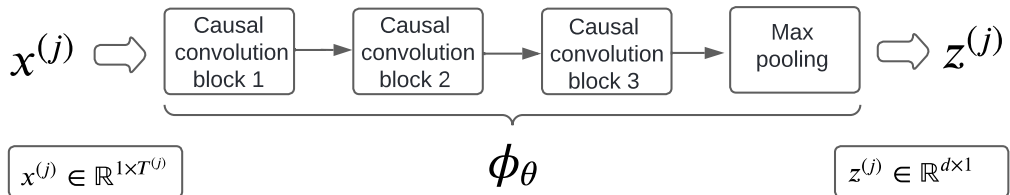
Figure 2.20: Simplified illustration of the causal CNN encoder with 3 causal convolution blocks applied on a univariate time series.
