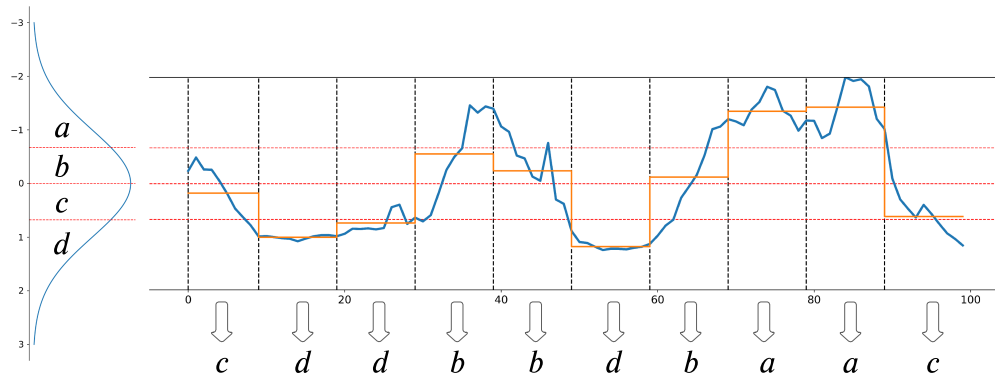
Figure 2.11: SAX representation of some part of the french national Hydraulic power generation time series in 2020.
