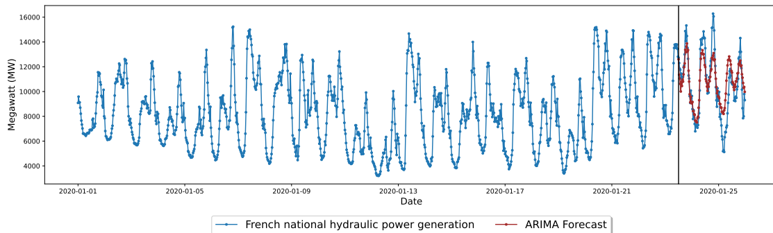
Figure 2.3: Visualization of an \text{ARIMA}(p = 24, d = 1, q = 1) forecast on the french national hydraulic power generation time series.
