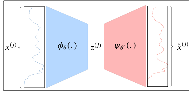
Figure 2.17: Time series neural representation: encoder-decoder structure.
