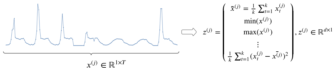
Figure 2.8: Basic time series representation vector of statistic features.
