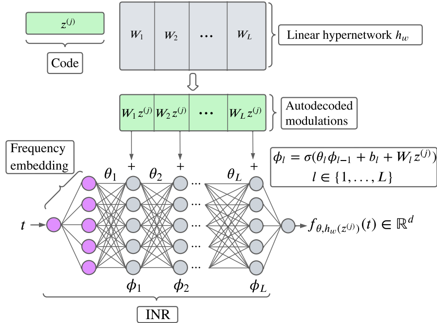
Figure 4.1: Overview of TimeFlow architecture. Forward pass to approximate the time series x^{(j)} . \sigma stands for the ReLU activation function.
