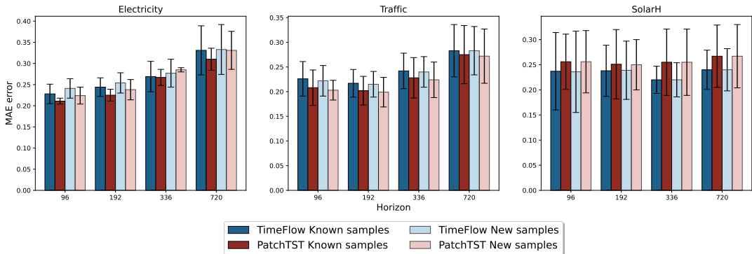
Figure 4.5: Mean MAE forecasting task results over different horizons in the context of generalization to new time series. Comparison of TimeFlow and PatchTST performances on the Electricity , Traffic and SolarH datasets.
