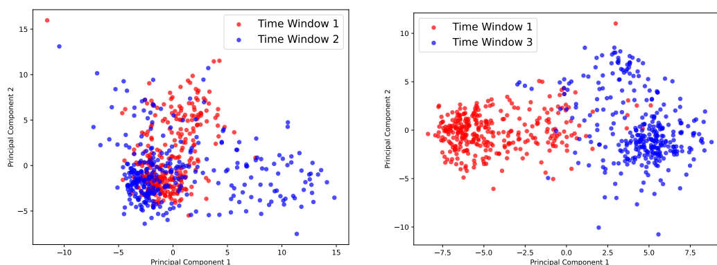
(a) The temporal shift between the two codes distribution is 3 months. (b) The temporal shift between the two codes distribution is 6 months.
