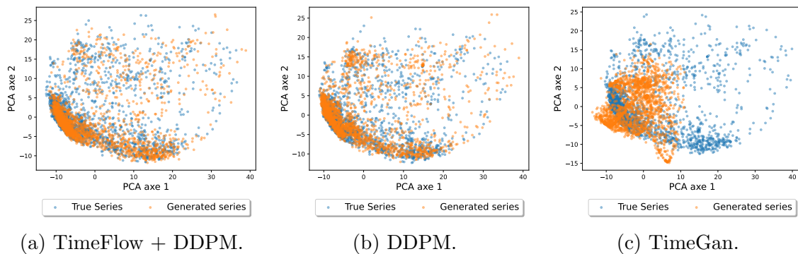
Figure D.3: PCA visualization comparing generated and test time series for the three considered methods.
