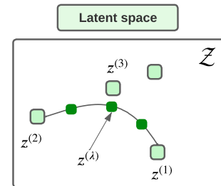
Figure 5.1: Latent space interpolation path (Bezier curve).
