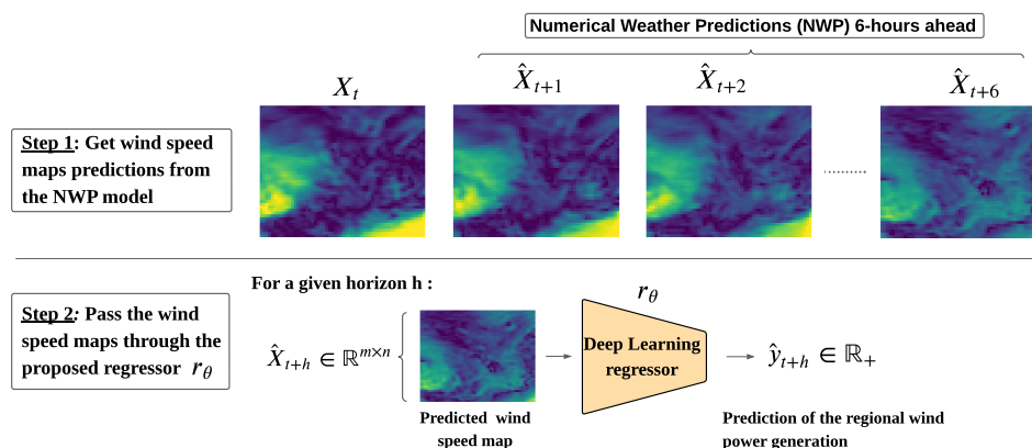
Figure A.1: Global scheme for wind power forecasting. Every 6 hours, the NWP model produces hourly forecasts. Each map is processed independently by the regressor which maps the grid to the wind power corresponding to the same timestamp.
