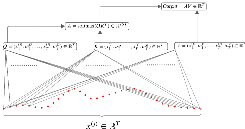
Figure 2.16: Simplified illustration of an attention layer.
