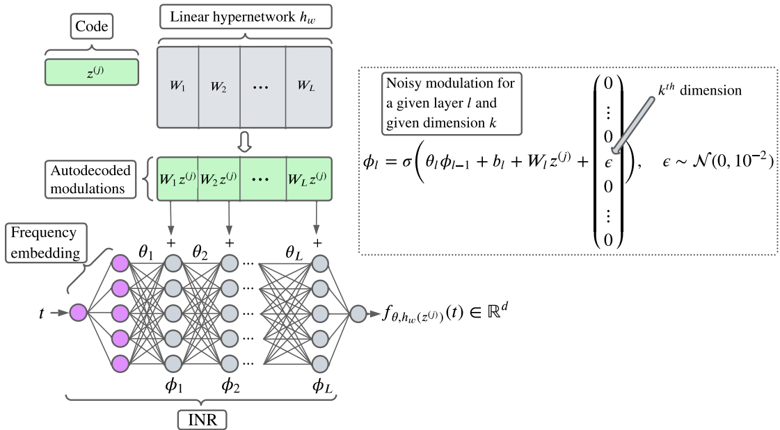
Figure D.1: Noisy modulation visualization.
