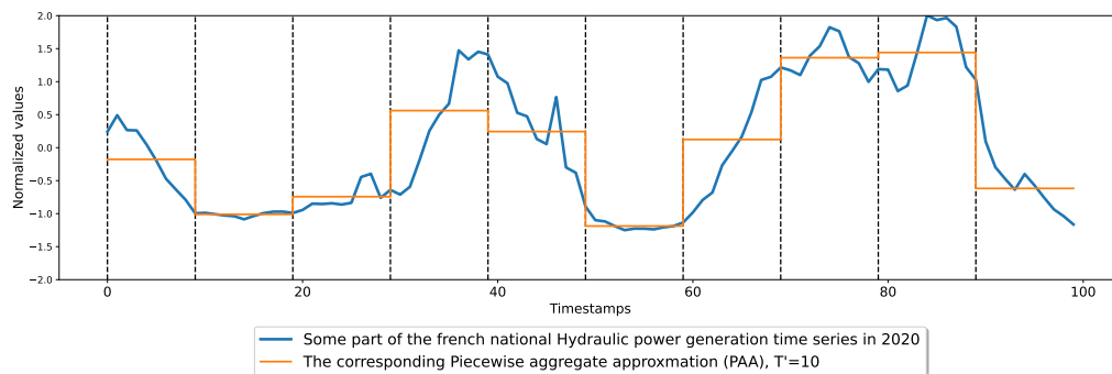
Figure 2.10: PAA of some part of the french national hydraulic power generation time series in 2020.
