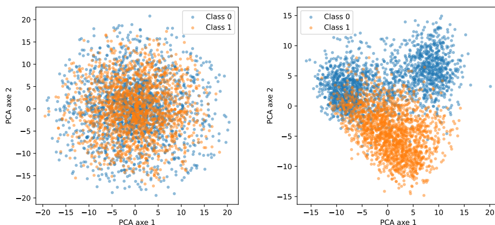
(a) PCA applied on the initial time series. (b) PCA applied on the representations.
