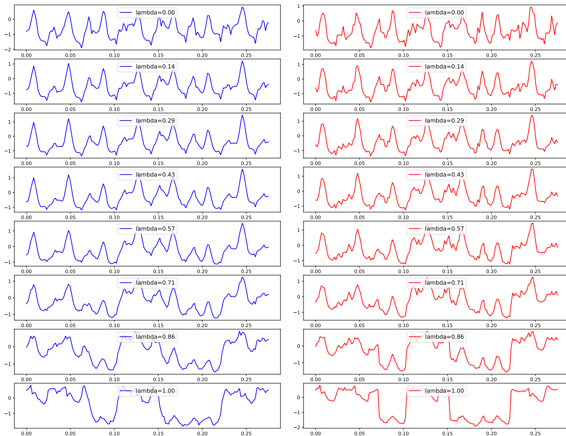
Figure 5.2: Electricity dataset. Visualization of the decoded Bézier interpolations between latent codes \mathbf{z}^{(1)} and \mathbf{z}^{(2)} (left plot), compared with Bézier interpolations of ground truth time series \mathbf{x}^{(1)} and \mathbf{x}^{(2)} (right plot).
