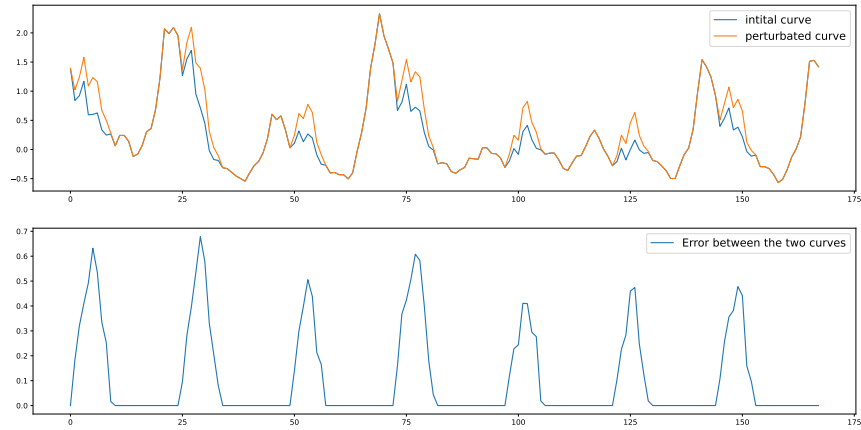
Figure 5.3: Small perturbation to the modulation of the third layer, 50th channel.
