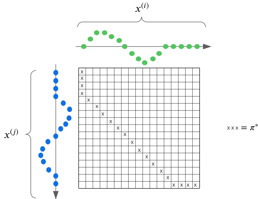
Figure 2.6: DTW explanation: illustration of the optimal warping path \pi^* .
