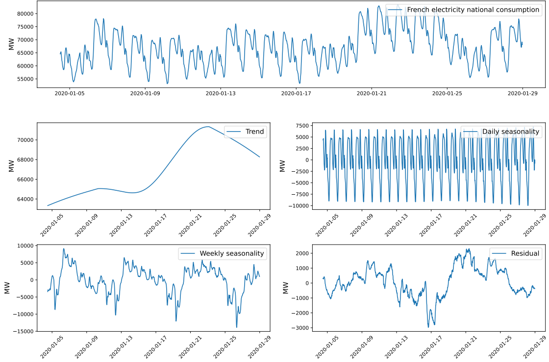
Figure 2.9: Additive STR decomposition on the french national electricity consumption over three weeks in January 2020.
