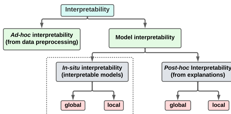
Figure 3.1: Interpretable time series model taxonomy introduced in Wang (2021).
