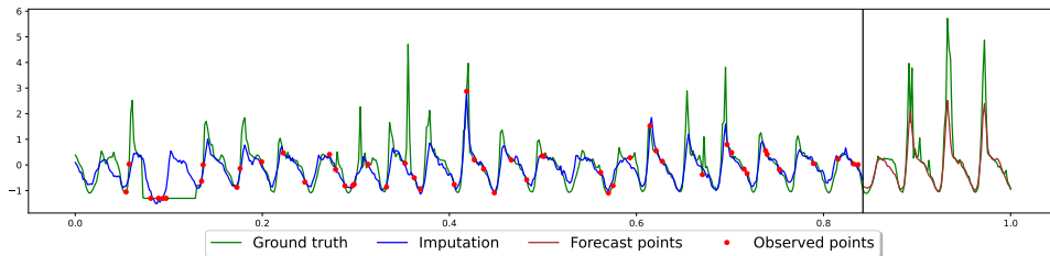
Figure 4.6: Traffic dataset, sample 95 . In this figure, TimeFlow simultaneously imputes and forecasts at horizon 96 with a 10% partially observed look-back window of length 512.
