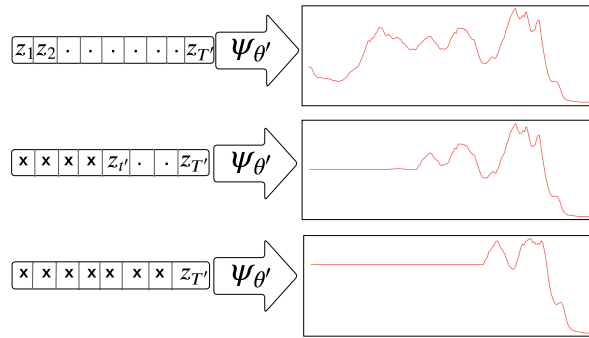
Figure 3.3: Visualization of how the representation is decoded for the complete representation, as well as for half of the representation and for only the last element. Coffee dataset .
