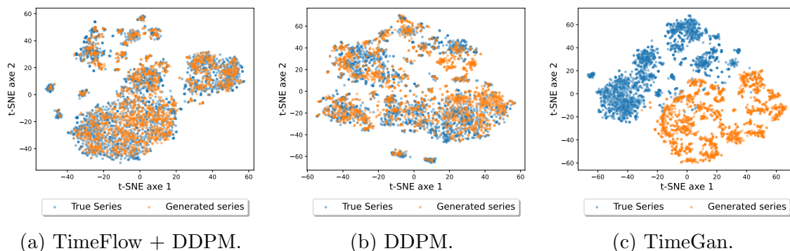
Figure 5.10: t-SNE visualization comparing generated and test time series for the three considered methods.
