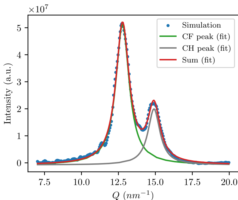
Figure B.31: GIXD \theta -integrated diffractogram for small values of \theta ( i.e. the intensity presented in Figure B.1 integrated along \theta in the range of 0 rad to 0.1 rad, or about 0^\circ to 5.73^\circ , as a function of Q ), calculated from the final configuration of the MD simulation trajectory of the pure F10H18 hemimicelle, which contained 3400 molecules of PFAA. The blue circles represent the data points retrieved from the calculation and the curves represent the fitted Lorentzian peaks corresponding to the proposed structures, labelled “CF peak” (green) and “CH peak” (grey). The red curve is the cumulative sum of the remaining fitted curves.
