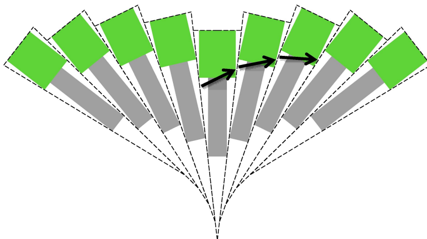
Figure 8.5: Geometrical relation between the conical-like shape of the PFAA molecules, the shift of the molecules relatively to each other, trying to align the dipoles at the \text{CH}_2\text{-CF}_2 junctions, and the consequent development of the dome’s curvature and formation of the central pit. The green and grey rectangles represent the fluorinated and the hydrogenated chains, respectively (not to scale). The dashed lines purport the conical shape of the PFAA molecules; the water molecules are not represented.
