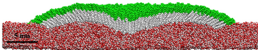
Figure A.4: Representative snapshot of the final state of the MD simulation trajectory, illustrating a side view of a cross-section cut through the middle of the surface aggregate modelled with the OPLS force field at the vacuum TIP4P/2005 interface. The CH and CF chains are coloured white and green, respectively. The water molecules are coloured red and white (oxygen and hydrogen atoms, respectively).
