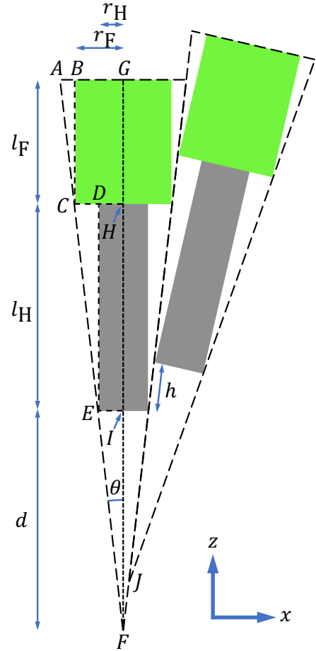
Figure 9.4: Longitudinal cross-section of the two-cylinder geometrical construction considered for the PFAA molecules. The capital letters mark some relevant points. The symbols and notation are presented in the text.
