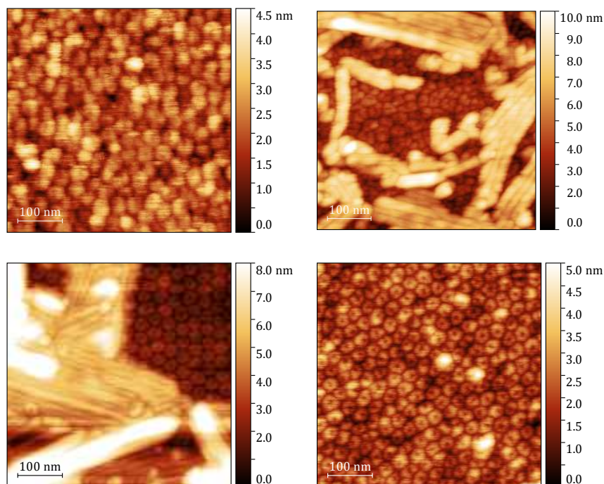
Figure 10.14: AFM height images of F8H18 thin films prepared by spin coating (top row) or by simple evaporation (bottom row) on silicon wafers previously wet with 2,2,2-trifluoroethanol (TFE).
