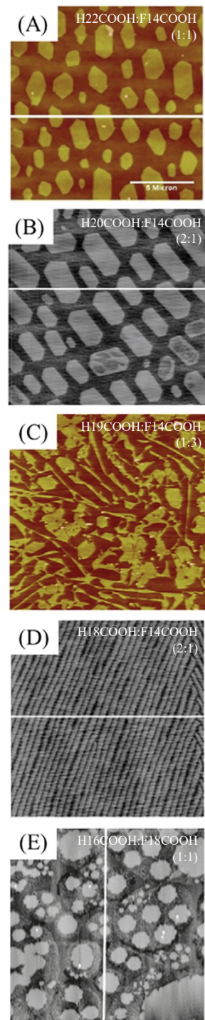
Figure 3.1: AFM images of phase-separated mixed monolayer systems (composition in top-right corners; image sides 5\ \mu\text{m} (D), 10\ \mu\text{m} (C, E), 15\ \mu\text{m} (A) and 20\ \mu\text{m} (B)). Adapted from [61].
