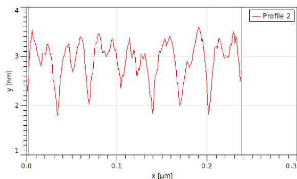
Figure 10.9: Height profile along the segment number 2 in Figure 10.8 (bottom left). The vertical lines mark the positions used to measure the distance corresponding to the lateral juxtaposition of 7 hemimicelles.
