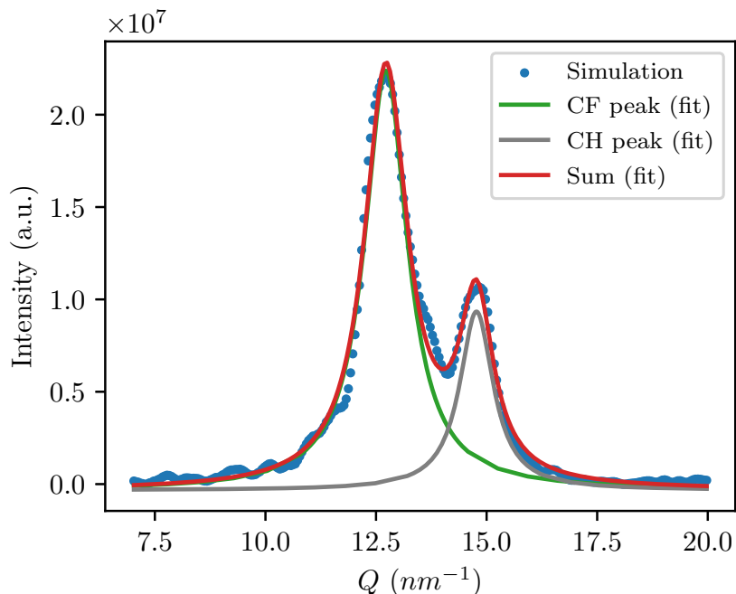
Figure B.2: GIXD \theta -integrated diffractogram for small values of \theta ( i.e. the intensity presented in Figure B.1 integrated along \theta in the range of 0 rad to 0.1 rad, or about 0^\circ to 5.73^\circ ), as a function of Q ), calculated from the final configuration of the MD simulation trajectory of the pure F8H14 hemimicelle, which contained 1700 molecules of PFAA. The blue circles represent the data points retrieved from the calculation and the curves represent the fitted Lorentzian peaks corresponding to the proposed structures, labelled “CF peak” (green) and “CH peak” (grey). The red curve is the cumulative sum of the remaining fitted curves.
