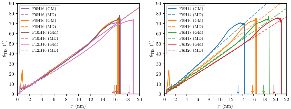
Figure 9.10: Average tilt angle ( \theta_{\text{Tilt}} , full lines) as a function of the radial distance to centre of the aggregate ( r ) for the simulated limit-size aggregates or hemimicelles of FnH16 ( n = 6, 8, 10, 12 ; left) and of F8Hm ( m = 14, 16, 18, 20 ; right). The dashed lines represent the corresponding dependency of \theta_{\text{Tilt}} on r predicted with the geometrical model. The arrows mark the radii of the hemimicelles computed from the MD simulation trajectories, using the same colour coding as the one presented in the legend.
