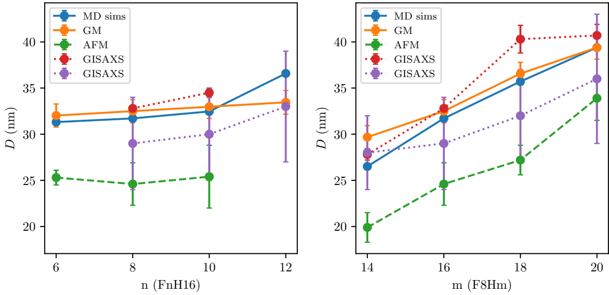
Figure 9.9: Diameter ( D ) of the PFAA hemimicelles formed at the air–water interface estimated with the geometrical model (orange, full lines) and computed from the simulation trajectories of the limit-size aggregates (blue, full lines) as functions of: the number of carbon atoms in the CF chain or n , for m=16 (FnH16; left); the number of carbon atoms in the CH chain or m , for n=8 (F8Hm; right). For comparison, other literature results obtained using different experimental techniques are also shown, namely: AFM (green, dashed lines), from Ref. [9], and GISAXS, from Refs. [5, 35] (red, dotted lines) and [36] (purple, dotted lines). The lines are guides to the eye.
