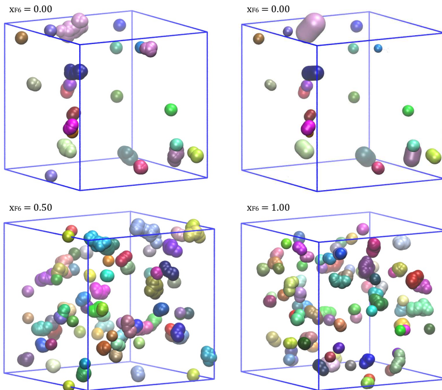
Figure 12.9: Snapshots of representative configurations of the mixtures of F6+H6 with x_{F6} = 0.00 (pure H6; top row), x_{F6} = 0.50 (bottom left) or x_{F6} = 1.00 (pure F6; bottom right), simulated at T = 298 K, displaying the voids in these systems identified by R_b colouring with R_b^{\text{probe}} = 0.20 nm. The F6 and H6 molecules are omitted for clarity. The void spherocylinders are illustrated for x_{F6} = 0.00 (pure H6; top right); the remaining images represent the void sites in a spacefill model to scale. Each void spherocylinder and the corresponding set of void sites, in the different representations, are coloured differently.
