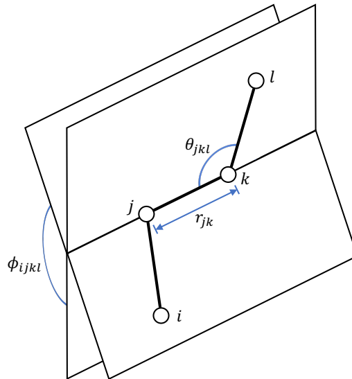
Figure 5.2: Bond length ( r_{jk} ), bond angle ( \theta_{jkl} ) and dihedral angle ( \phi_{ijkl} ) definitions for a sequence of four covalently bonded atoms i , j , k and l . The \phi_{ijkl} follows the IUPAC convention, for which \phi_{ijkl} = 0^\circ for the cis configuration. However, the implementation of this angle in some FFs is based on the supplementary angle \varphi_{ijkl} = 180^\circ - \phi_{ijkl} .
