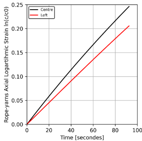
Figure 6.27 – Change of the rope-yarns axial logarithmic strain \ln\left(\frac{c}{c_0}\right) with time [minutes]
