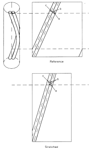
Figure 6.28 – Axial shear described by Leech (Leech, 2002)
