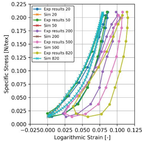
Figure 5.21 - Specific Stress [N/tex] versus logarithmic strain [-] during fatigue test for chosen cycles. Comparison between simulation using the POLYAMOR law and the experimental data.
