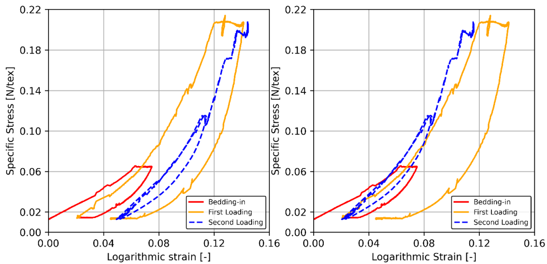
Figure 4.13 – Left : specific stress [N/tex] versus logarithmic strain for LC45 test during the bedding-in [red solid line], the first creep and recovery (yellow solid line) and the second creep (dashed blue line). Right : specific stress [N/tex] versus logarithmic strain for LC45 test with a shift of the second creep (dashed blue line) to match the first creep (yellow solid line)
