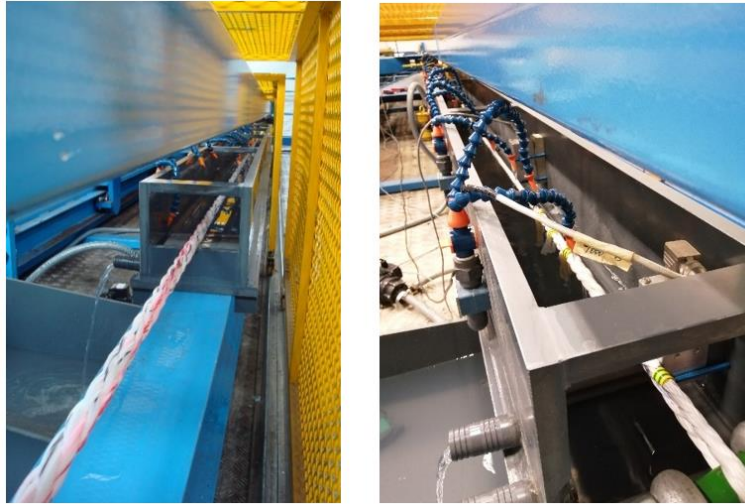
Figure 2.11 - Servo-hydraulic machine with 300 kN capacity: (left) 6-meter-long 7T sub-rope sample installed on the testing machine, (right) 4T sub-rope sample installed on the testing machine.
