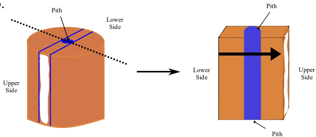
466 Figure 4 : Protocol for measuring the MFA of tension wood in poplar stems. (a) Determination of 467 the 002 arc intensity from the diffraction pattern of a sample. (b) Diametral sticks were cut from the 468 upper and lower faces of the stems, and the MFA was measured across the entire length of the 469 diametral stick.
