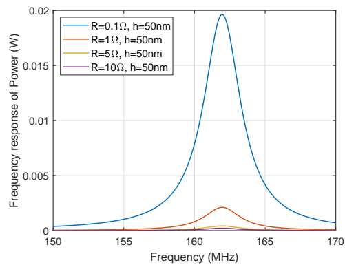
(c) Power frequency response
