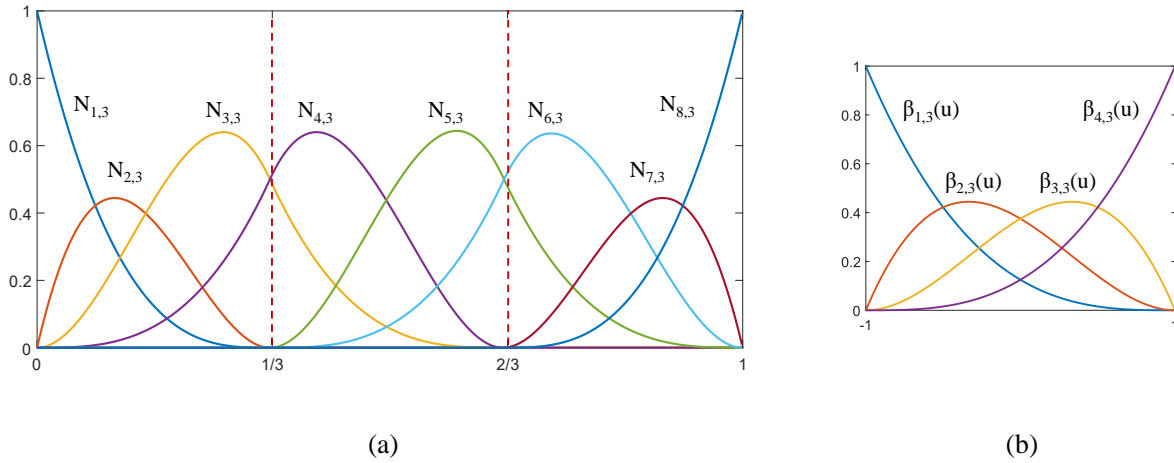
Figure 3.3: (a) 1D B-spline basis, degree p = 3 and knots \xi=[0, 0, 0, 0, 1/3, 1/3, 2/3, 2/3, 1, 1, 1, 1] ; (b) 1D Bernstein basis of degree p = 3 ;
