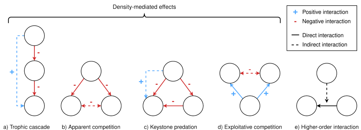
Figure 1.4: Schematic representation of indirect interactions. Species are depicted as circles and interactions as arrows. The arrow points to the species receiving a positive or negative outcome. Only the relevant interactions are represented (e.g. the predation in a) is only symbolized with a negative outcome for the prey). Density-mediated effects include: a) trophic cascade, where a top predator indirectly benefits a species at an inferior trophic level; b) apparent competition, when a predator induces indirect competition between two prey species; c) keystone predation, where a predator indirectly benefits a subordinate competitor; d) exploitative competition, where two predators indirectly compete for the same resource. e) Higher-order interactions occur when a species modifies the nature of the interaction between two other species (on this diagram, the trophic level is irrelevant).
