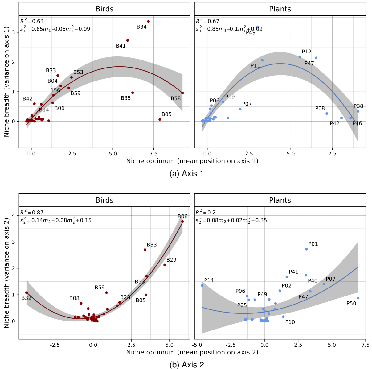
Figure 2.1.5: Niche breadth versus niche optimum on the 2 multivariate axes. Niche breadths (variances) and niche optima (means) were computed with reciprocal scaling. The top graphs (a) shows the relationship on axis 1 and the bottom graphs (b) on axis 2. The left and right panels represent bird and plant species, respectively. The solid line is the prediction of the best linear model and the gray shading represents the 95% confidence interval around the predicted mean value. The coefficient of determination ( R^2 ) and the linear model equation are shown in the top left corner.
