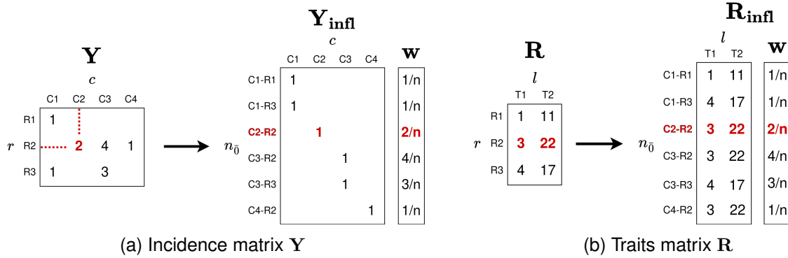
Figure 2.3.1: Correspondence between original and inflated matrices. (a) Correspondence between an incidence matrix \mathbf{Y} and the inflated matrix \mathbf{Y}_{\text{infl}} . (b) Correspondence between a traits matrix \mathbf{R} and the inflated matrix \mathbf{R}_{\text{infl}} . In this example, \mathbf{Y} represents the interactions between r = 3 resources and c = 4 consumers. \mathbf{R} represents l = 2 traits for resource species. For clarity, zeroes are omitted in the matrices. In the inflated matrices, each row corresponds to an interaction type from the original matrix ( n_{\bar{0}} = 6 interaction types). The weight vector \mathbf{w} contains interaction weights, computed as the weight of the interaction from the original matrix (where n is the grand total of \mathbf{Y} ). The interaction between R2 and C2, and the corresponding traits for R2 are highlighted in all matrices to show their correspondence.
