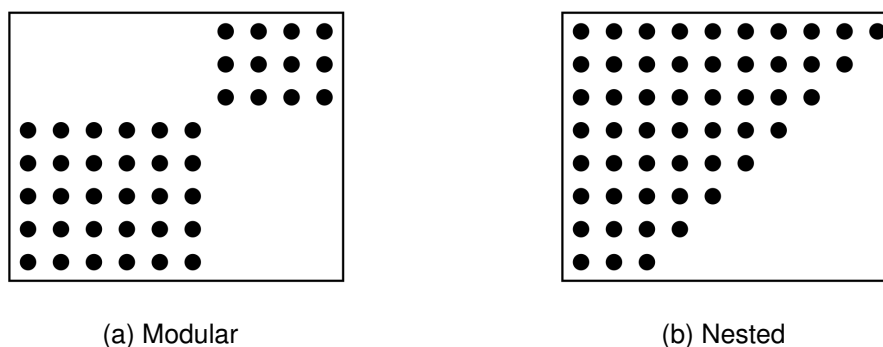
Figure 1.8: Matrix representations of perfectly modular (a) and nested (b) networks. Rows and columns of the matrices represent respectively the two types of nodes of a bipartite network, and non-null values in the matrix (dots) represent a link.
