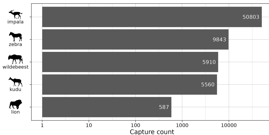
Figure 3.I.1: Capture count for each species. These counts take into account the number of times capture events without accounting for the number of individuals on the picture. The x-axis is in log-scale. Silhouette images from PhyloPic by Lukasiniho (wildebeest), Margot Michaud (lion), Robert Hering (kudu), Zimices (zebra) and an unknown author (impala).
