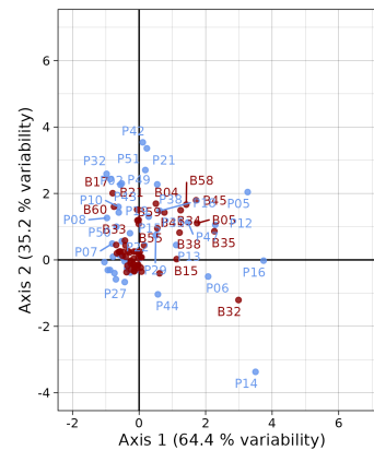
(c) Bird niches ( V^* and U )
