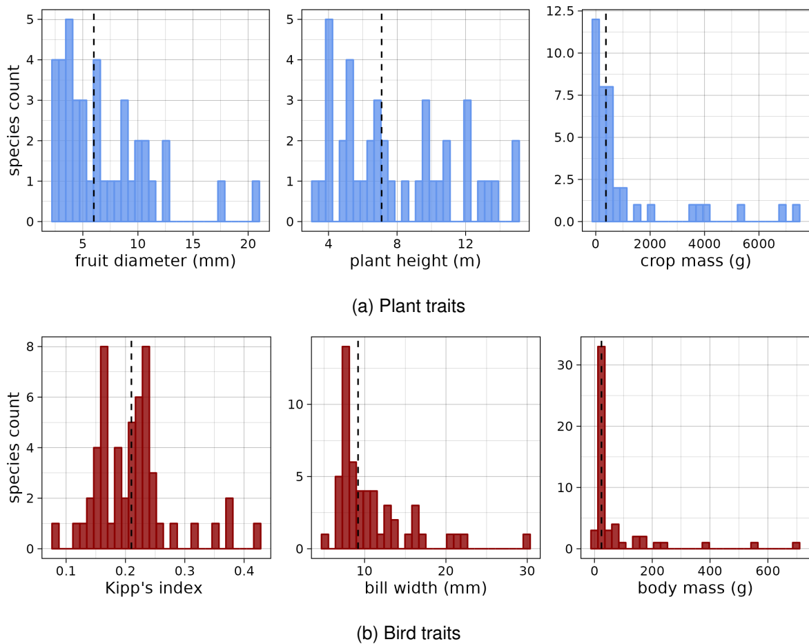
Figure A.1: Bird and plant traits histograms. a) represents the distribution of plant traits in the community and b) for the birds traits. The vertical dashed line represents the median and the y-axis represents species count.
