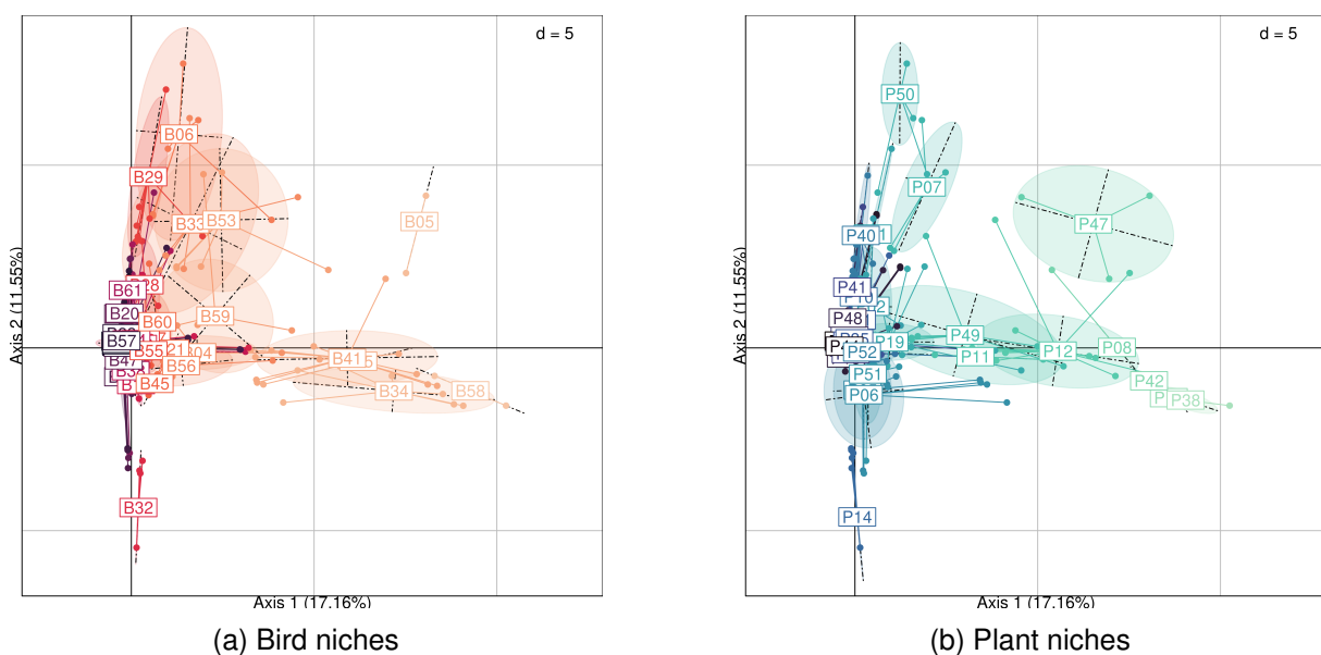
Figure 2.1.4: Reciprocal scaling of the birds-plants interaction network. Points correspond to the correspondences h_k(i, j) in the first 2 dimensions. The correspondences are grouped by bird species (a) or plant species (b). The species label are placed at the reciprocal scaling mean, and the ellipses correspond to the bivariate normal distribution of variances and covariances given by reciprocal scaling (with a scaling factor of 1.5, i.e. the ellipse axes lengths are equal to 1.5\sqrt{\lambda_k} on axis k , corresponding to around 67% of the points contained in the ellipse). Species are colored according to their position on the first axis.
