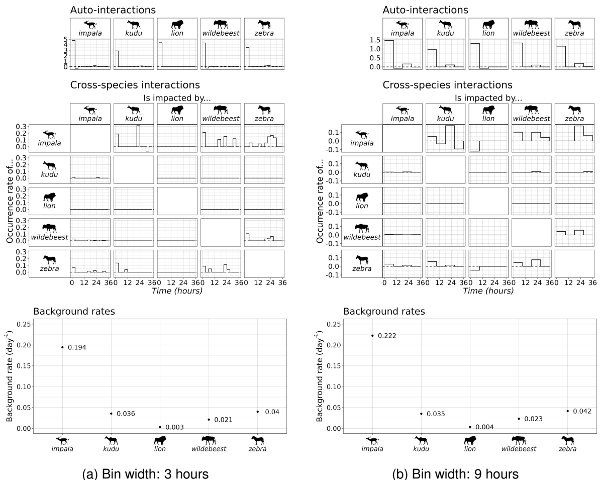
Figure S4: Inference of a multivariate Hawkes process with different bin widths. (a) shows the parameters inferred with 3 hours bins and (b) the parameters inferred with 9 hours bins. Silhouette images from PhyloPic by Lukasiniho (wildebeest), Margot Michaud (lion), Robert Hering (kudu), Zimices (zebra) and an unknown author (impala).
