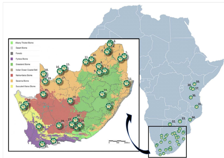
Figure 4.1.1: Location of the Snapshot Safari camera trap grids. Figure 1 from Pardo et al. (2021).
