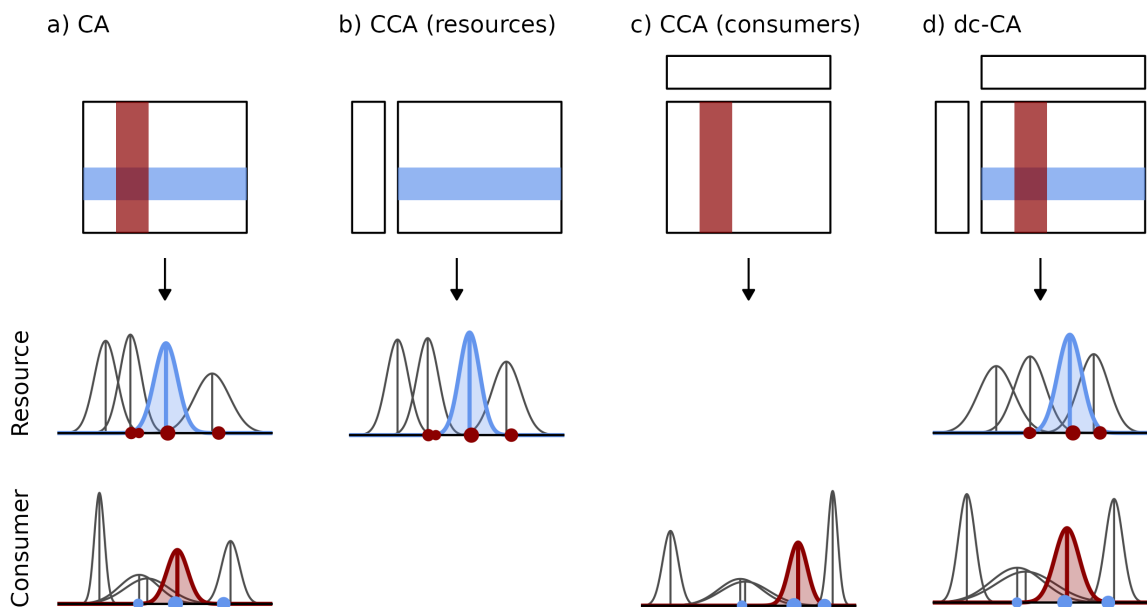
Figure 2.D.1: Summary of CA methods and niche inference. Each column represents a CA method. The first row represents the matrices inputs, and the second and third rows represent the inferred species niches in one dimension. In each case, one species for which the niche is computed is highlighted in blue (resource) or in red (consumers). The interacting partners of the species are represented as colored points on the niche axis (red for consumers and blue for resources), with their size proportional to their abundance.
