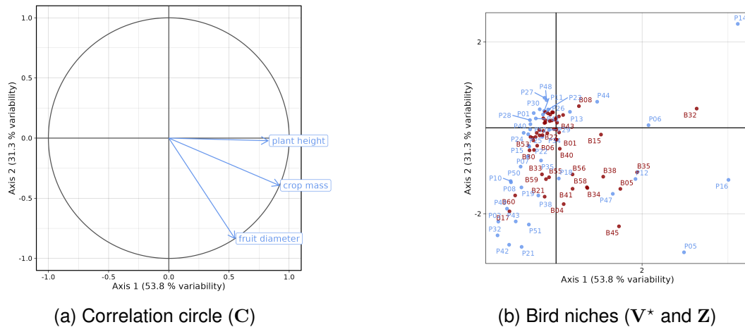
Figure B.1: Correlation circle and bird niches optima from CCA constrained with plant traits. (a) Correlation circle of the CCA constrained with plant traits. (b) Biplot showing bird niches optima ( V^* ) in relation to plant traits ( Z ).
