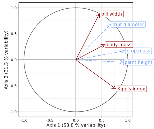
(a) Correlation circle ( C_R and C_Q )
