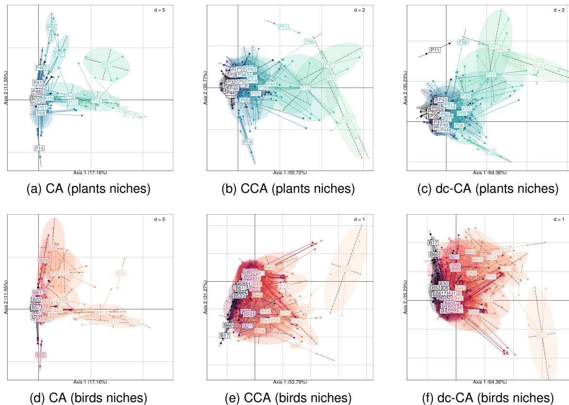
Figure 2.D.2: Comparison of the niches inferred with the different methods. The top row (a-c) shows plant niches and the bottom row (d-f) bird niches. The first column (a and d) shows CA, the second column CCA constrained with bird traits (b) and CCA constrained with plant traits (e) and the last column shows dc-CA (c and f).
