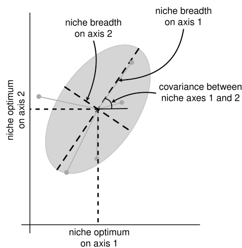
Figure 2.1.1: Visualization of the interaction niche in the multivariate plane. The niche of is depicted by an ellipse whose center represents niche optima and axes represent niche breadths on each axis. The angle of the ellipse represents the covariance between niche axes.
