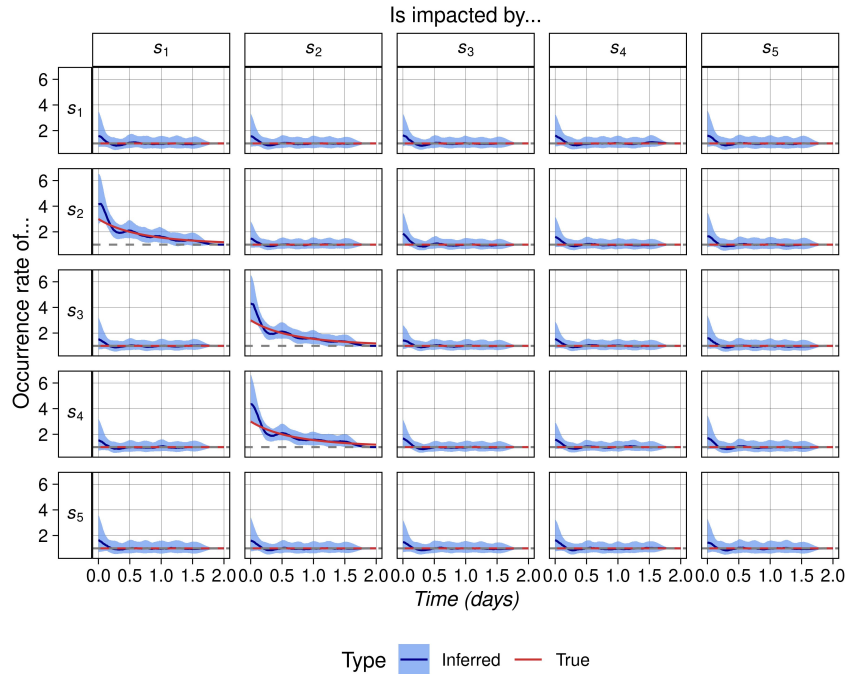
Figure 3.2.2: Performance of the inference with the non-linear multivariate Hawkes process. This graph shows the inferred function (blue, with confidence interval), compared to the true functions used in the simulation model (red) for each pair of species. The line for the inferred interactions functions represents the median of the function for the 100 repetitions and the confidence interval represents the medians of the 95% confidence interval computed by ppstat . The intensity of species in rows is affected by species in columns. The horizontal dashed line represents one. Interaction functions correspond to the f_{j \rightarrow i} from Equation (3.2.2).
