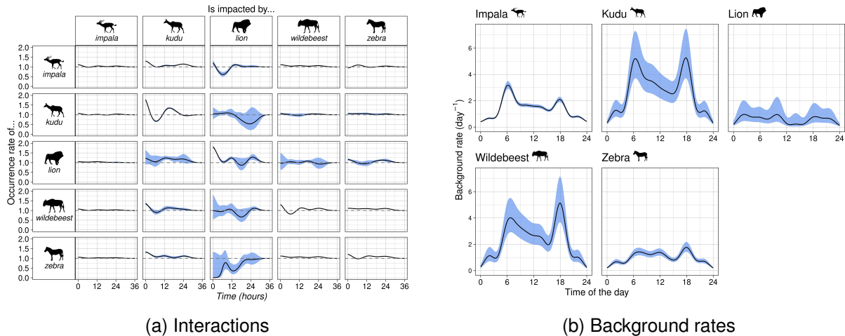
Figure 3.2.4: Model inferred with a time of day covariate. (a) Inferred interaction functions, where the intensity of species in rows is affected by species in columns. The horizontal dashed line represents one. Interaction functions correspond to the f_{j \rightarrow i} from Equation (3.2.2). (b) Inferred background rate. With this model, background rates are a function of the time of the day. They correspond to the \nu_i^l defined in Equation (3.2.2). Silhouette images from PhyloPic by Lukasinioho (wildebeest), Margot Michaud (lion), Robert Hering (kudu), Zimices (zebra) and an unknown author (impala).
