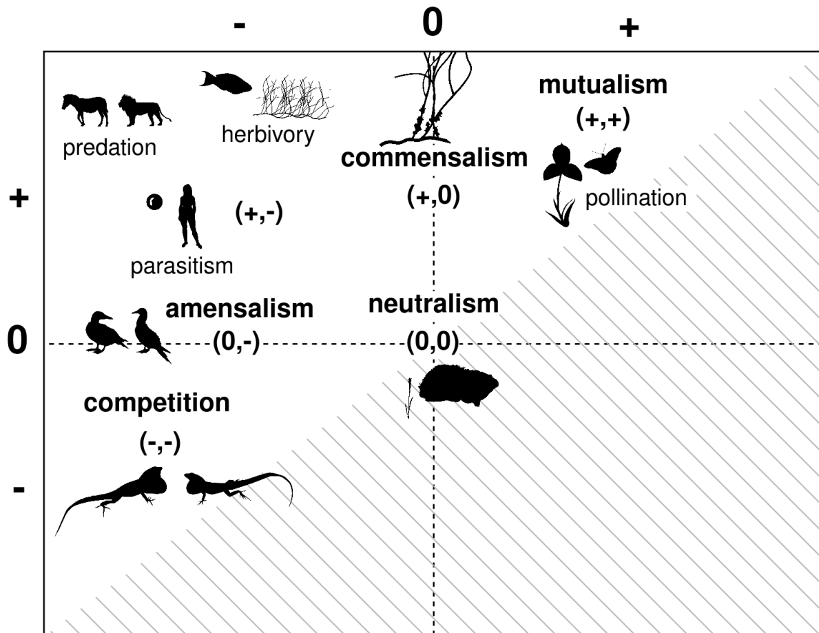
Figure 1.3: Classification of interactions following their effect on the interacting species. Interactions can be classified along a positive-negative effect gradient with two dimensions, one for each species. The x-axis describes the effect of the interaction on the first species, and the y-axis on the second species: positive (+), negative (-) or neutral (0) effect. Each zone corresponds to one interaction type and species silhouettes illustrate examples of interactions described in the main text. The hatched area covers symmetric interactions types to those already represented on the figure. Own figure (CC BY-SA 4.0) inspired by Figure II in Morales-Castilla et al. (2015). Silhouette images from Phylopic by Andy Wilson ( Meneris tulbaghia ), Beth Reinke (Nazca booby), Jon Hill (blue-footed booby), Jonathan Wells ( Plasmodium falciparum ), and NASA ( Homo sapiens sapiens ), others are in the public domain.
