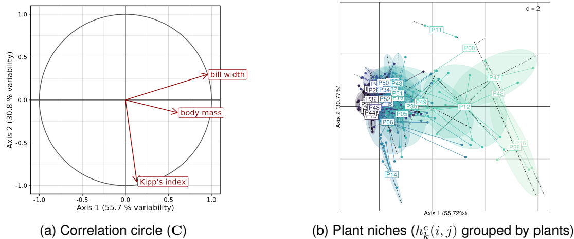
Figure 2.3.3: Correlation circle and plant niches from CCA constrained with bird traits. (a) Correlation circle of the CCA constrained with bird traits. (b) Plant niches. On this figure, each point represents a bird-fruit pairwise interaction. The scores h_k^c(i, j) are computed from \mathbf{Y}^T constrained with \mathbf{Q} . Plant labels are positioned at the optimum of their niche and the ellipse correspond to the bivariate normal distribution of variances and covariances given by reciprocal scaling (with a scaling factor of 1.5, i.e. the ellipse axes lengths are equal to 1.5\sqrt{\lambda_k} on axis k , corresponding to around 67% of the points contained in the ellipse). Species are colored according to the position of their niche optima on the first axis.
