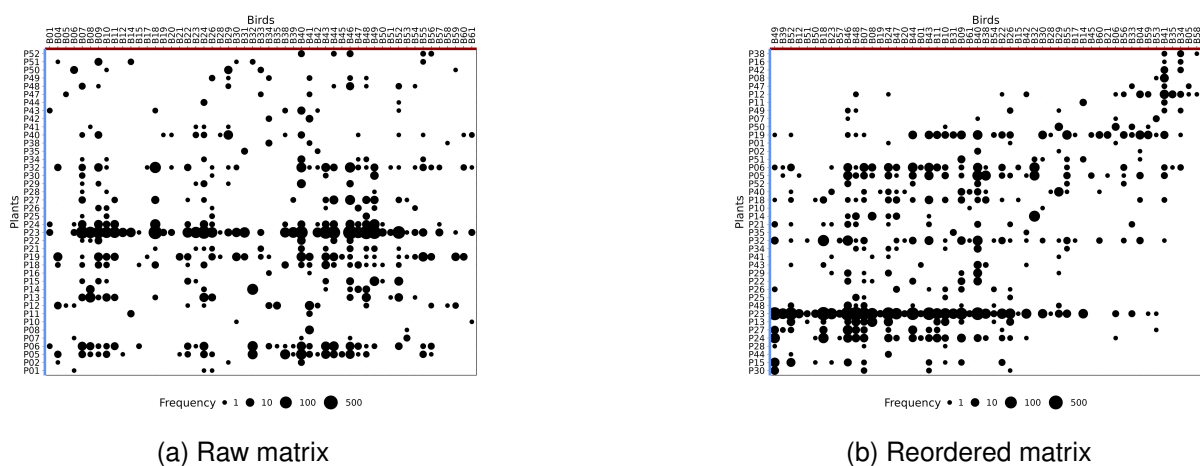
Figure C.1: Interaction matrix reordered using correspondence analysis. This figure shows how an interaction matrix can be reordered using CA. Rows and columns of matrix (a) are ordered alphabetically and for matrix (b) they are ordered following the coordinates of species on the first axis of CA.
