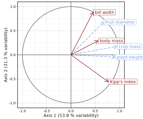
(a) Correlation circle ( C_R and C_Q )
