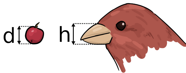
Figure 2.1.1: Illustration of trait matching between a bird and a fruiting plant. Here, trait matching is based on the morphological complementarity between the bird's beak height h and the fruit diameter d (a single trait is involved).
