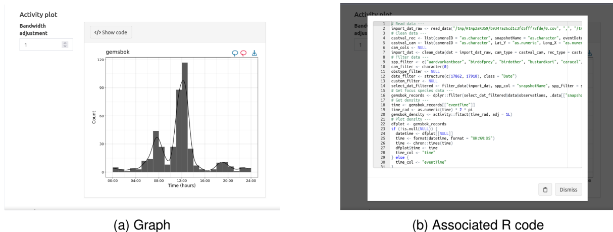
Figure 4.2.3: R code display in the Shiny application. (a) In the interface, the graph is associated with a “Show code” button (top left) allowing to display the associated R code (b).
