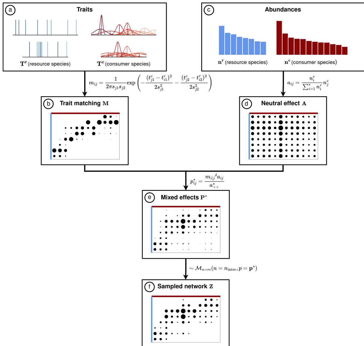
Figure 2.1.2: Model used to simulate interactions between consumer and resource species. (a) Two traits are generated for each species corresponding to their niche optima. For consumers, standard deviations are also associated to traits to generate the niche breadths. (b) Interaction probabilities due to trait matching are computed using a multivariate normal distribution. (c) In parallel, resource and consumers abundances are randomly generated. (d) Interactions counts representing the neutral effect of abundances on interaction probability are computed from abundances. (e) Matching and abundance-driven interactions are combined to get the interactions counts based on both processes. (f) Observed interactions are then sampled from the mixed interaction probabilities. Equations are explained in the main text.
