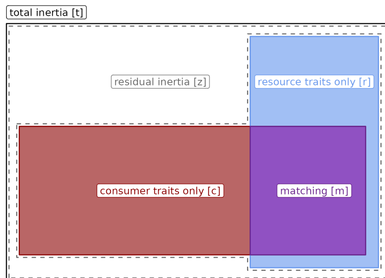
Figure 2.2.1: Variance partitioning of the interaction table. This schematic representation shows how the total inertia of the interaction table [t] can be partitioned into inertia explained by resource and consumer traits in isolation (respectively [r] and [c] ), inertia due to trait matching [m] and residual inertia [z] ( [t] = [r + c + m + z] ). In the general case, when there is some degree of trait matching (i.e. [m] \neq \emptyset ), the total variance explained by resource ( [r + m] ) and consumer traits ( [c + m] ) overlap. Own figure inspired from Figure 1 of Sîrbu et al. (2021).
