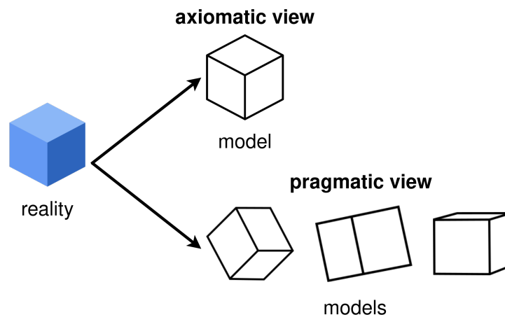
Figure 5.2: Axiomatic and pragmatic view of models. The axiomatic view postulates that the model is an approximation of the reality, while the pragmatic view adds that models also represent a point of view of a given phenomenon occurring in reality. Cube for reality and axiomatic view by kmg design. Other cubes are own designs.
