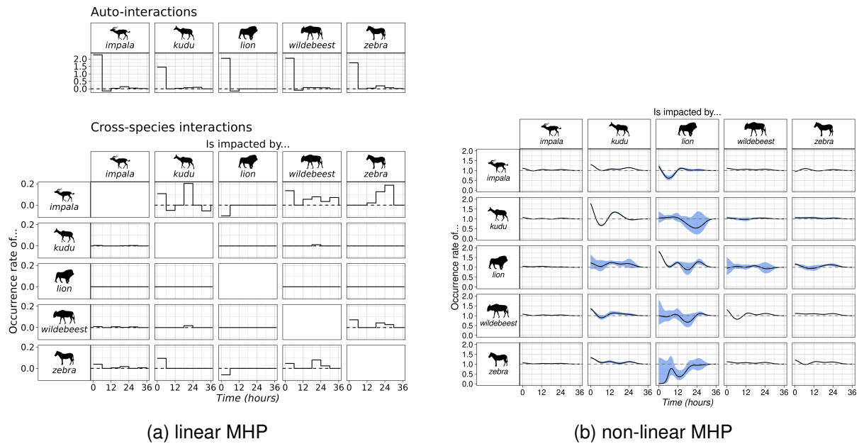
Figure 3.D.1: Comparison of the linear and non-linear MHPs. (a) Linear MHP inferred in chapter 3.1. (b) Non-linear MHP with time of day as a covariate inferred in chapter 3.2. The intensity of species in rows is affected by the species in columns. Silhouette images from PhyloPic by Lukasiniho (wildebeest), Margot Michaud (lion), Robert Hering (kudu), Zimices (zebra) and an unknown author (impala).
