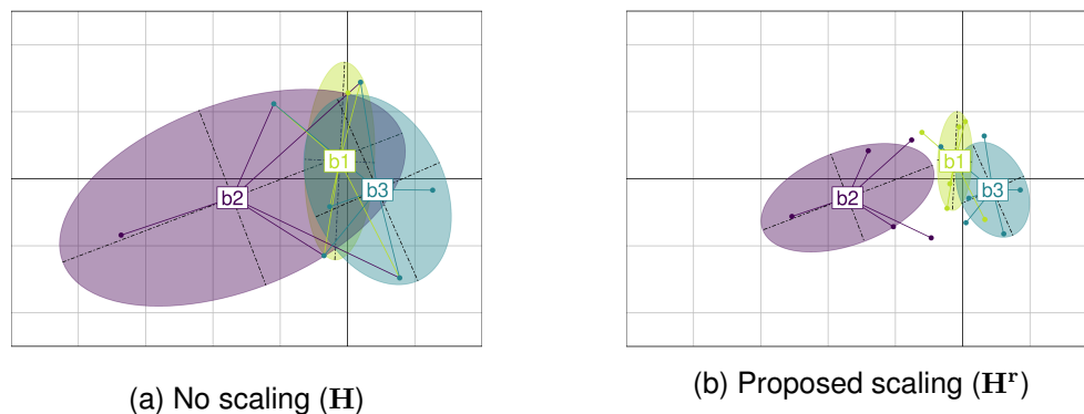
Figure 2.3.2: Graphical effect of the proposed scaling. This figure illustrates how the proposed scaling changes the graphical representation of species niches on a synthetic dataset where 3 consumer species niches are represented.
