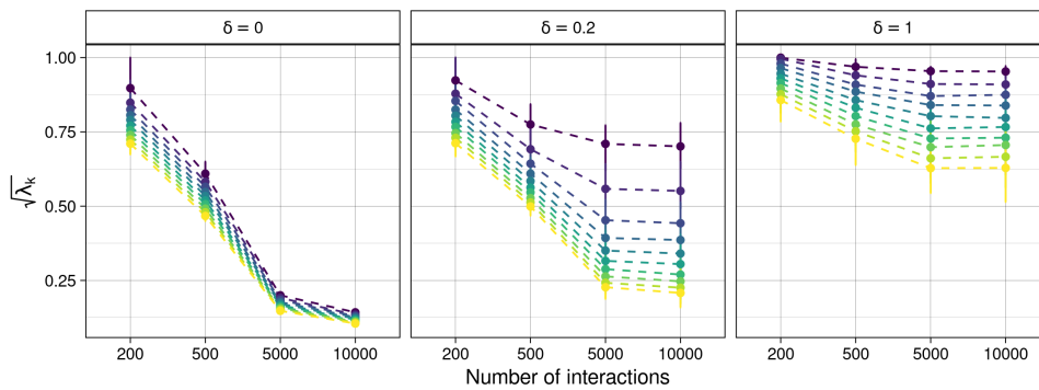
Figure A.2: Eigenvalues evolution with sampling intensity for different values of \delta . This plot shows how eigenvalues evolve with sampling strength, for different values of \delta (panels). Colored points and dotted line represent an eigenvalue, and error bars represent the 2.5 and 97.5-th percentiles on the eigenvalues over 100 repetitions.
