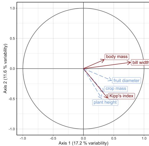
Figure 2.1.6: Correlation circle measured a posteriori between species traits and multivariate axes. Bird traits are shown in solid red lines and plant traits in dashed blue lines. Axis 1 shows a size effect while axis 2 is defined by the matching between plant height and Kipp's index.
