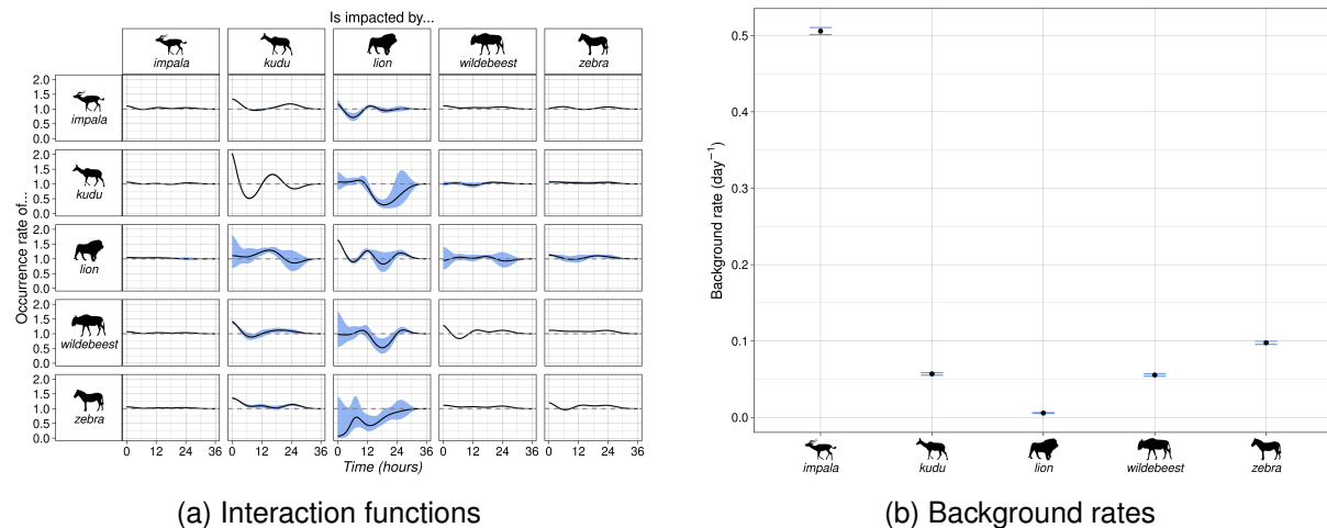
Figure 3.2.3: Model inferred without covariates. (a) Inferred interaction functions, where the intensity of species in rows is affected by species in columns. The horizontal dashed line represents one. Interaction functions correspond to the f_{j \rightarrow i} from Equation (3.2.2). (b) Inferred background rate. With this model, background rates are a constant depending only on the species. They correspond to the \nu_i^l defined in Equation (3.2.2). Silhouette images from PhyloPic by Lukasinio (wildebeest), Margot Michaud (lion), Robert Hering (kudu), Zimices (zebra) and an unknown author (impala).
