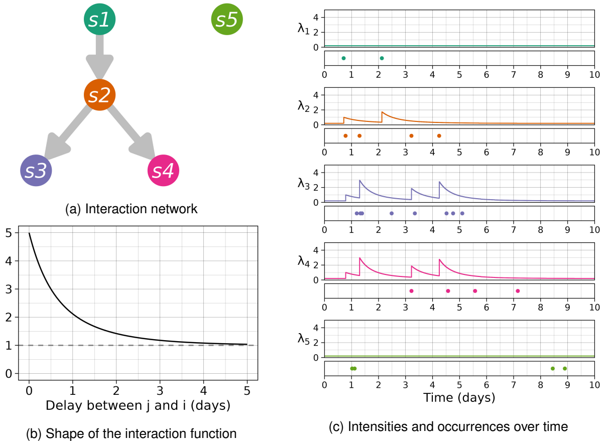
Figure 3.2.1: Example of a realization of a non-linear multivariate Hawkes process. (a) shows the interaction network between five species (each arrow represents an interaction function f_{i \rightarrow j} different from one). (b) shows the shape of the interaction functions f_{i \rightarrow j} , corresponding to arrows in the interaction network (a). The functions f_{i \rightarrow j} are equal to \exp(g_{i \rightarrow j}) , where g_{i \rightarrow j} are defined as a decreasing exponentials. (c) shows a realization of the Hawkes process with the interaction network and the interaction functions shown in (a) and (b). For this simulation, the background rate \nu_i^l was set to 0.2 occurrences day -1 for all species. For each species i , the above panel shows the intensity \lambda_i and the bottom panel shows the species occurrences. Each time an attracting species occurs, the intensity for the attracted species is multiplied by a factor dictated by the interaction function and then decreases following this function's shape.
