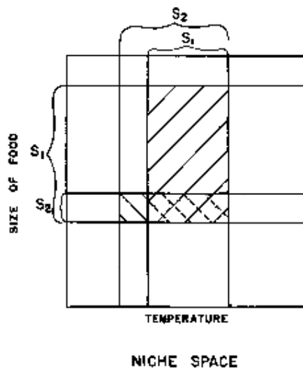
Figure 2.1.2: Original illustration of the Hutchinsonian niche concept. This figure shows two-dimensional niches defined by food size and temperature. The niches of species S_1 and S_2 are depicted as hatched areas and overlap in the middle of the graph. Adapted from Figure 1 in Hutchinson (1957).
