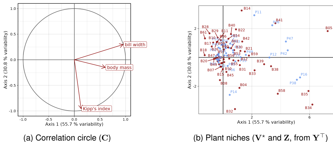
Figure 2.2.2: Correlation circle and plant niches optima from CCA constrained with bird traits. (a) Correlation circle of the CCA constrained with bird traits. (b) Biplot showing plant niches optima ( V^* ) in relation to bird traits ( Z ).
