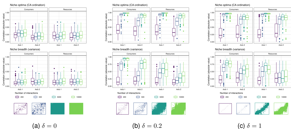
Figure A.1: Effect of the relative importance of matching on the inference of niche parameters. Each subfigure shows the result of the inference for a different value of the trait matching strength \delta . For a more complete description of the figure axes, panels and example matrices, refer to Figure 2.1.3 from the main text.
