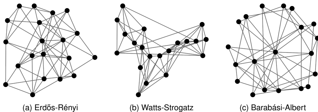
Figure 1.6: Examples of networks generated with different models. (a) Erdős-Rényi network with N = 20 nodes and linkage probability p = 0.3 . (b) Watts-Strogatz network with N = 20 nodes, K = 3 links per node and rewiring probability p = 0.1 . (c) Barabási-Albert network with N = 20 nodes, m_0 = 1 initial nodes and m = 3 links per new node.
