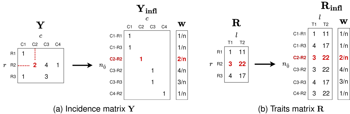
Figure 2.3.1: Correspondence between original and inflated matrices. (a) Correspondence between an incidence matrix \mathbf{Y} and the inflated matrix \mathbf{Y}_{infl} . (b) Correspondence between a traits matrix \mathbf{R} and the inflated matrix \mathbf{R}_{infl} . In this example, \mathbf{Y} represents the interactions between r = 3 resources and c = 4 consumers. \mathbf{R} represents l = 2 traits for resource species. For clarity, zeroes are omitted in the matrices. In the inflated matrices, each row corresponds to an interaction type from the original matrix ( n_{\bar{0}} = 6 interaction types). The weight vector \mathbf{w} contains interaction weights, computed as the weight of the interaction from the original matrix (where n is the grand total of \mathbf{Y} ). The interaction between R2 and C2, and the corresponding traits for R2 are highlighted in all matrices to show their correspondence.
